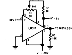
Zero Crossing Detector driving MOS logic
