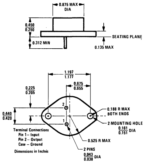
TO-3 Power Package
