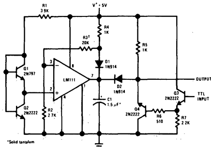
Precision Squarer
