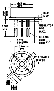
8 Lead Metal Can Package
