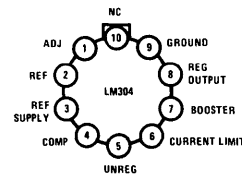
Metal Can
