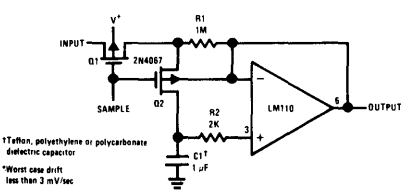
Low Drift Sample and Hold*
