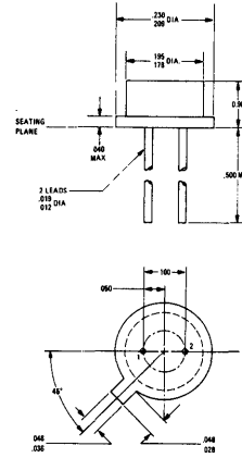
2 Lead Metal Can Package (Modified 3 Lead)
