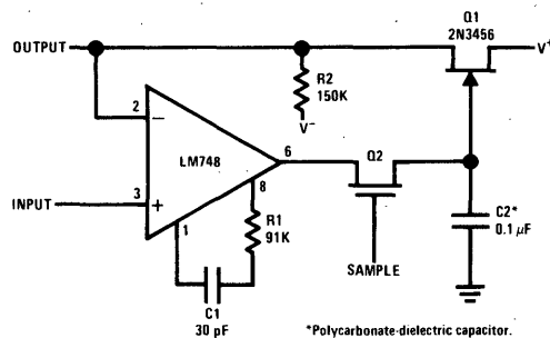
Low Drift Sample and Hold
