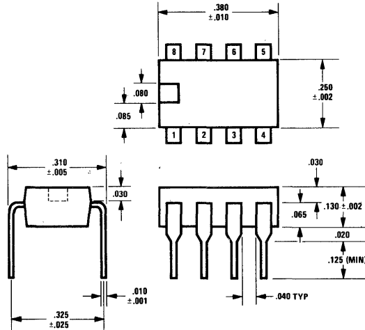
8 Pin Molded Dual-In-Line Package
