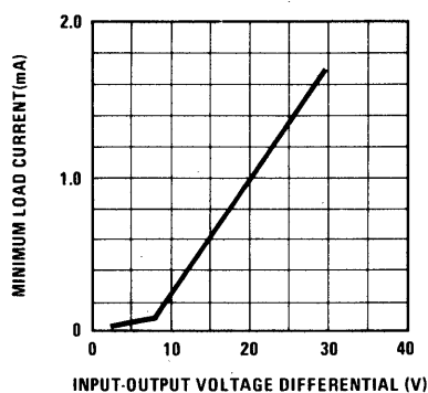
Minimum Load Current vs Input-Output Voltage Differential
