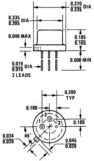
3 Lead Metal Can Package
