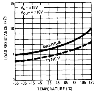
Output Swing
