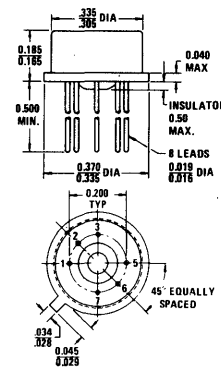
6 Lead Metal Can Package (Modified 8 Lead)
