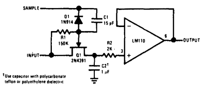
Sample and Hold
