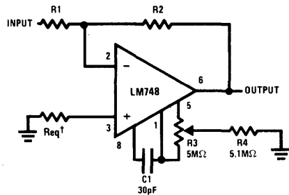
Inverting Amplifier with Balancing Circuit
