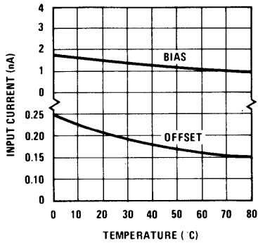
Input Currents
