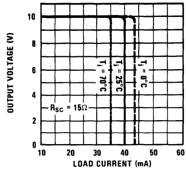
Current Limiting
