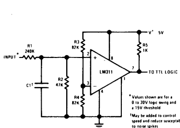
TTL Interface with High Level Logic
