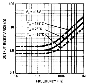
Output Resistance
