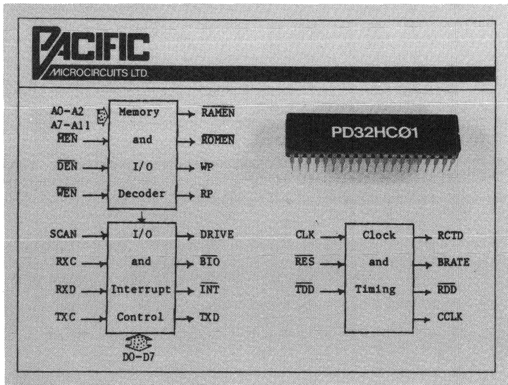
Figure 11-6. Pacific Microcircuits' PD32HC01 Interface IC
