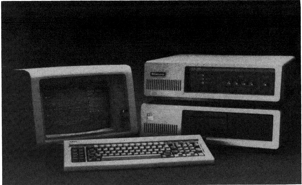
Figure 11-8. SIGnology's SP-20 DSP Development/Measurement System
