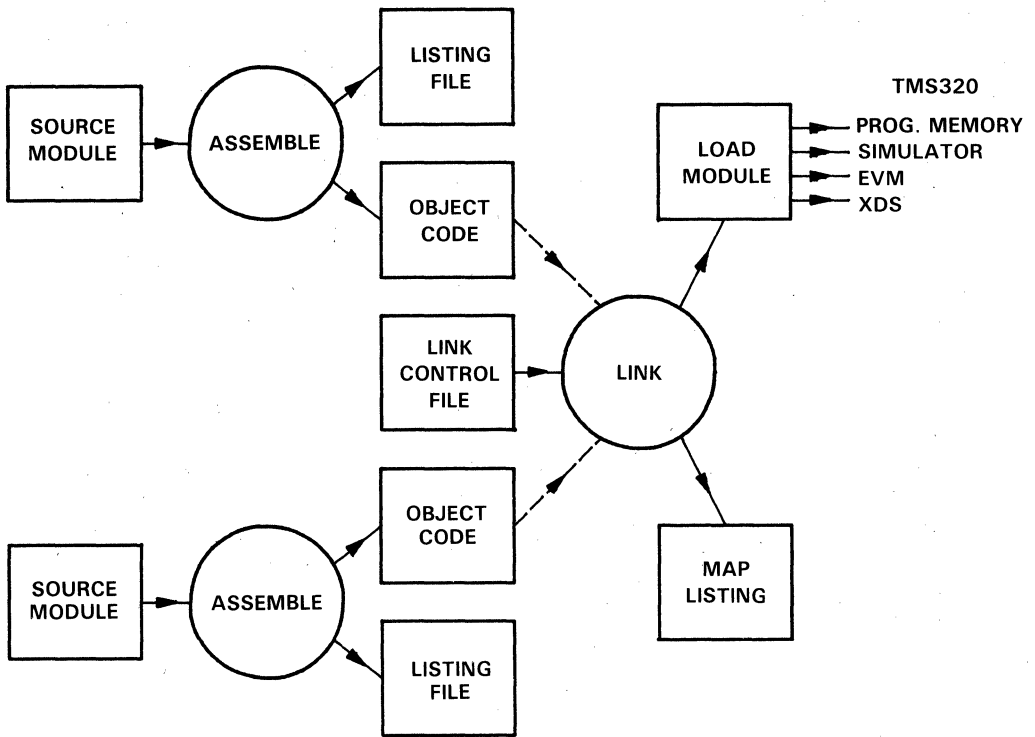
Figure 6-2. Linked Assembly with Multiple-Source Modules
