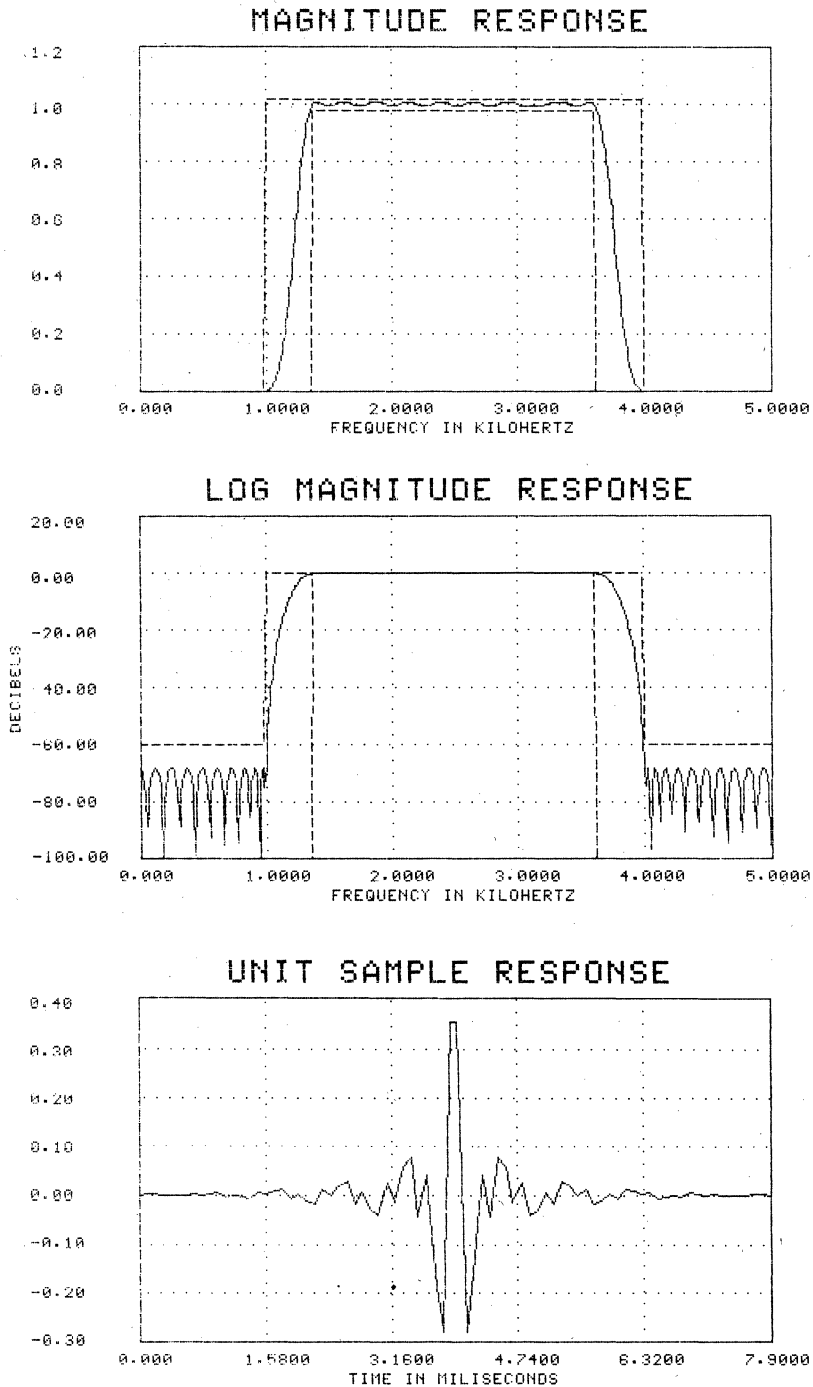
Figure 6-7. DFD Plot Examples
