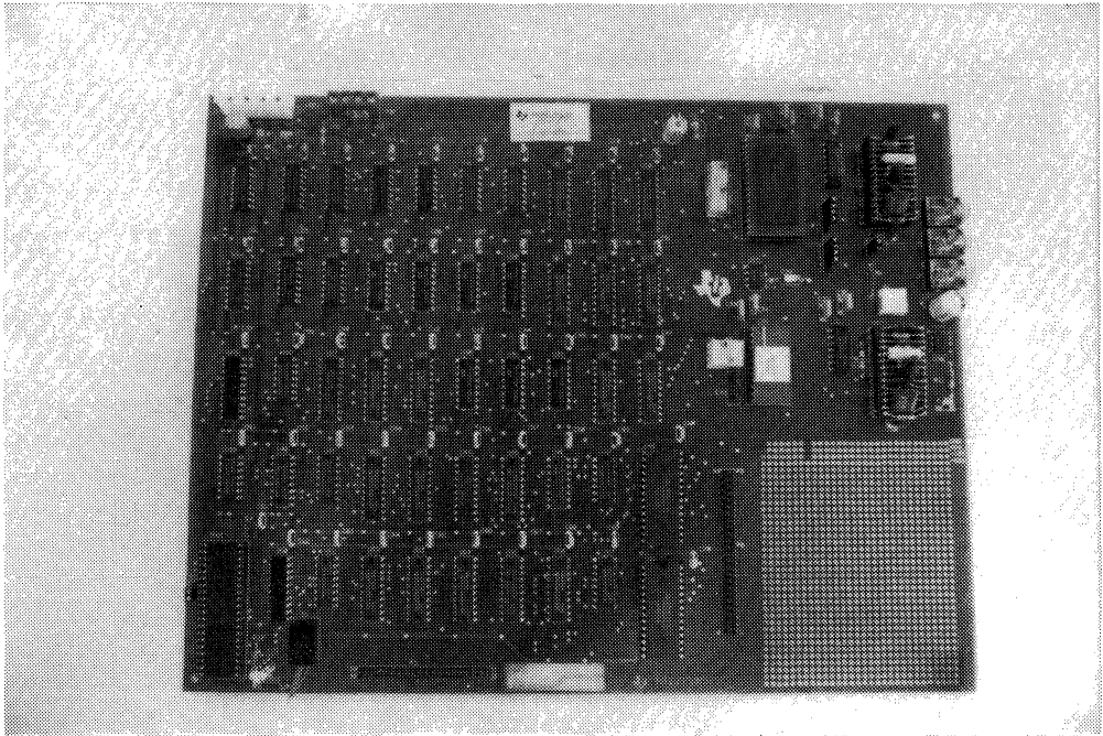
Figure 7-14. TMS320 Analog Interface Board
