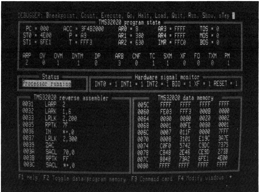
Figure 6-5. SWDS Screen Example
