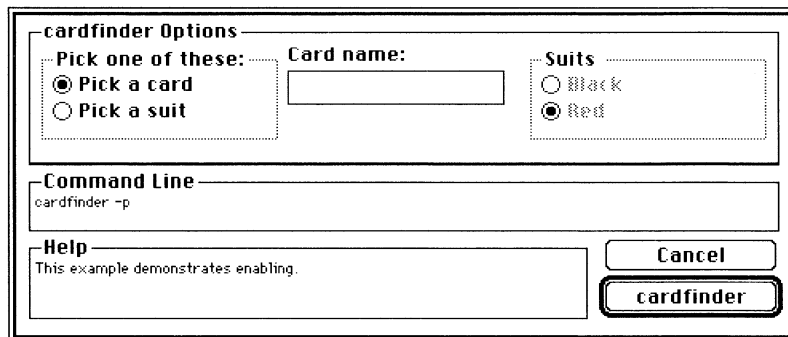
Figure 13-16 Dependencies example: First control selected
