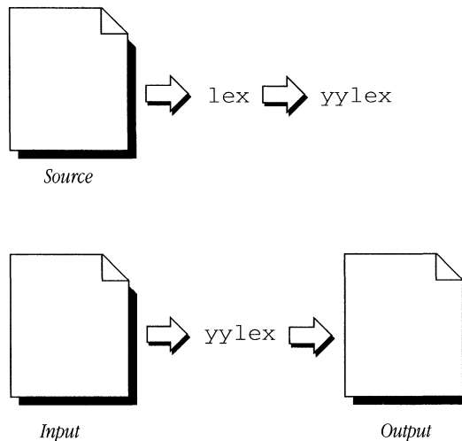
Figure 5-1 Overview of lex
