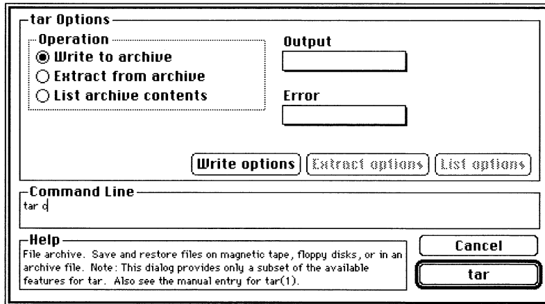
Figure 13-3 Commando dialog box for the UNIX command tar
