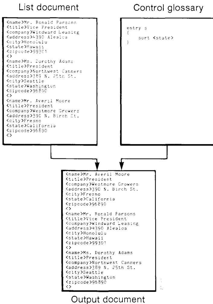
Figure 19 The sort function rearranges records according to the order you specify and by the particular field you choose
