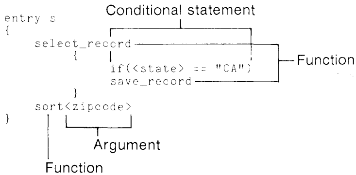
Figure 17 The parts of a control-glossary entry
