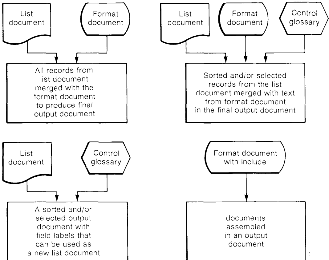
Figure 5. Records Processing Uses from One to Three Documents, Depending on What You Specify
