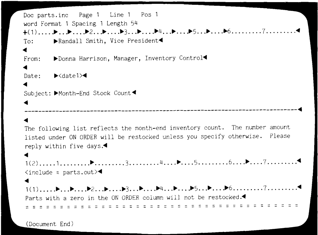
Figure 11 Format document with include statement
