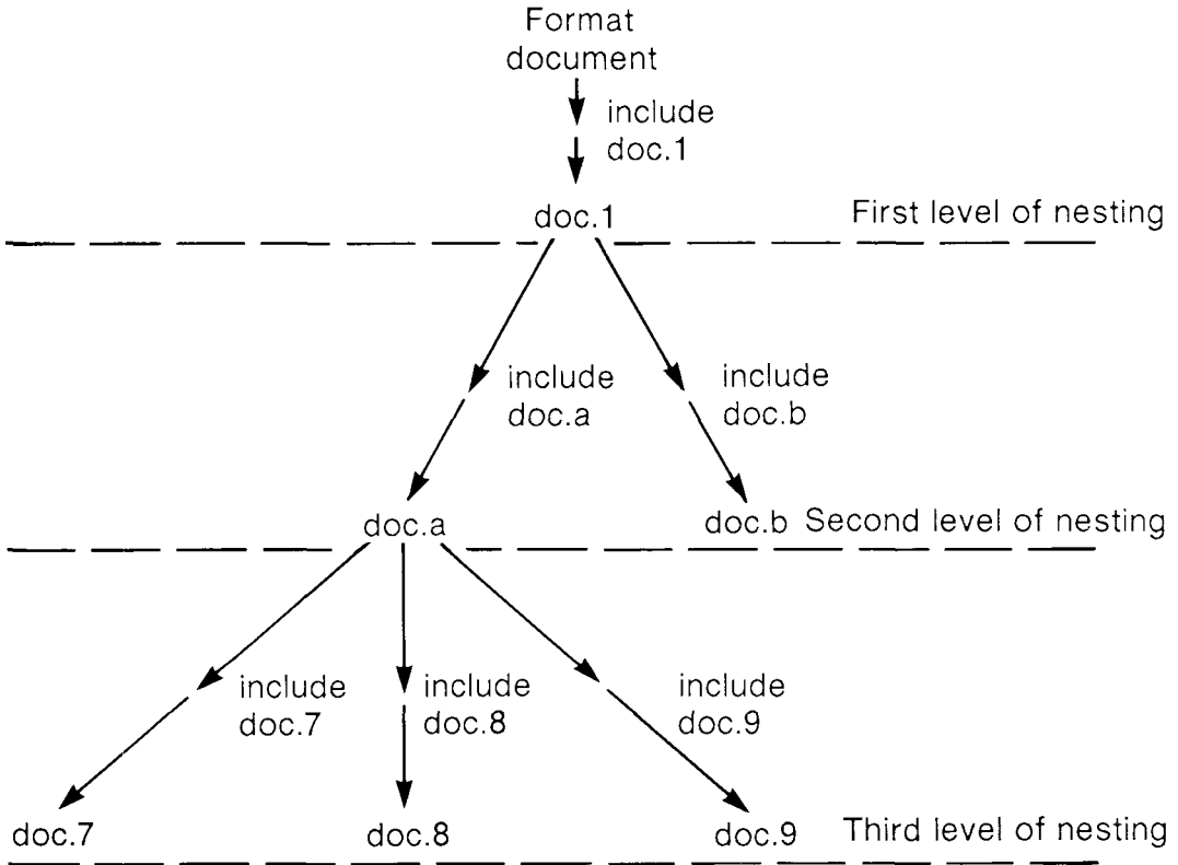
Figure 10 Up to 16 levels of nested include statements are allowed in Records Processing
