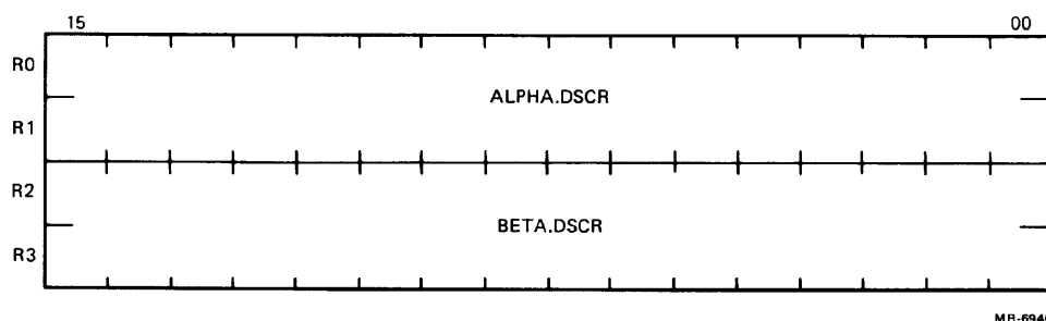
Figure 14-38 Load Two Descriptors Format
