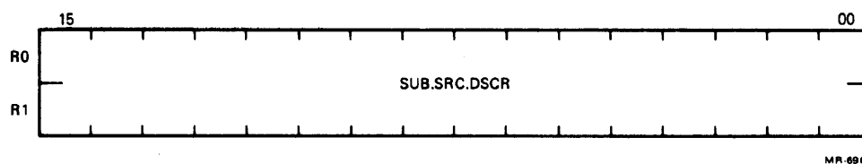
Figure 14-59 Span Character Format (In-Line)
