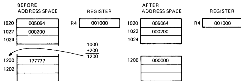
Figure 6-10 Index Mode Example
