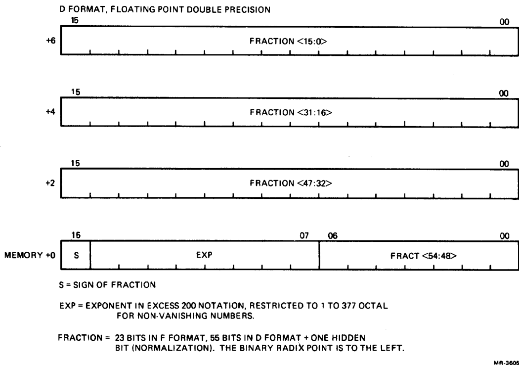
Figure 9-2 Double-Precision Format
