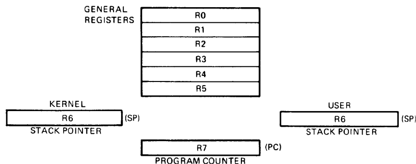
Figure 1-1 General-Purpose Registers
