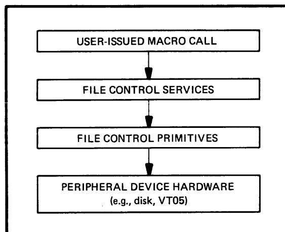
Figure 1-1 File-Access Operation
