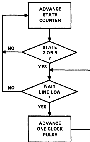
FIGURE 13 – WAIT sequencing steps.
