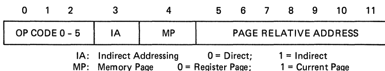
FIGURE 4 – Memory Reference Instruction Format
