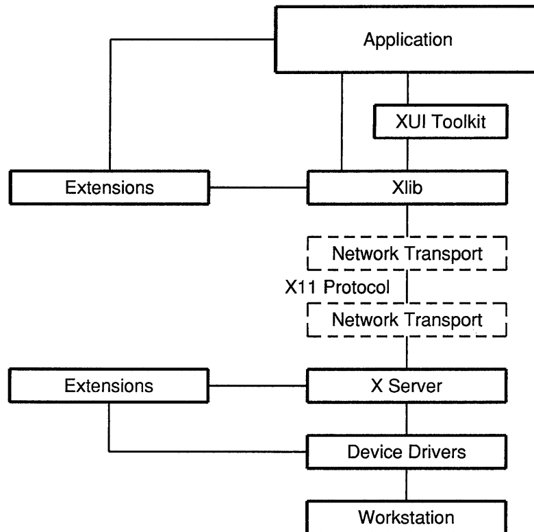
Figure 2-1: XUI Architecture
