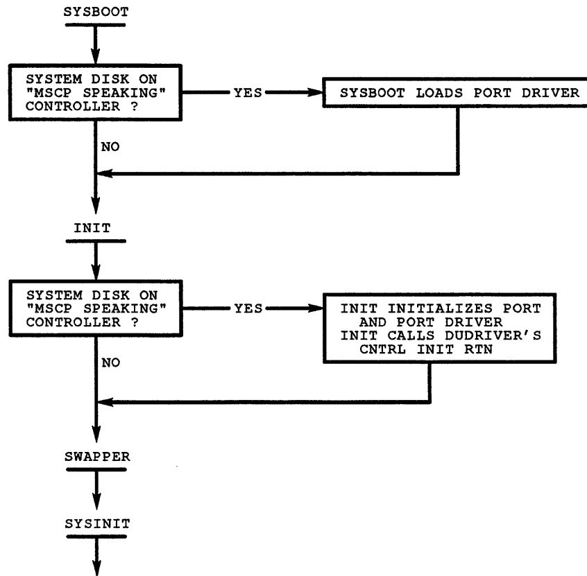
Figure 2-12: Configuration of Devices by Sysboot and Init
