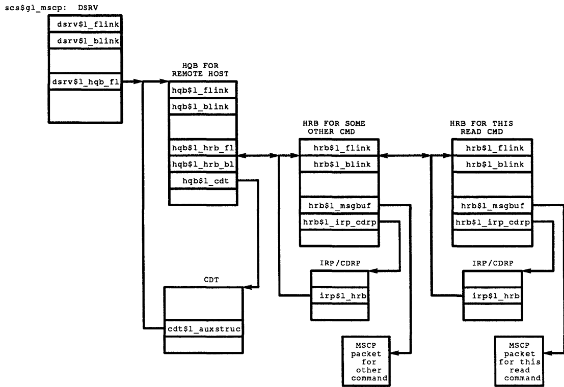
Figure 5–15: Data Structures and Linkage Involved in a Server Receiving a Command
