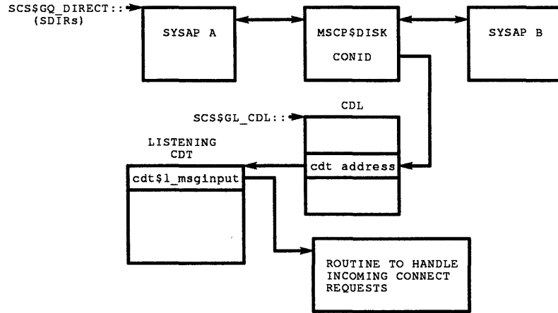
Figure 1-7: Example of a SYSAP in a Listening State
