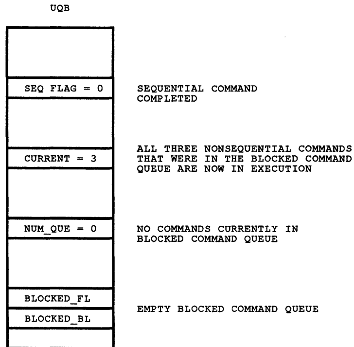
Figure 5-26: Sequential Command Completes and NonSequential Commands Resume
