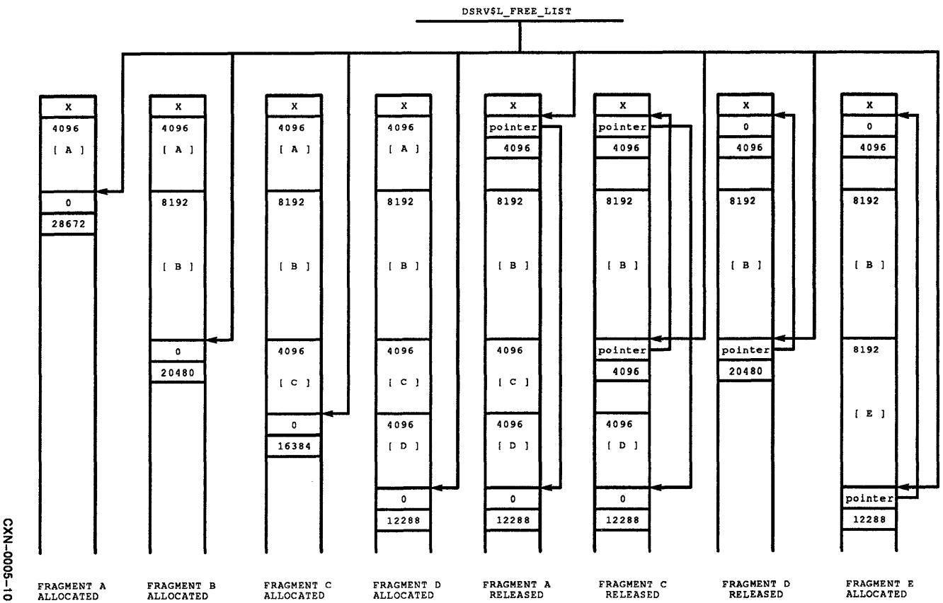
Figure 5-13: Transfer Buffer Allocation and Deallocation
