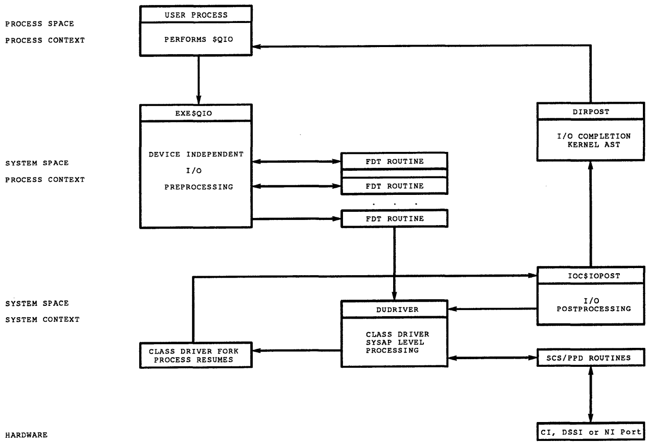
Figure 3-6: QIO Flow Through the Class Driver
