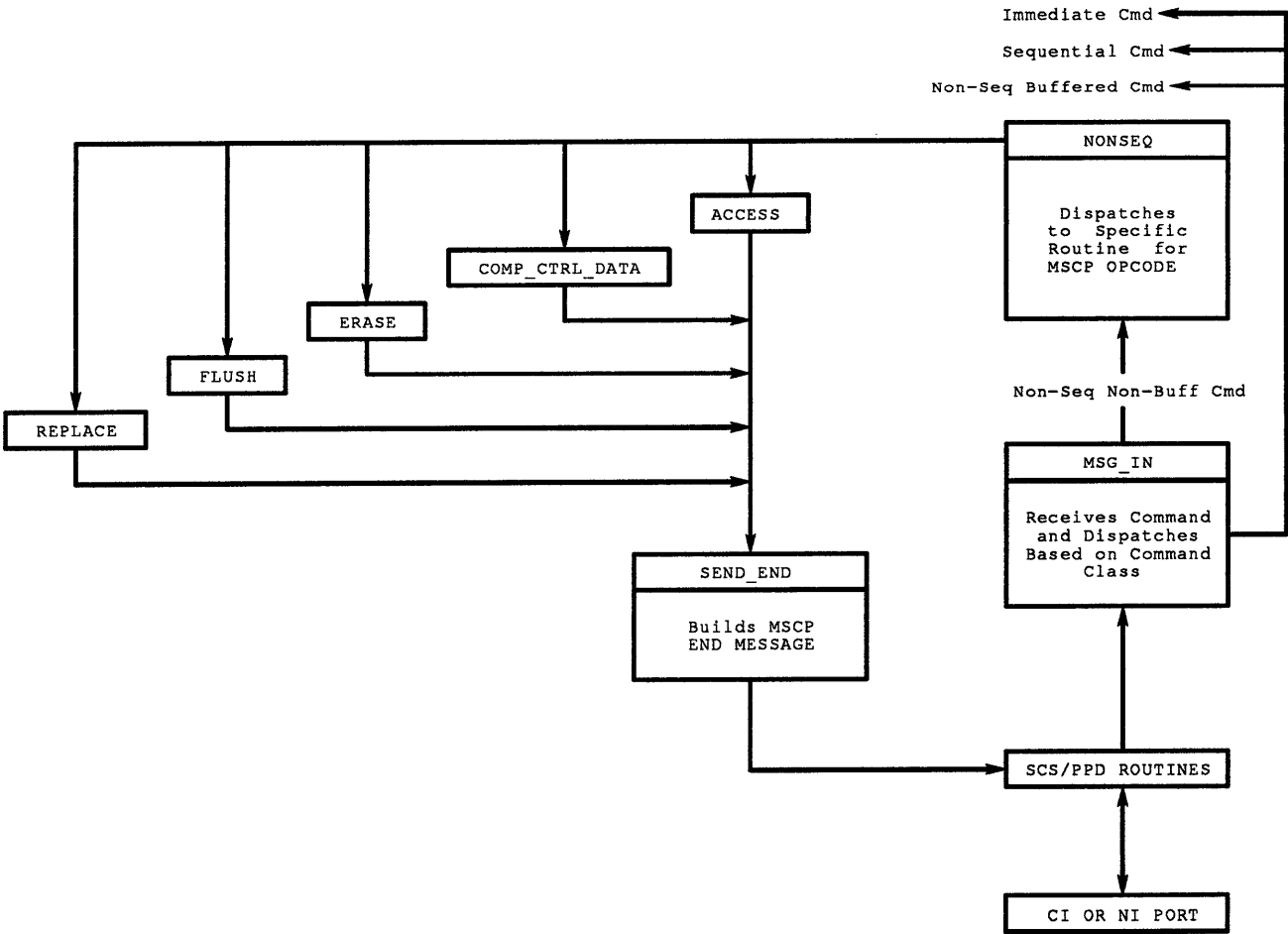
Figure 5-18: NonSequential NonBuffered Command Flow
