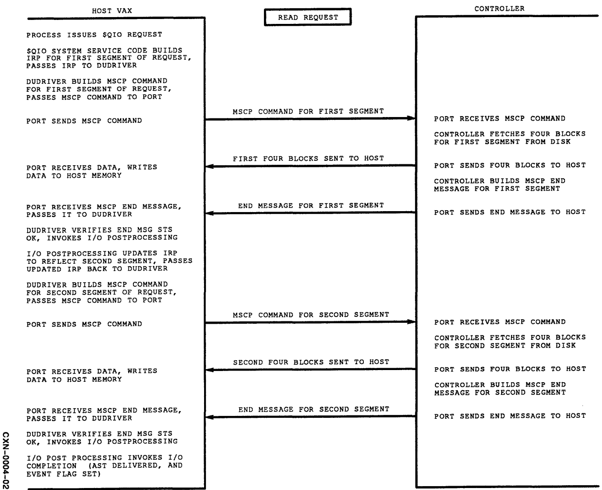
Figure 4-3: MSCP Read Request Message Flow
