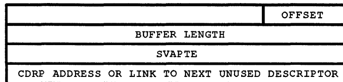
Figure 1-13: Layout of the Buffer Descriptor
