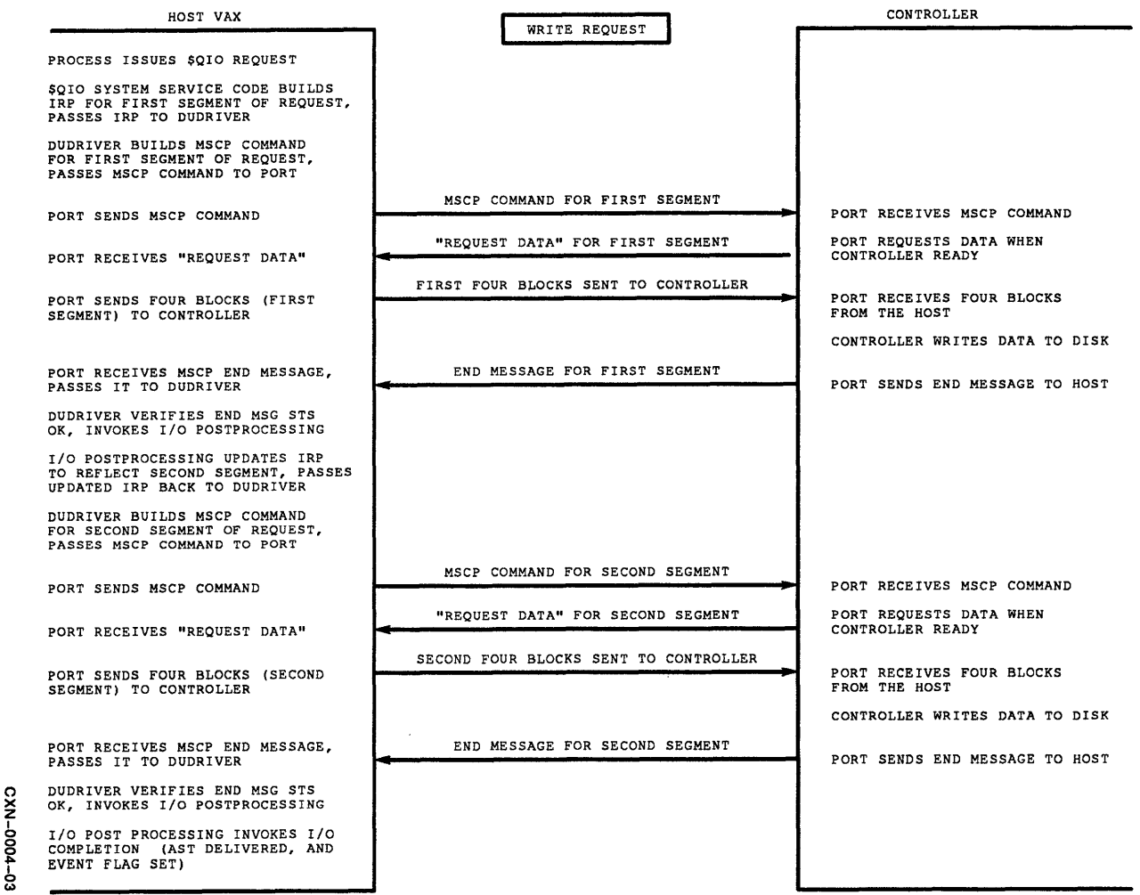
Figure 4-4: MSCP Write Request Message Flow
