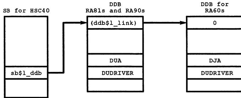
Figure 2-2: DDB Linkage off of the System Block
