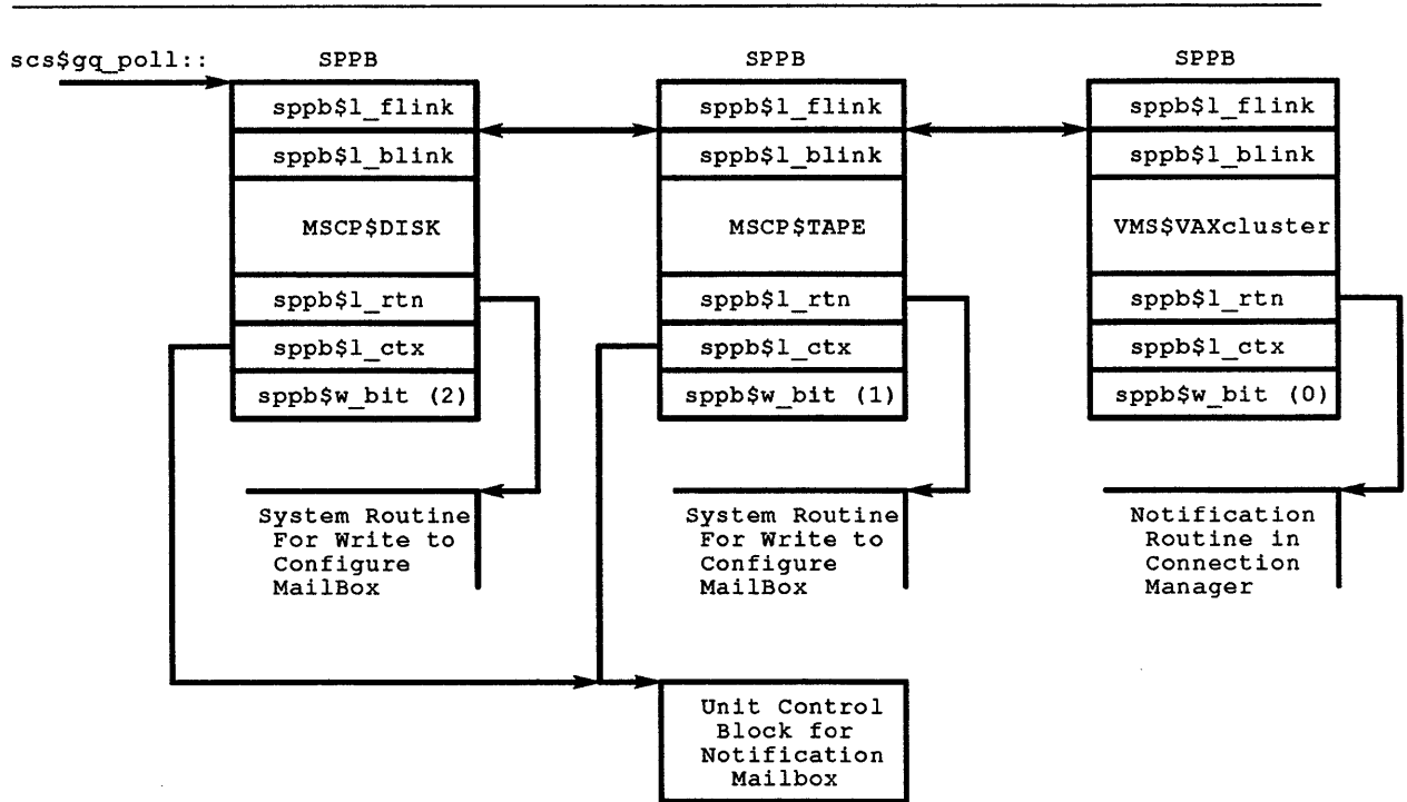
Figure 1-8: SCS Process Poll Block Linkage
