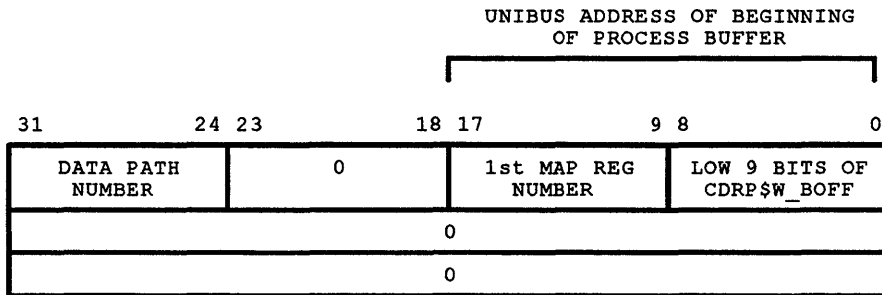
Figure 3-10: Buffer Handle for a UDA buffer
