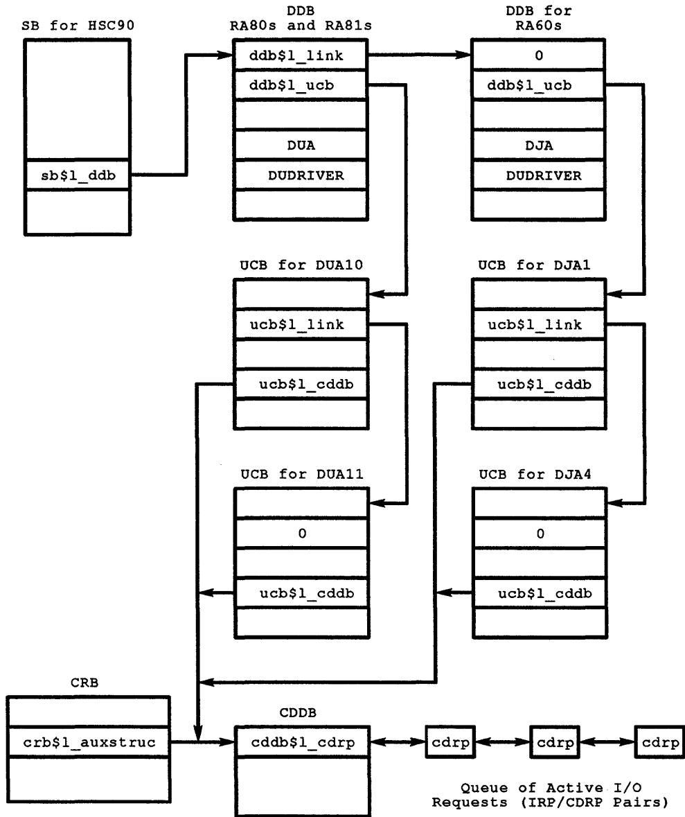
Figure 2-9: CRB Linkage and the General Related Data Structures
