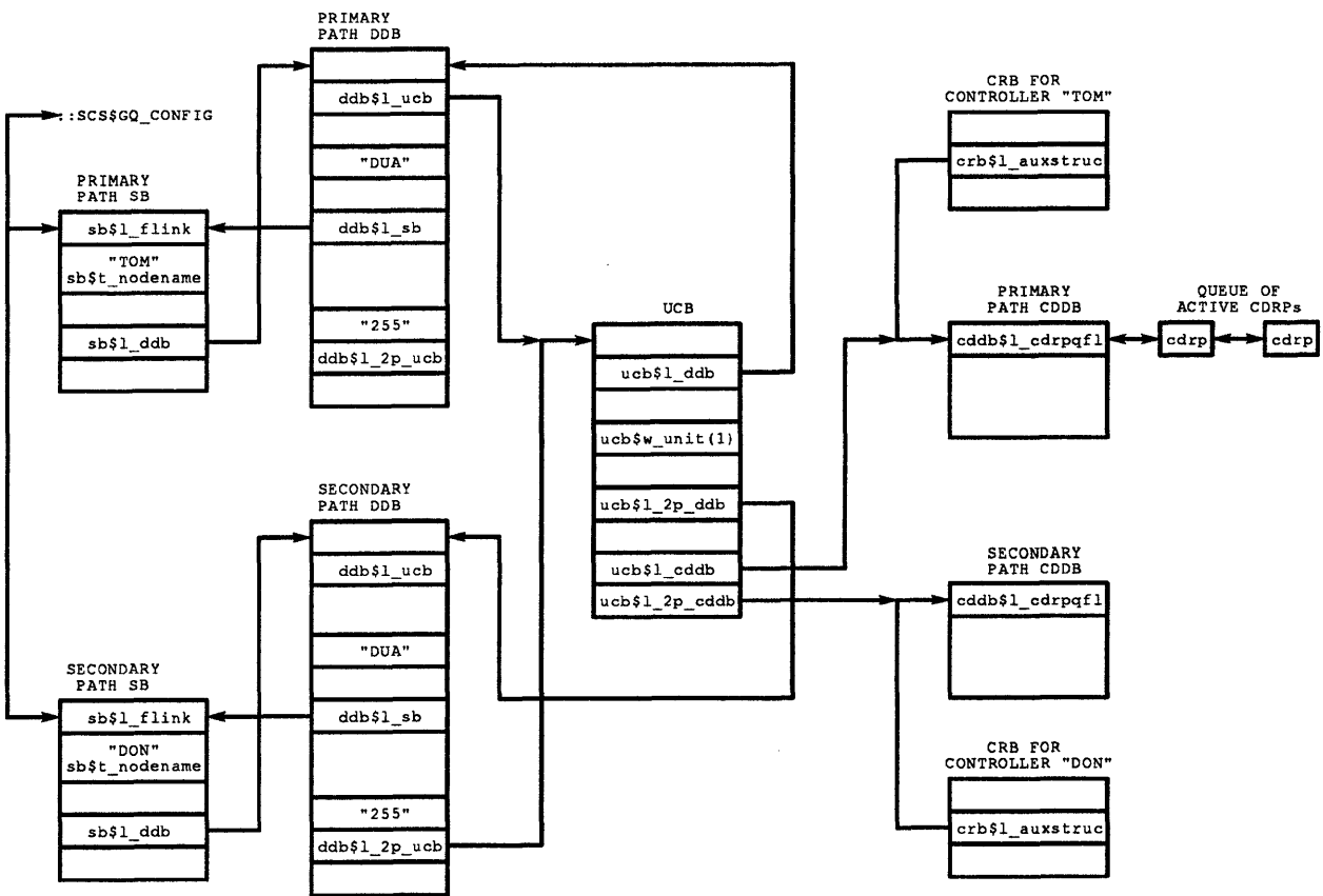
Figure 2-10: Data Structures Supporting Secondary Paths
