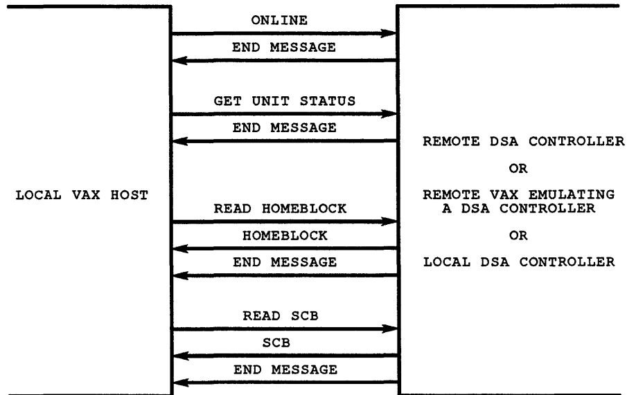
Figure 4-6: Mount Verification Validation Flow
