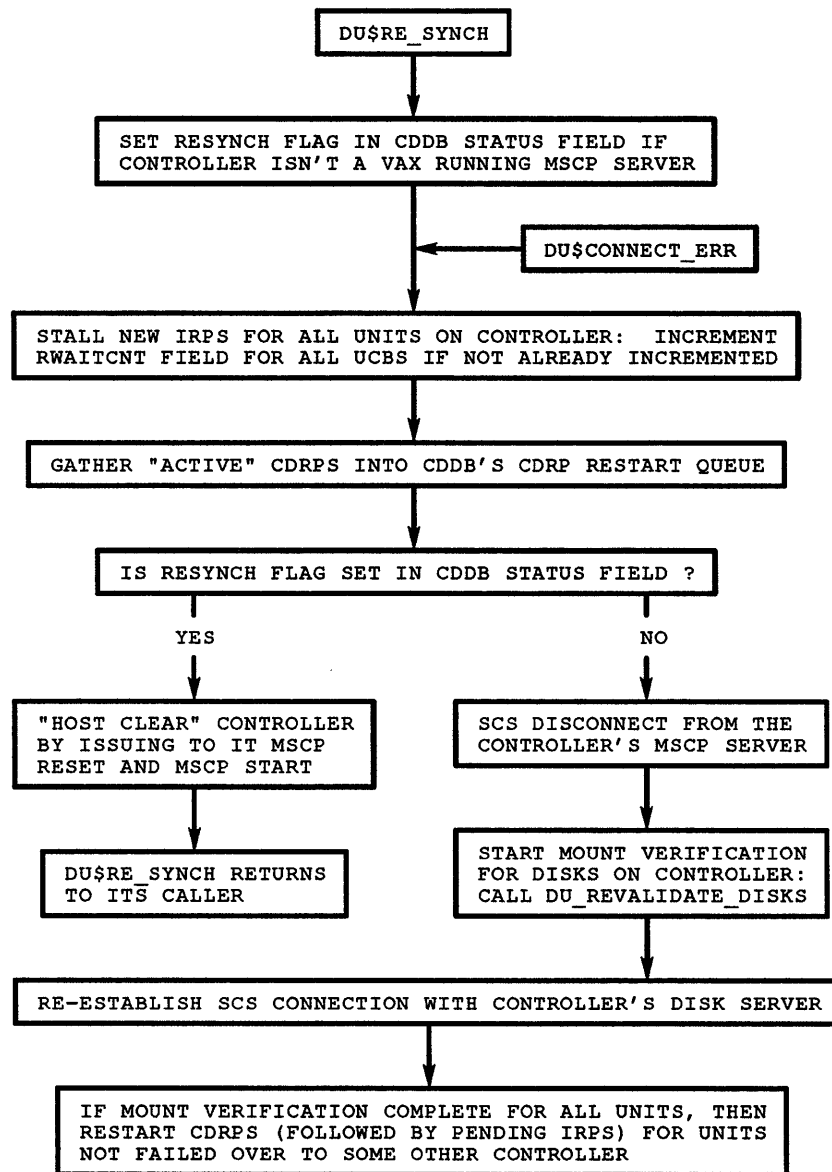
Figure 4-5: DUDRIVER resynchronization flow
