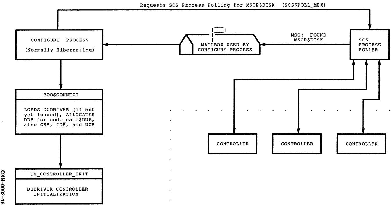
Figure 2-16: Configure Process Polling and Device Configuration
