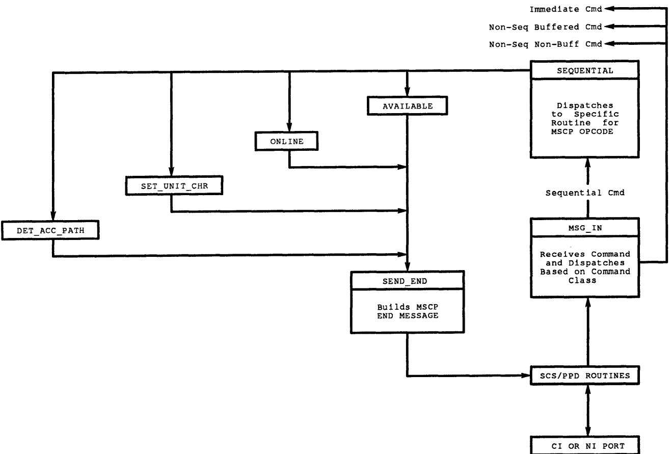
Figure 5-19: General Flow of Sequential Commands
