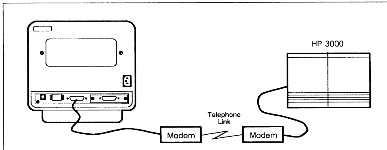
Figure 2-3. Modem Computer Connection for HP 2392A Terminal
