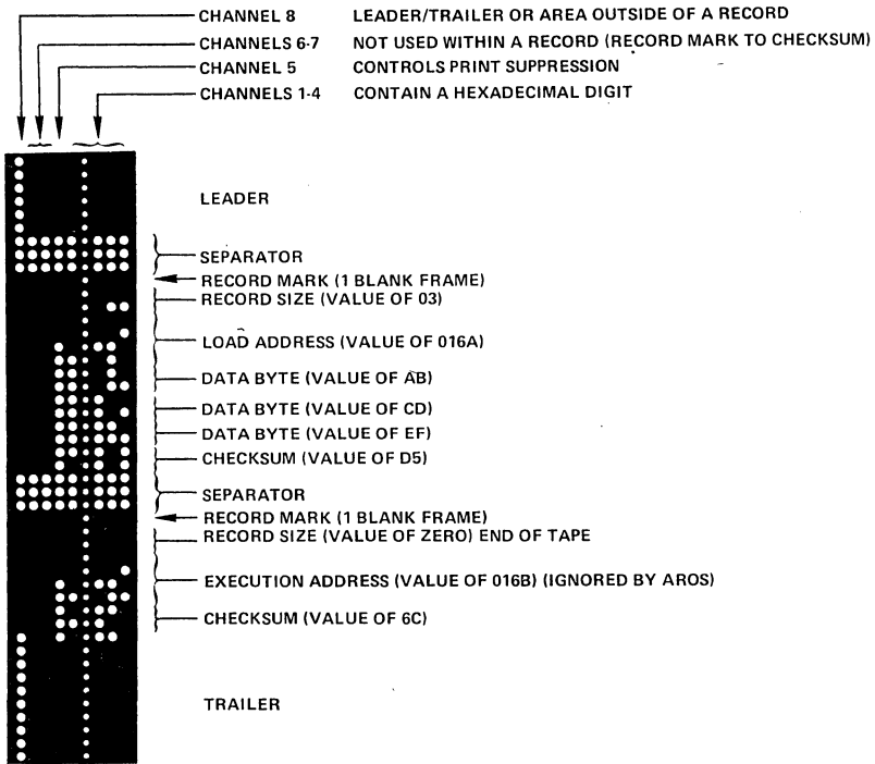
Figure 22. Binary Paper Tape Format
