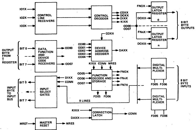
Figure 15. I/O Interface Block Diagram
