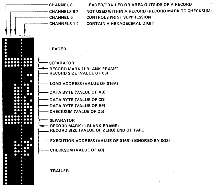
Figure 21. Binary Paper Tape Format
