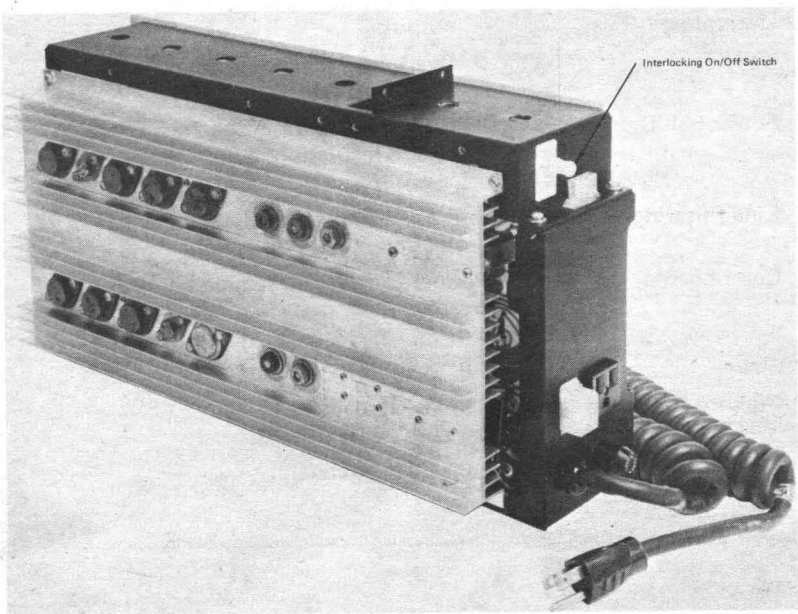
Figure 12. Integral Power Supply of the MICRO 1600
