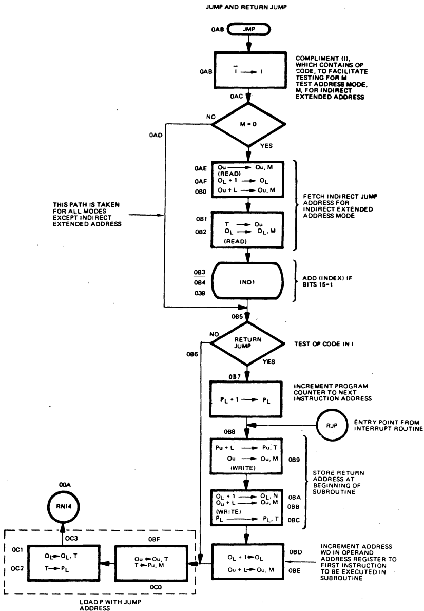
Figure 29. Jump and Return Jump
