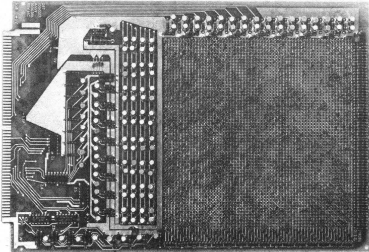
Diode Matrix 256-Word Read-Only Memory.
