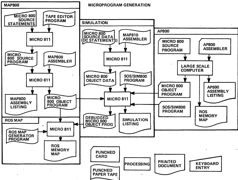
Figure 41. Microprogramming Generation
