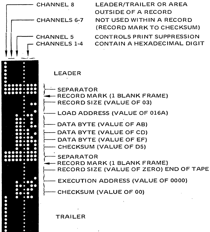
Figure 3. Binary Paper Tape Format
