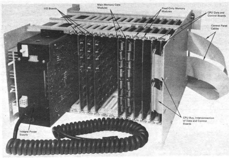
Figure 11. Rear View of Typical MICRO 1600 Card Cage Configuration Showing Integral Power Supply
