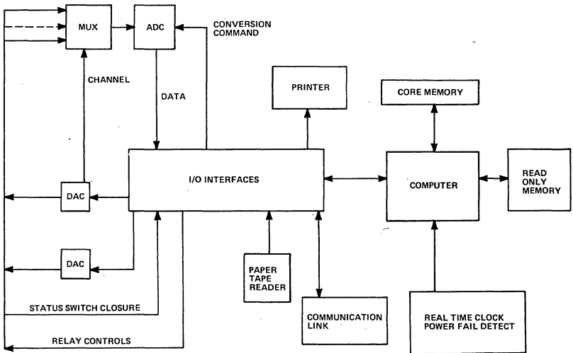
Figure 40. System Example Block Diagram
