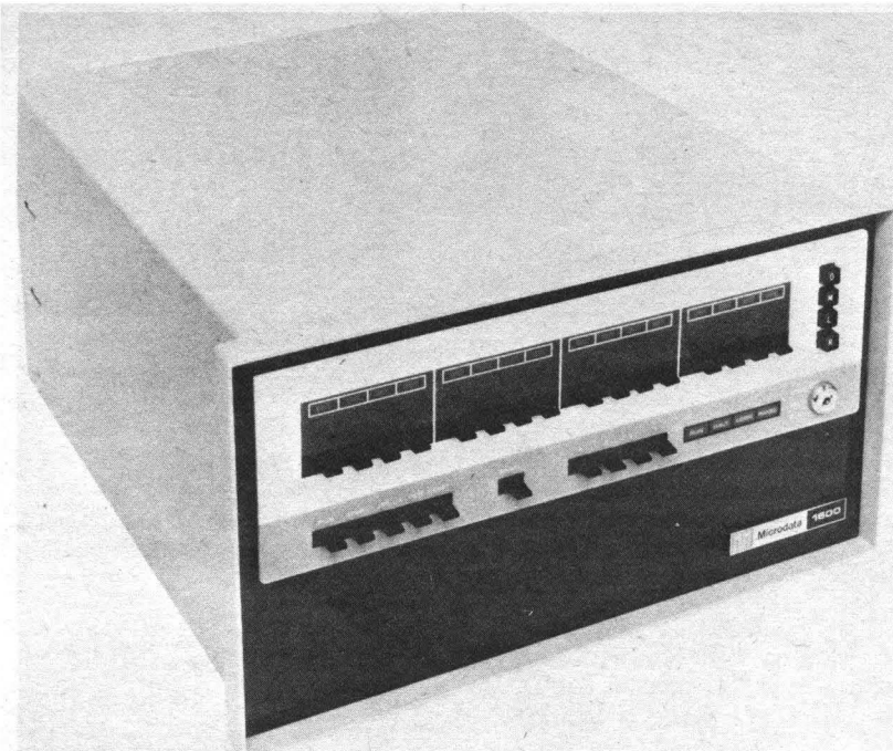
Figure 9. Rack-Mounted Enclosure With Cooling
