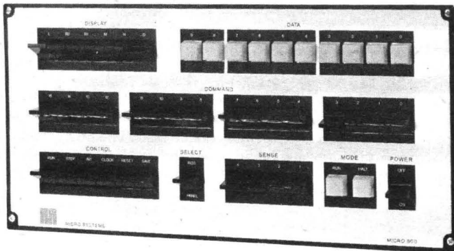
Figure 17. System Console
