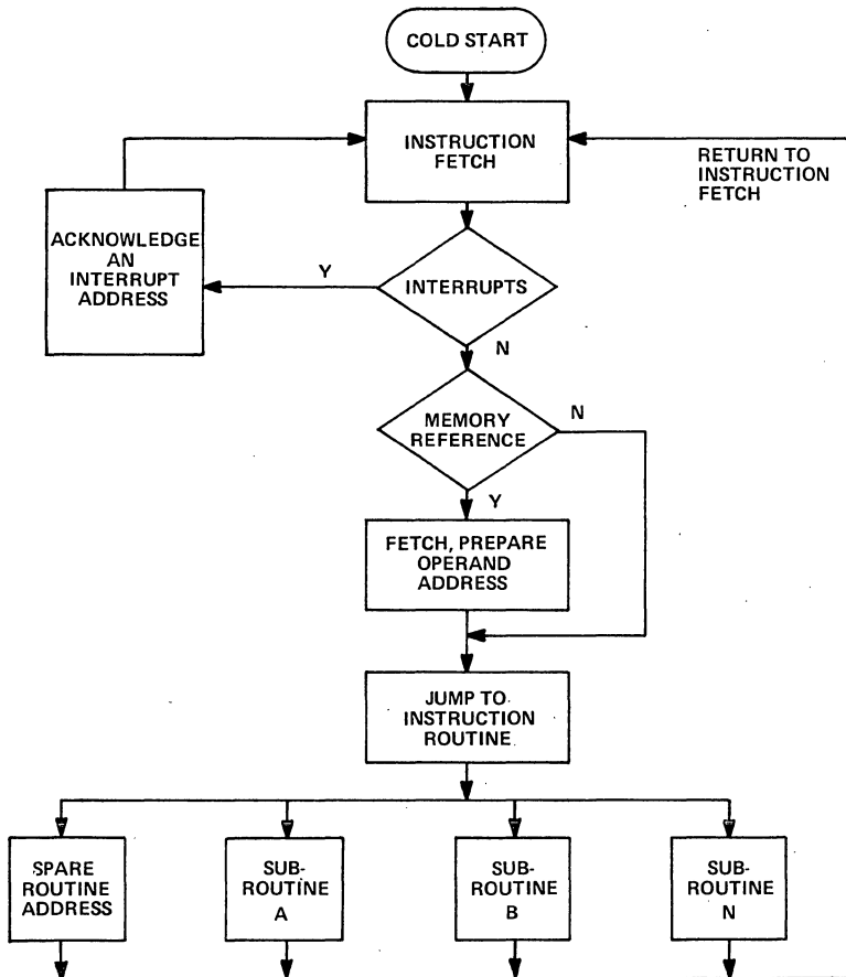
Figure 4. Firmware Function Flow
