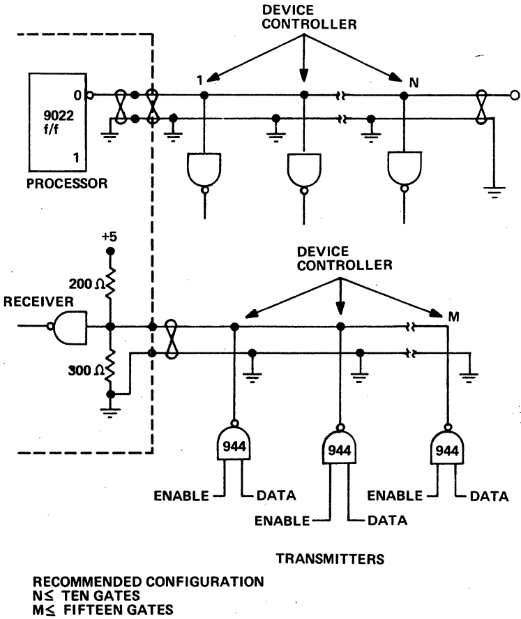
Figure 14. Bus Lines
