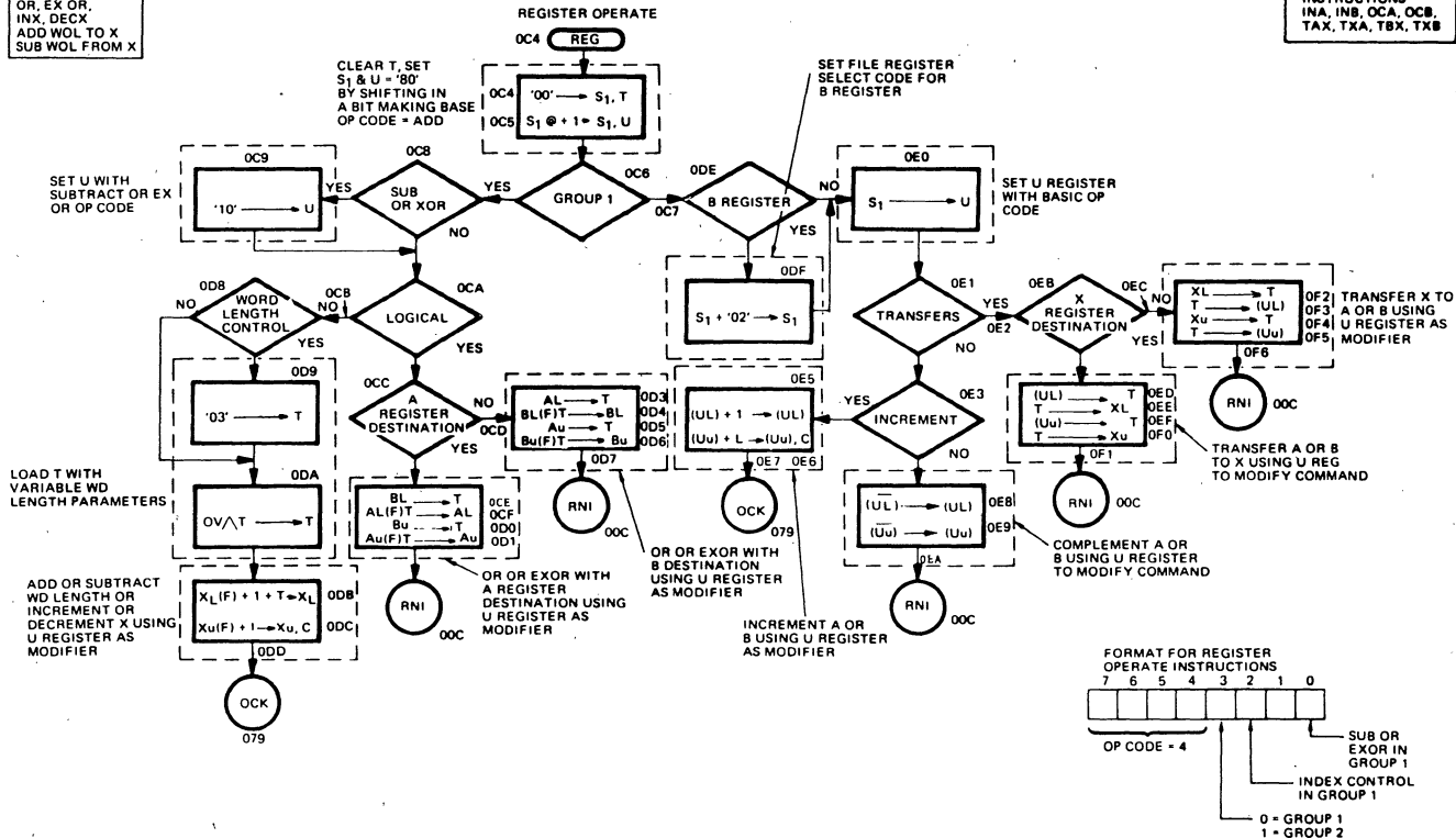
Figure 30. Register Operate
