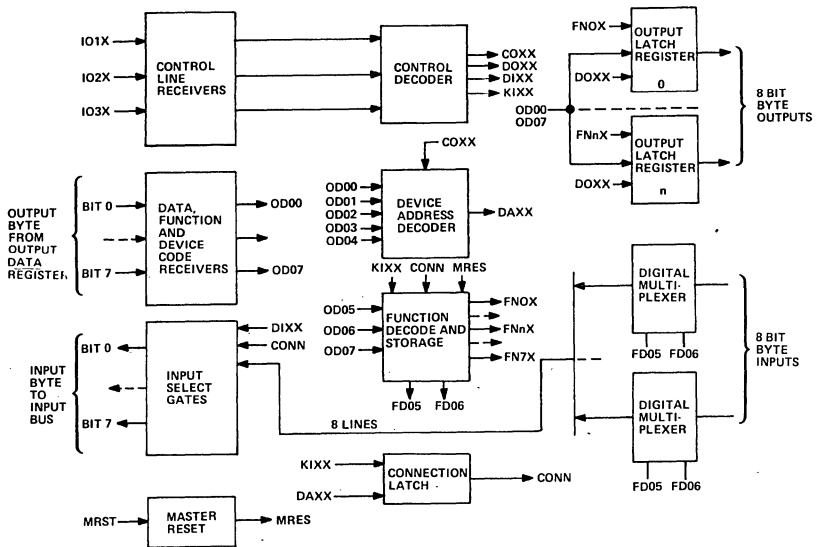
Figure 5. I/O Interface Block Diagram
