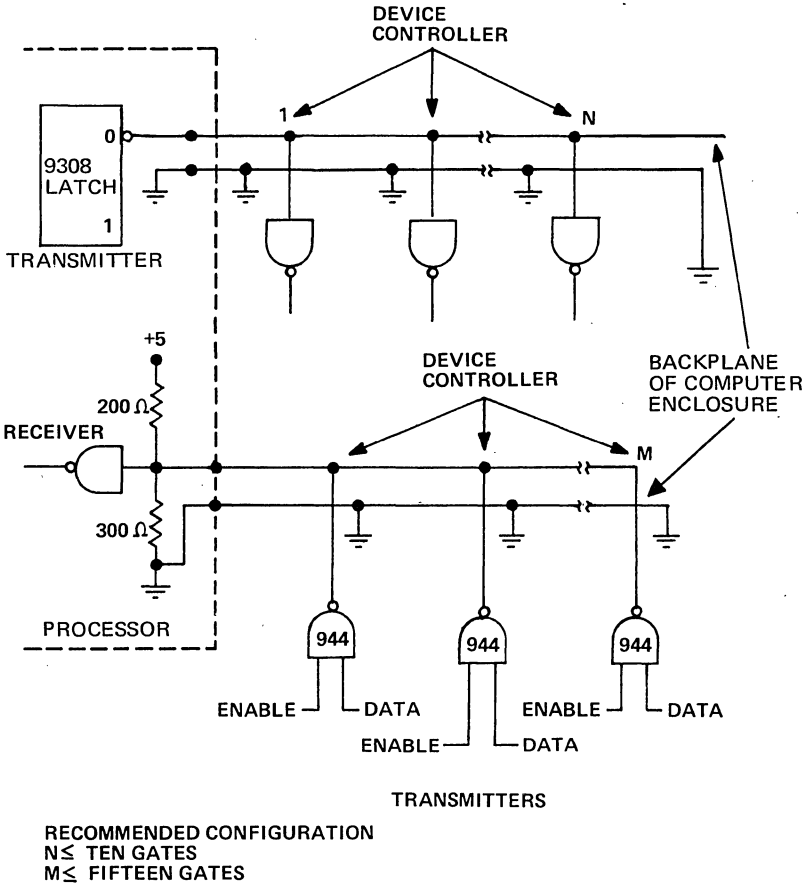
Figure 4. Bus Lines
