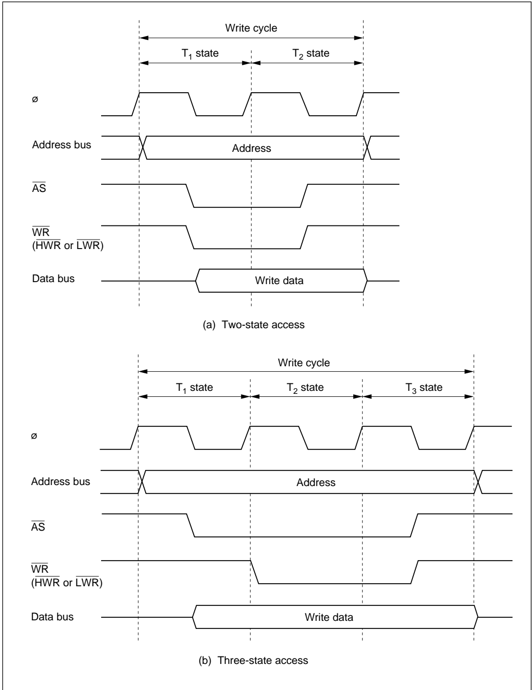
Figure 4-6 External Device Access Timing (2) Write Timing
