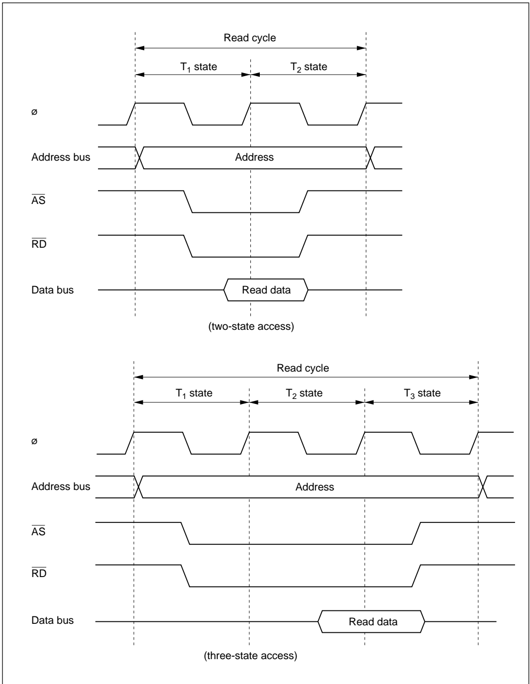
Figure 4-5 External Device Access Timing (1) Read Timing
