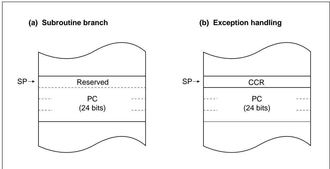
Figure 1-5 Stack Structure (advanced mode)
