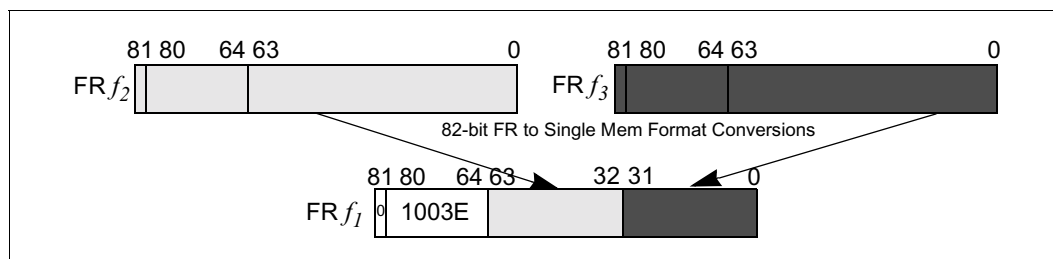
Figure 2-14. Floating-point Pack
