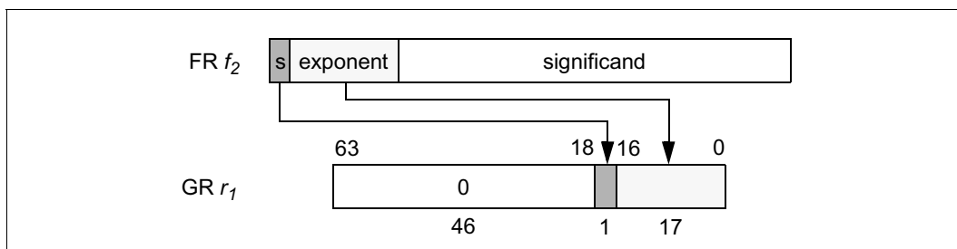
Figure 2-23. Function of getf.exp
