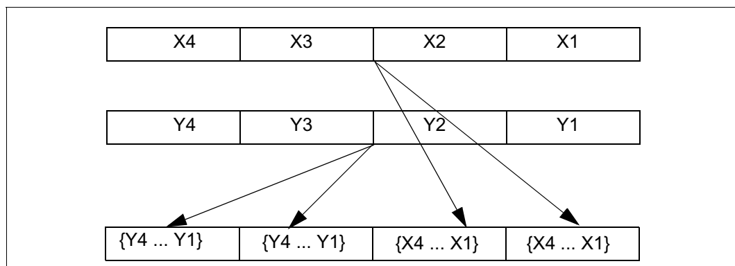
Figure 3-5. Packed Shuffle Operation
