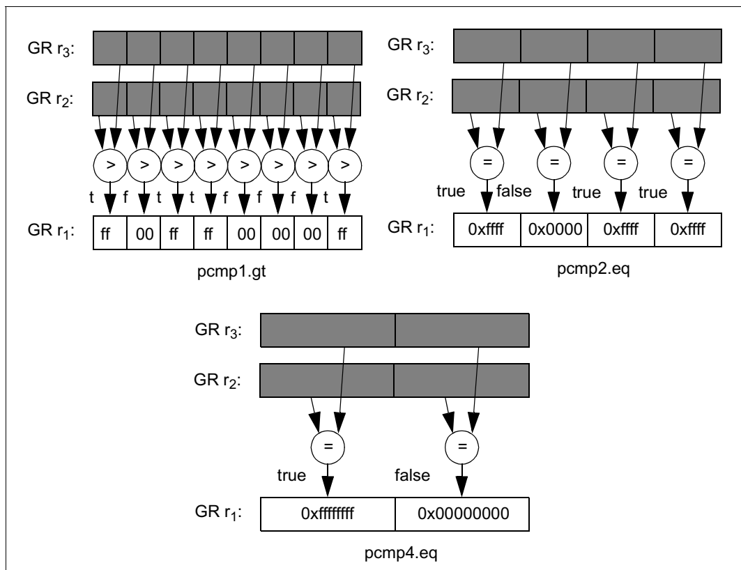
Figure 2-33. Parallel Compare Example
