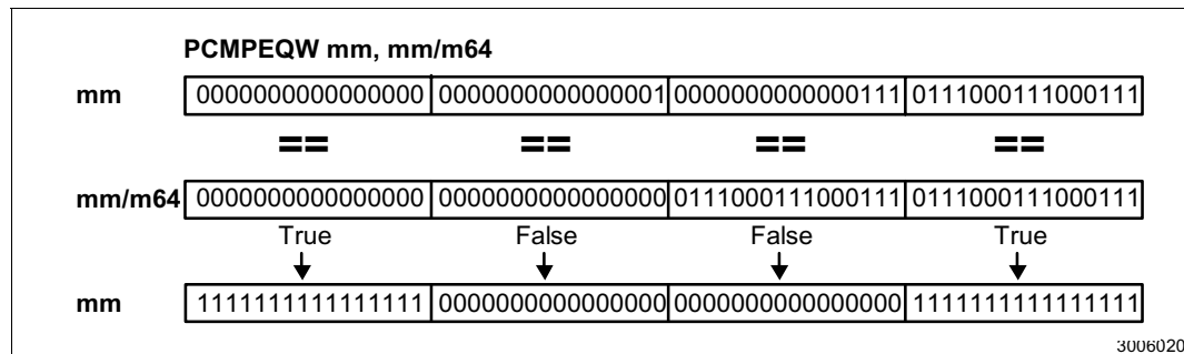
Figure 2-10. Operation of the PCMPEQW Instruction
