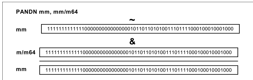
Figure 2-9. Operation of the PANDN Instruction
