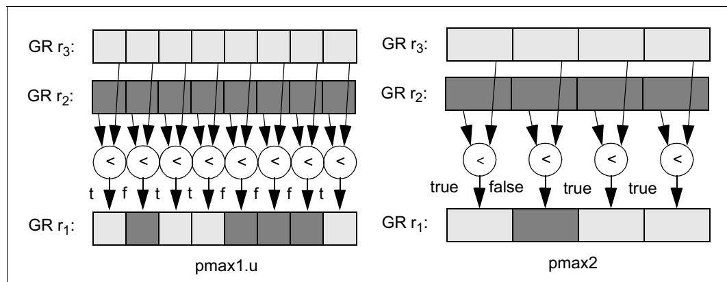
Figure 2-34. Parallel Maximum Example
