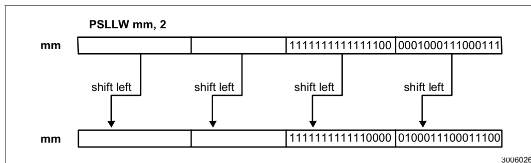
Figure 2-16. Operation of the PSLLW Instruction
