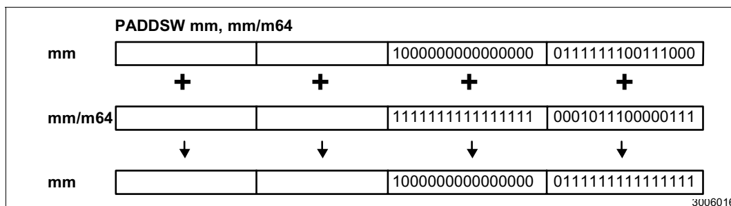
Figure 2-6. Operation of the PADDSSW Instruction
