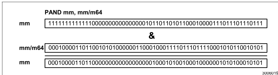
Figure 2-8. Operation of the PAND Instruction
