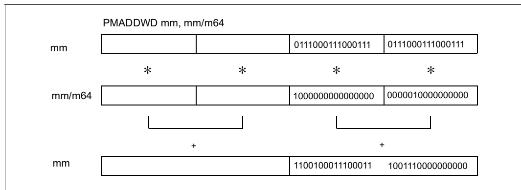
Figure 2-12. Operation of the PMADDWD Instruction
