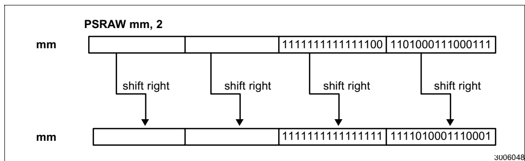
Figure 2-17. Operation of the PSRAW Instruction
