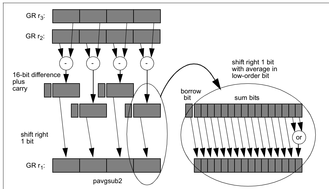
Figure 2-32. Parallel Average Subtract Example
