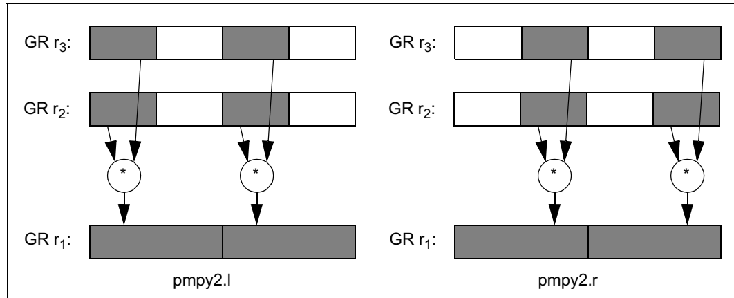
Figure 2-36. Parallel Multiply Operation
