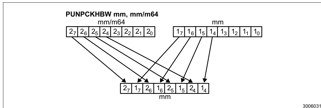
Figure 2-22. High-order Unpacking and Interleaving of Bytes with the PUNPCKHBW Instruction
