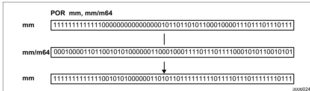
Figure 2-15. Operation of the POR Instruction.
