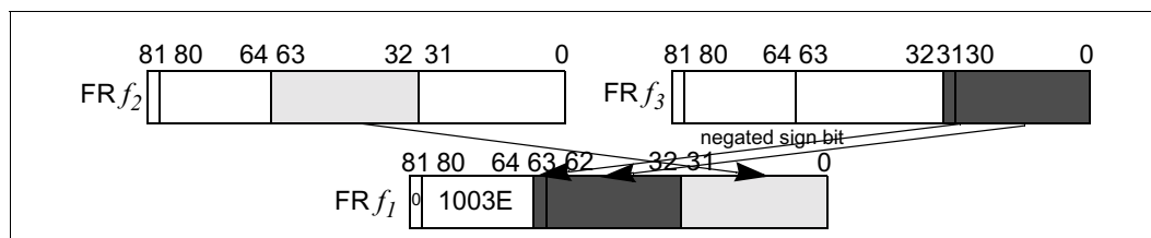
Figure 2-20. Floating-point Swap Negate Right
