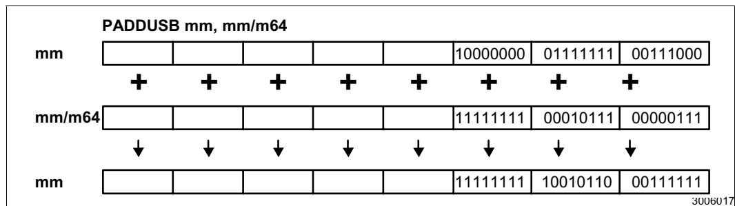
Figure 2-7. Operation of the PADDUSB Instruction
