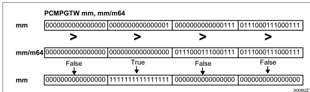
Figure 2-11. Operation of the PCMPGTW Instruction
