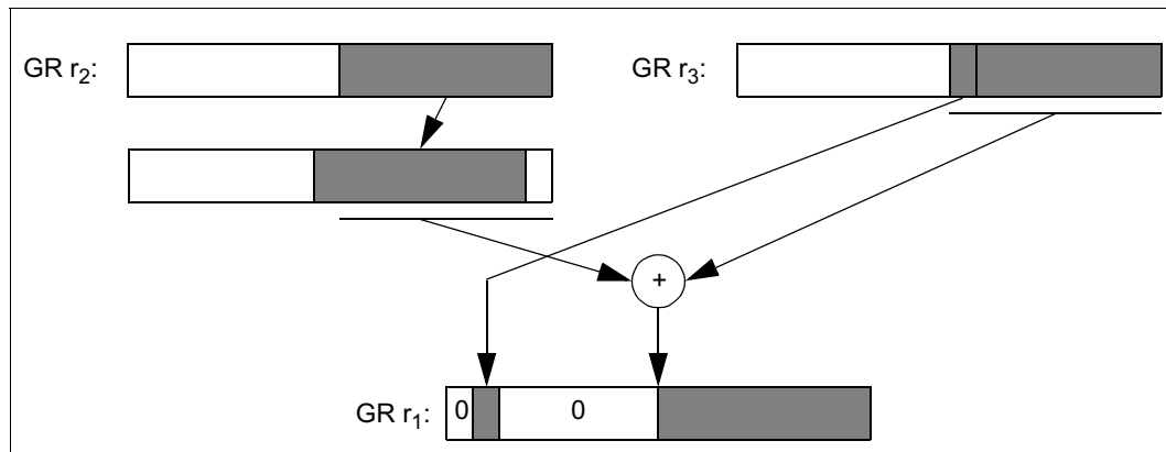
Figure 2-43. Shift Left and Add Pointer
