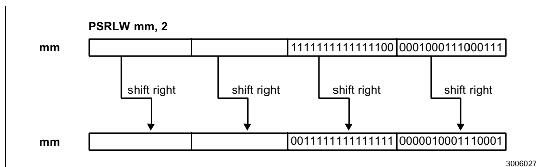
Figure 2-18. Operation of the PSRLW Instruction
