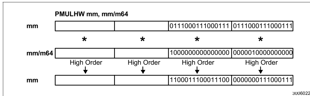
Figure 2-13. Operation of the PMULHW Instruction
