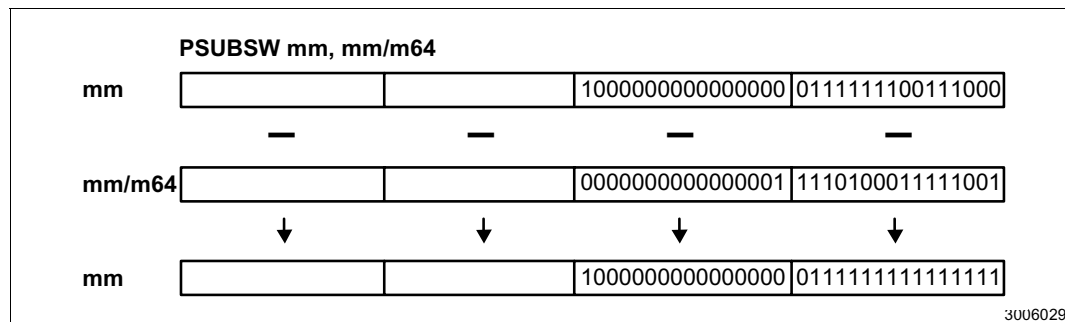
Figure 2-20. Operation of the PSUBSW Instruction
