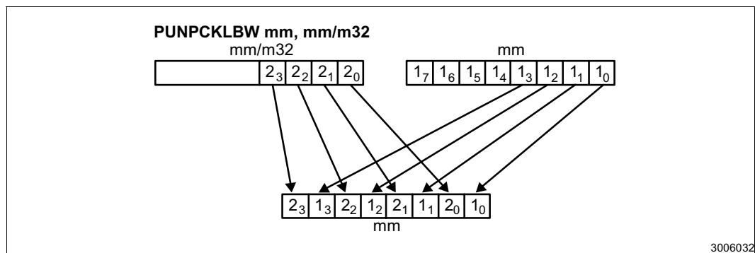
Figure 2-23. Low-order Unpacking and Interleaving of Bytes with the PUNPCKLBW Instruction
