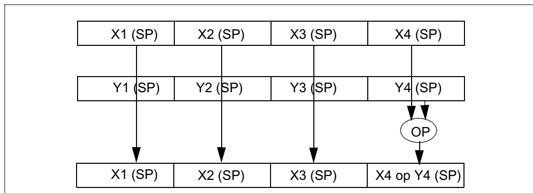
Figure 3-4. Scalar Operation
