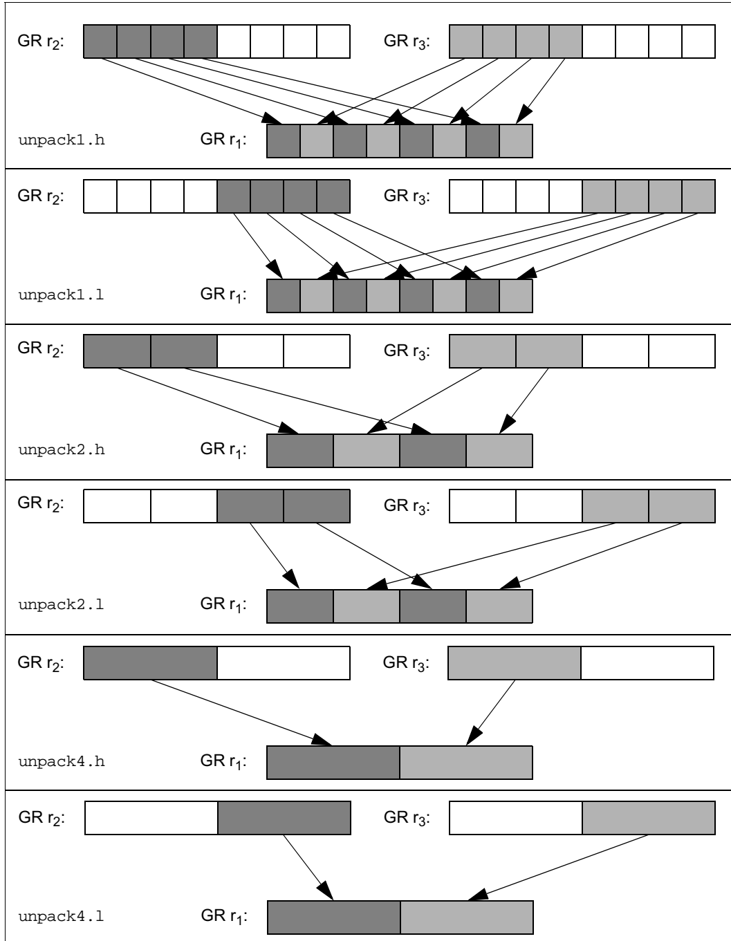
Figure 2-45. Unpack Operation
