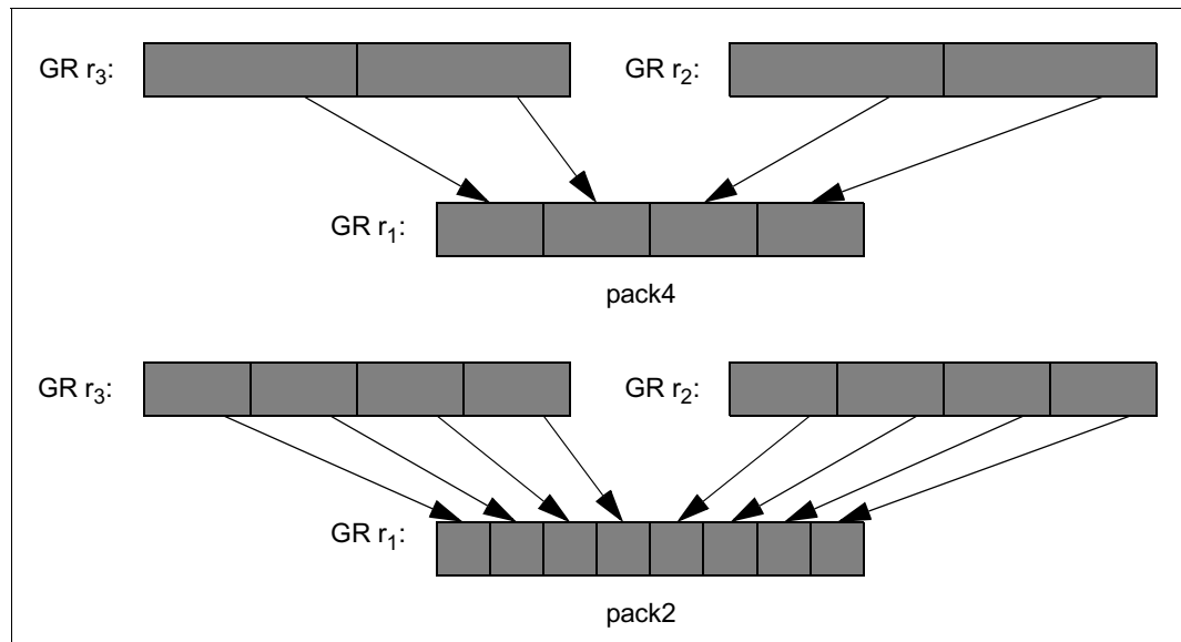
Figure 2-28. Pack Operation
