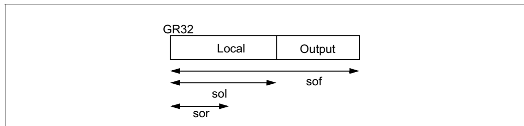
Figure 2-2. Stack Frame
