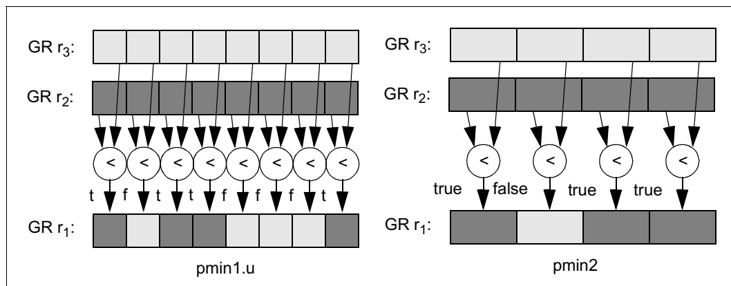
Figure 2-35. Parallel Minimum Example
