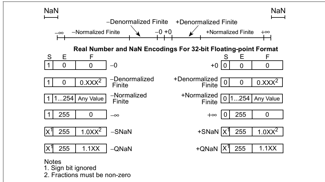
Figure 3-10. Real Numbers and NaNs
