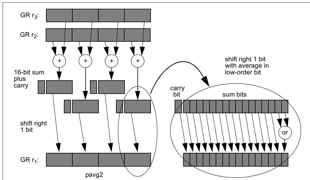
Figure 2-30. Parallel Average Example
