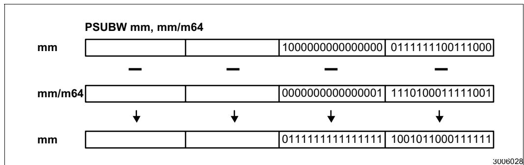
Figure 2-19. Operation of the PSUBW Instruction
