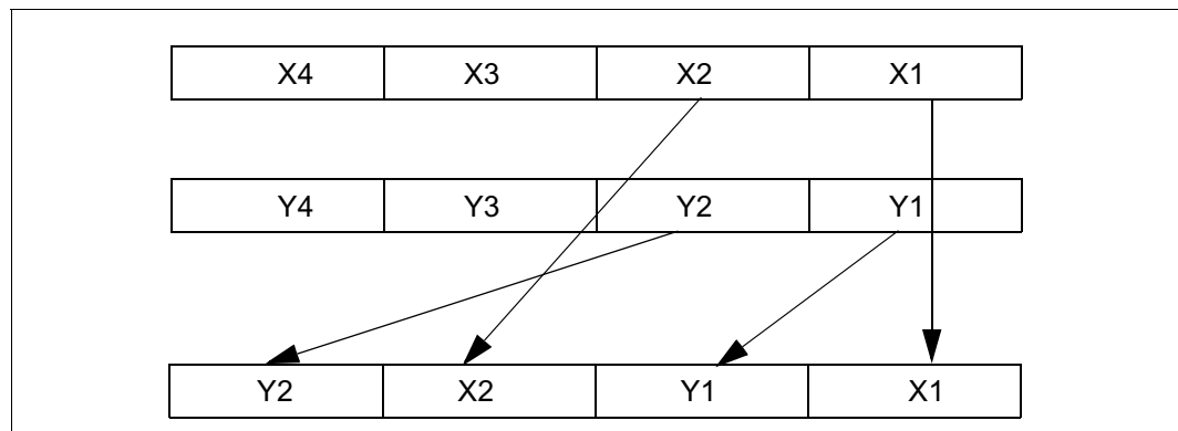
Figure 3-7. Unpack Low Operation
