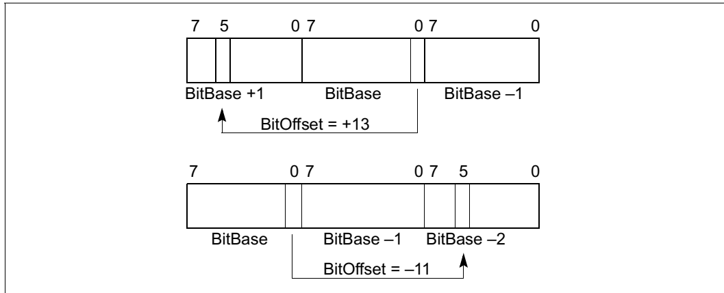
Figure 1-2. Memory Bit Indexing
