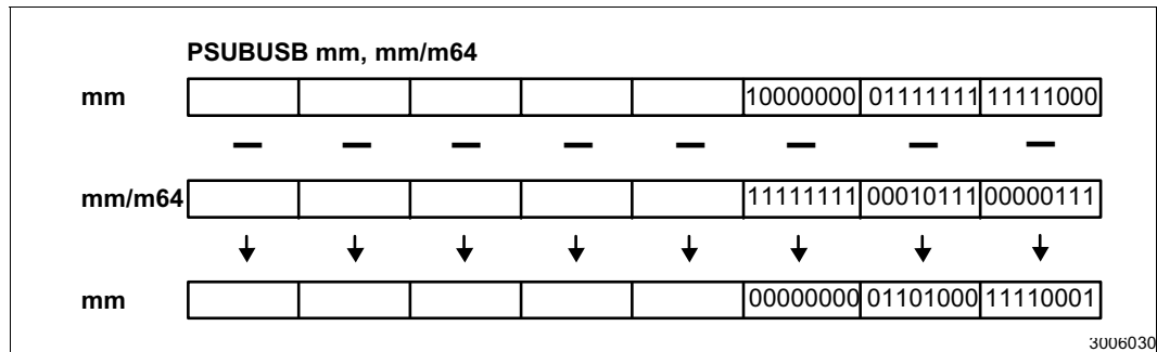
Figure 2-21. Operation of the PSUBUSB Instruction
