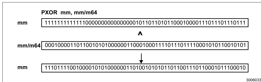
Figure 2-24. Operation of the PXOR Instruction
