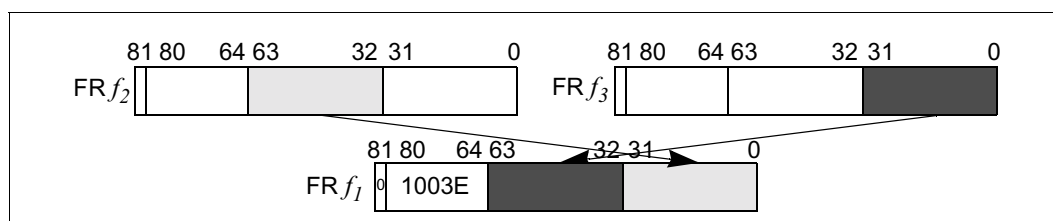
Figure 2-19. Floating-point Swap Negate Left
