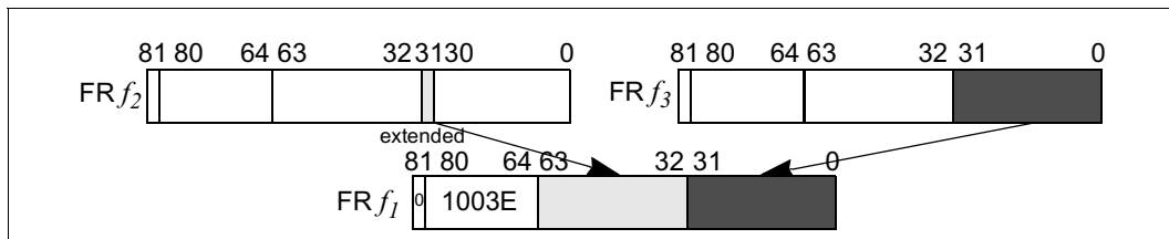
Figure 2-22. Floating-point Sign Extend Right
