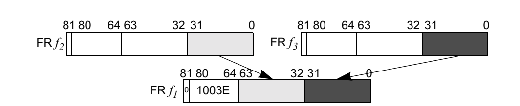
Figure 2-13. Floating-point Mix Left-Right
