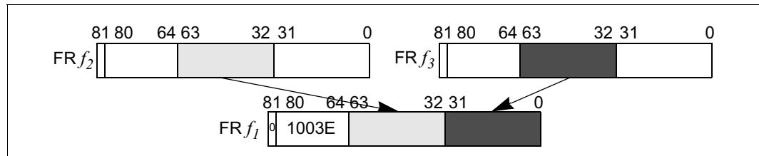
Figure 2-12. Floating-point Mix Right
