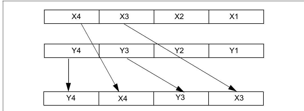
Figure 3-6. Unpack High Operation
