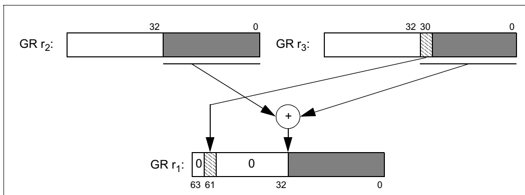
Figure 2-1. Add Pointer
