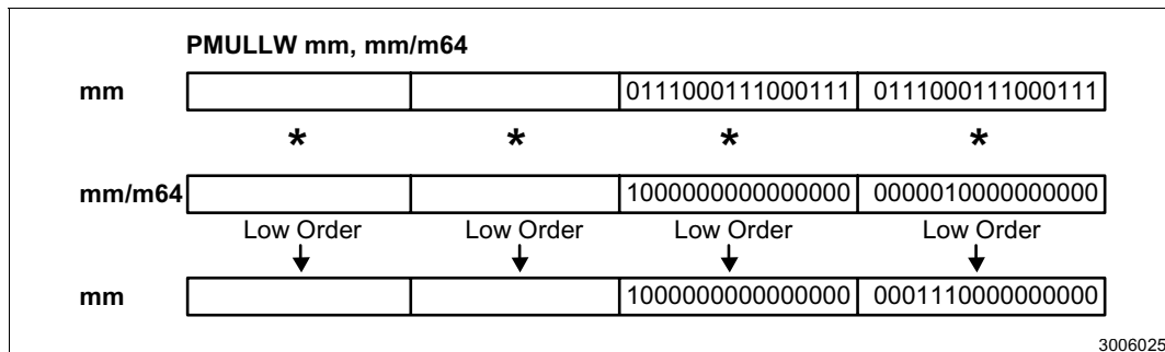
Figure 2-14. Operation of the PMULLW Instruction
