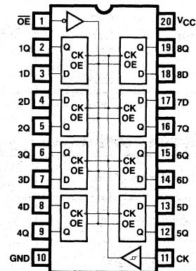
374 Octal Register
