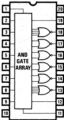
PAL12L6
