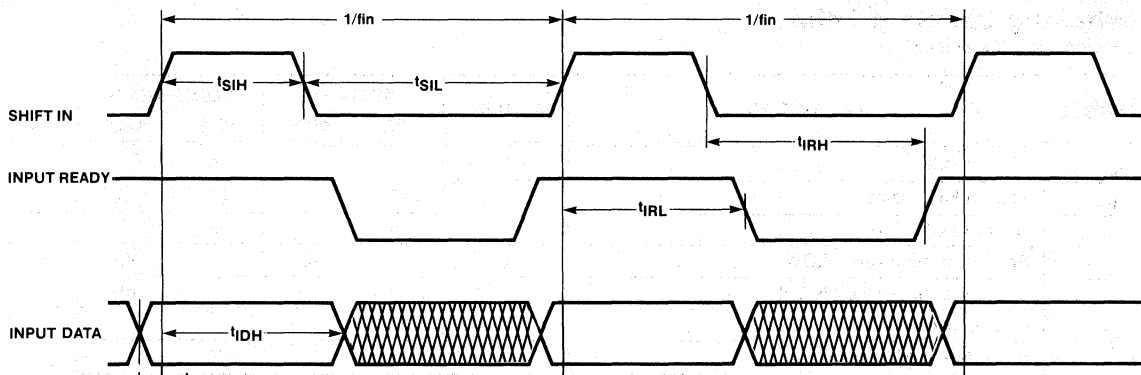
Figure 1. Input Timing
