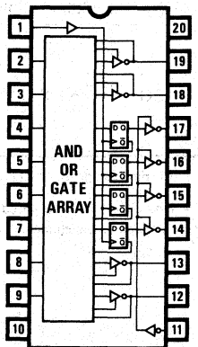
PAL16R4
