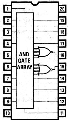
PAL16L2
