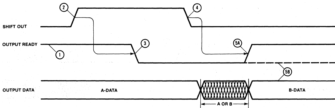
Figure 8. The Mechanism of Shifting Data Out of the FIFO.
