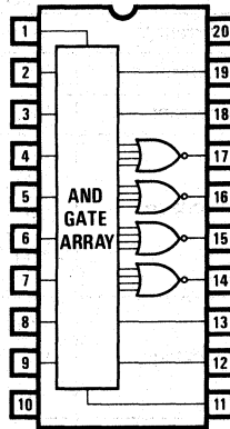
PAL14L4
