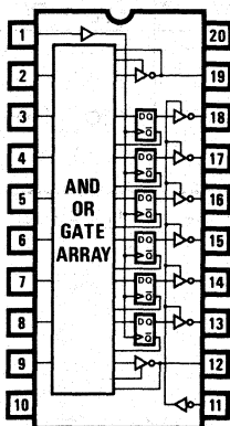
PAL16R6
