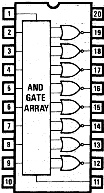
PAL10L8
