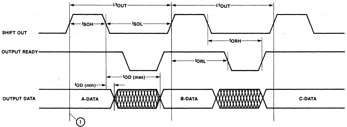
Figure 6. Output Timing
