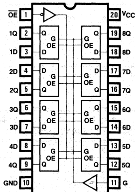
373 Octal Latch
