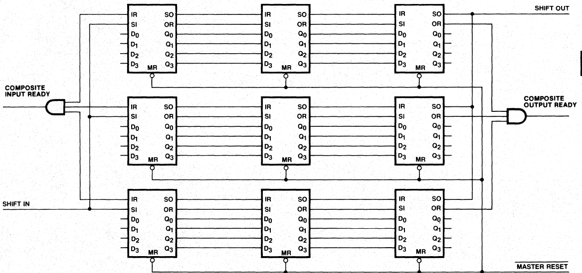
Figure 13. 192x12 FIFO.
