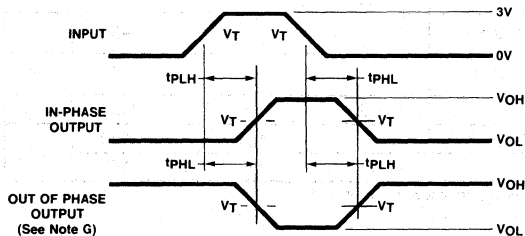
Propagation Delay
