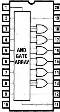
PAL12H6
