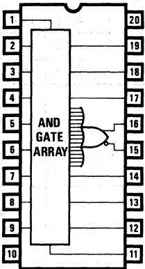
PAL16C1
