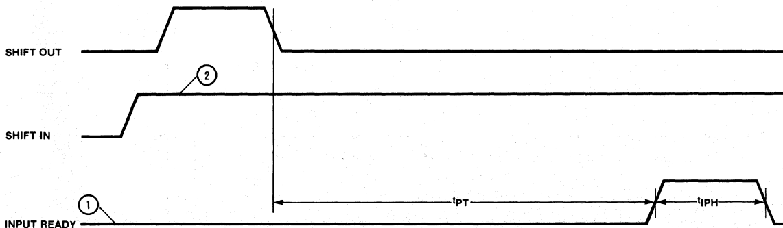
Figure 4. t_{IPH} Specification
