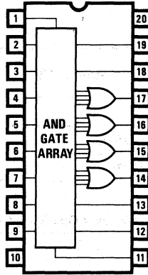
PAL14H4
