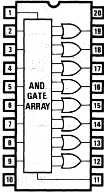
PAL10H8
