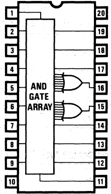
PAL16H2
