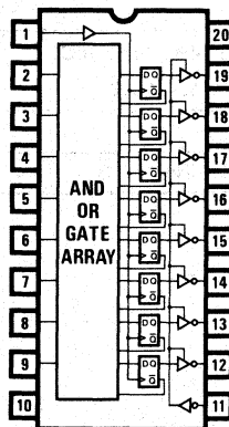
PAL16R8
