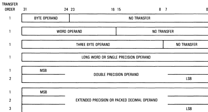
Figure 7-4. Operand CIR Data Alignment
