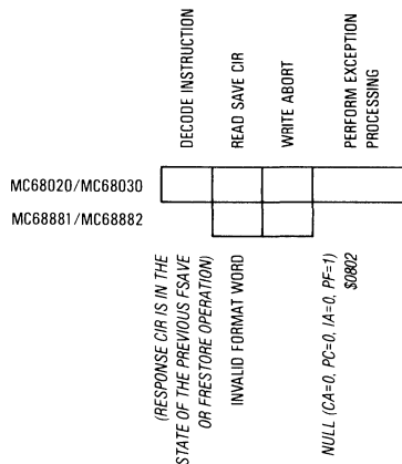
Figure 7-39. FSAVE Format Exception Dialog
