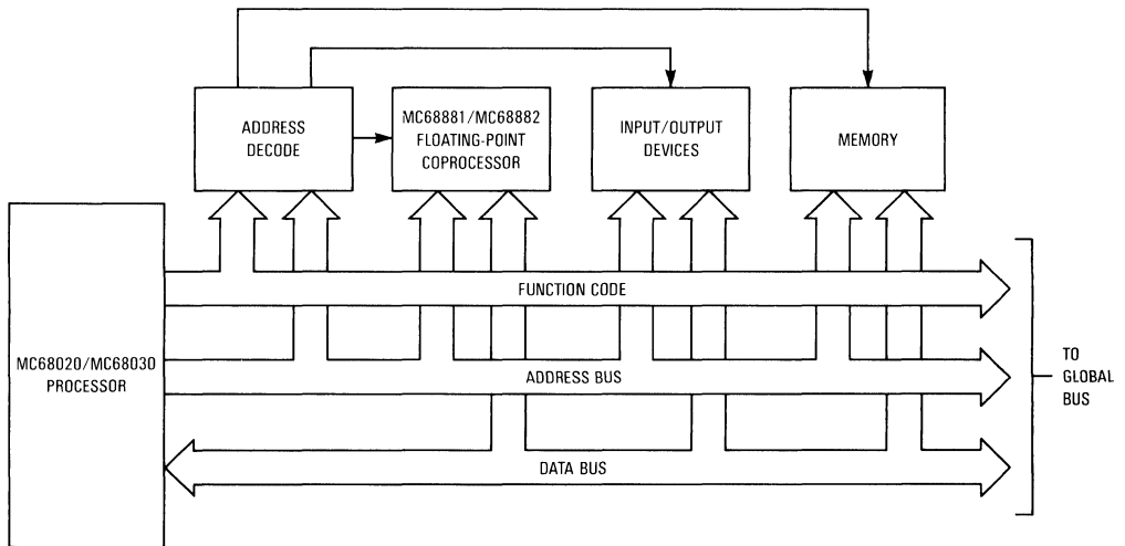
Figure 1-7. Typical Coprocessor Configuration
