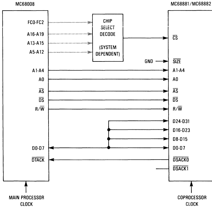
Figure 11-5. 8-Bit Data Bus Peripheral Processor Connection
