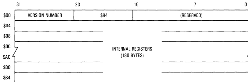
Figure 6-4. MC68881 State Frame Formats
