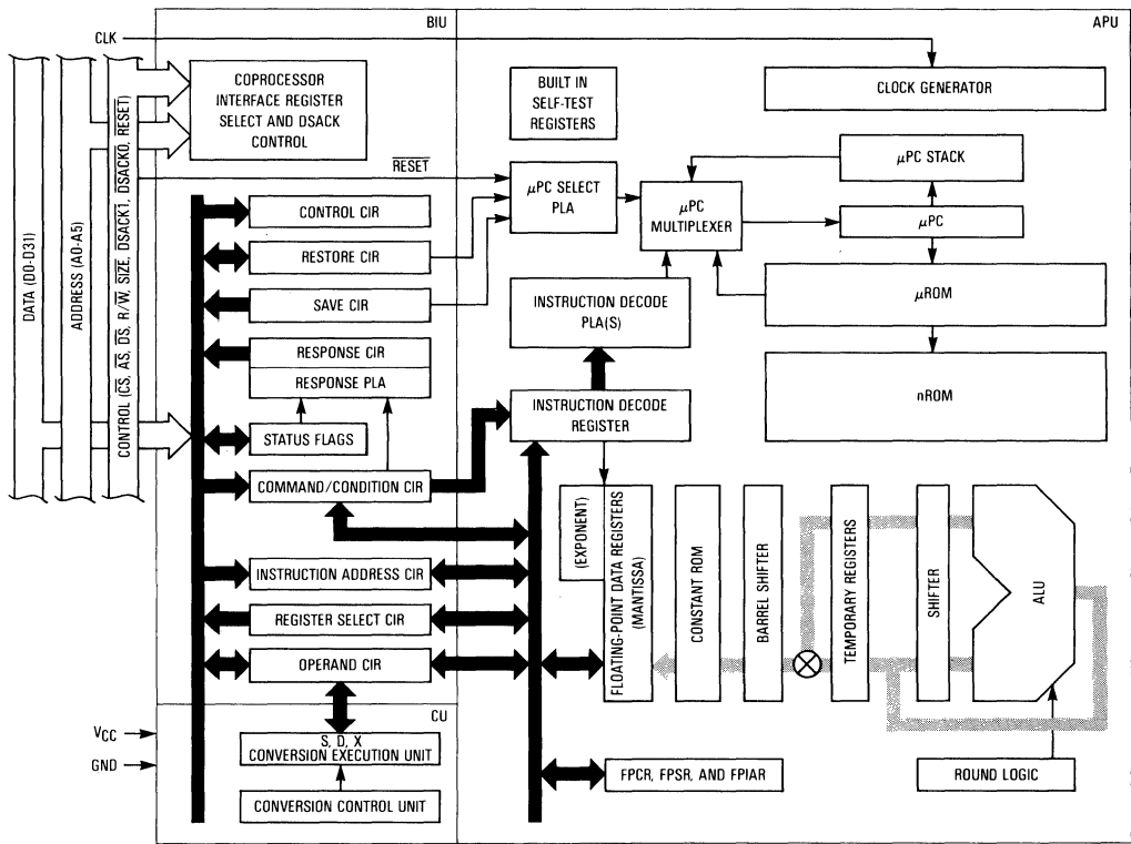
Figure 1-9. MC68882 Simplified Block Diagram
