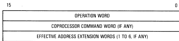
Figure 7-5. Coprocessor Instruction General Format
