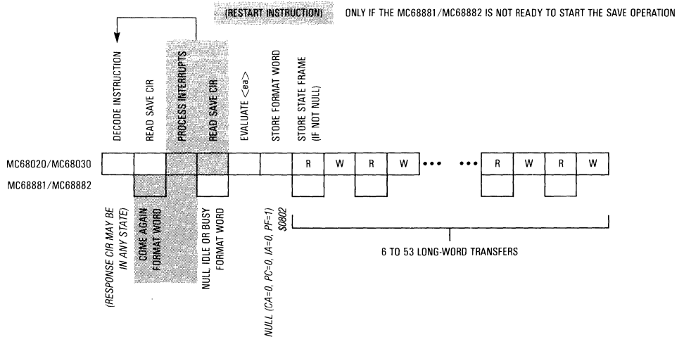
Figure 7-25. FSAVE Instruction Dialog
