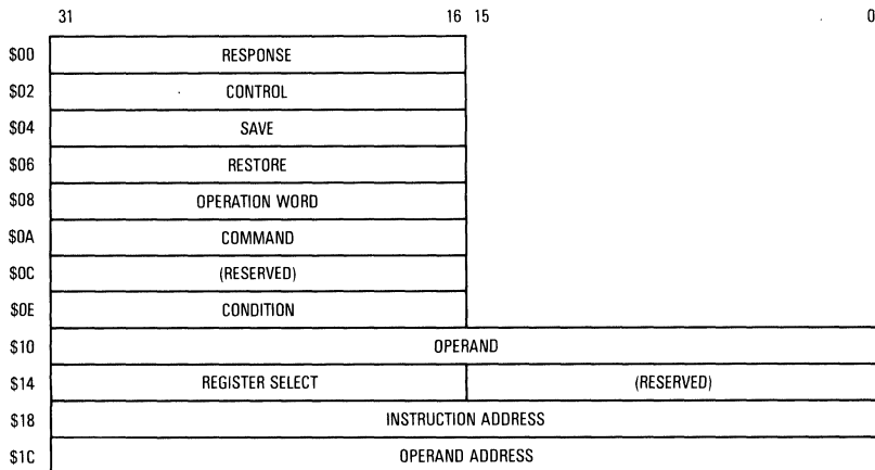
Figure 7-2. FPCP Coprocessor Interface Register Map
