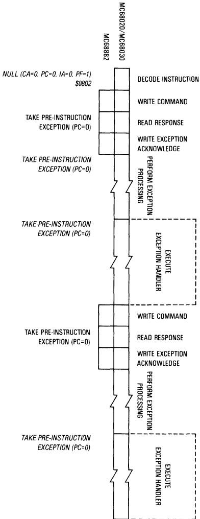
Figure 7-29. Take Pre-Instruction Exception Dialog — MC68882 with No FSAVE Instruction in the Handler
