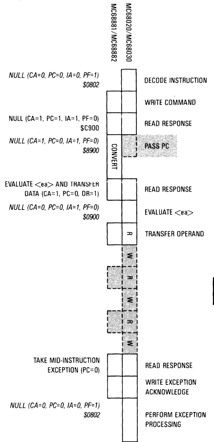
Figure 7-32. Take Mid-Instruction Exception Dialog — MC68882 General Concurrent Case
