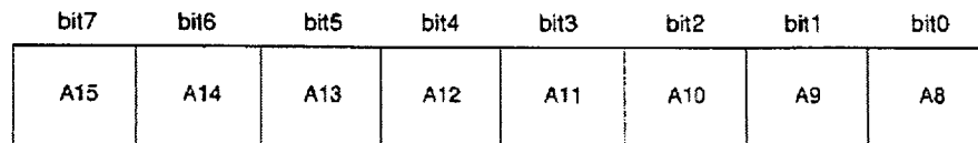
CPU DMA Address Counter Middle (19H)
