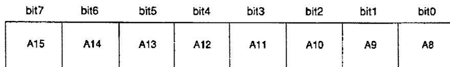
Host DMA Transfer Counter Upper (17H)
