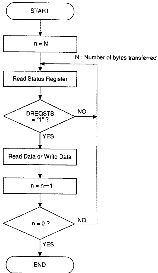
Fig. 4.3 Example of data transfer control in I/O mode
