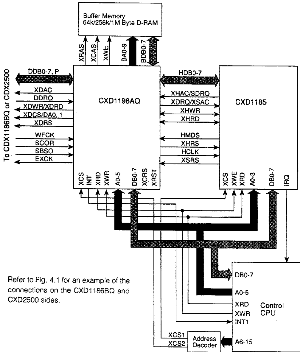
Fig. 4.4 Example of connection with SCSI control LSI
