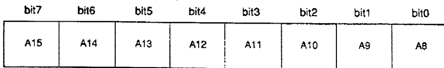
CPU DMA Address Counter Middle (19H)
