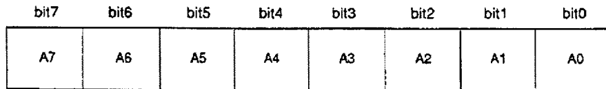
Host DMA Transfer Counter Lower (16H)
