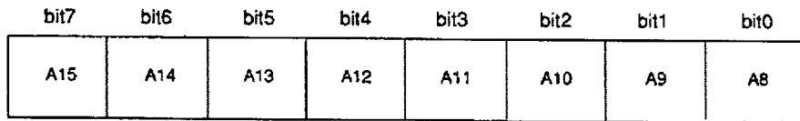
Host DMA Transfer Counter Upper (17H)
