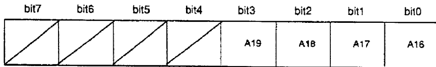
Host DMA Address Counter Upper (15H)
