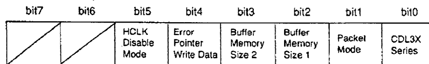
Configuration Register (1BH)
