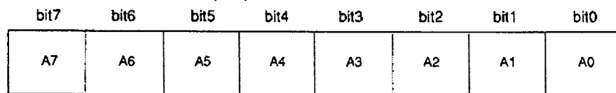
CPU DMA Address Counter Lower (18H)
