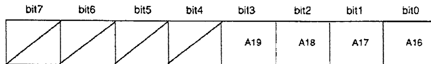
CPU DMA Address Counter Upper (1AH)
