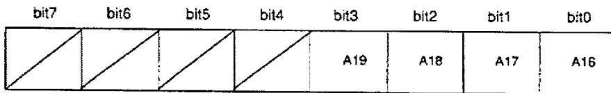
CPU DMA Address Counter Upper (1AH)
