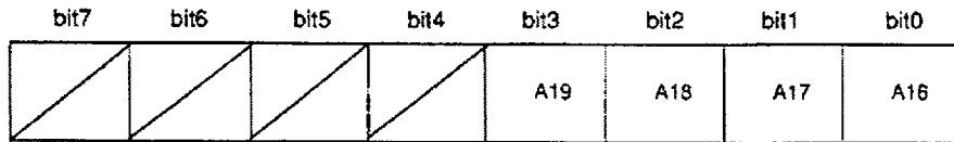
Host DMA Address Counter Upper (15H)
