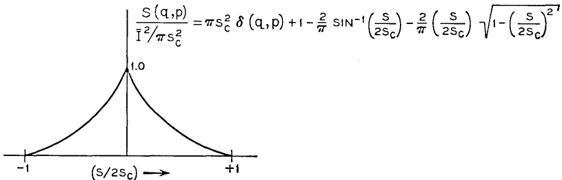
Fig. 2 — Section of the spatial power spectral density for a uniform diffuse surface imaged through a circular aperture. The complete two dimensional spectrum is obtained by rotating the above curve about the vertical axis.
