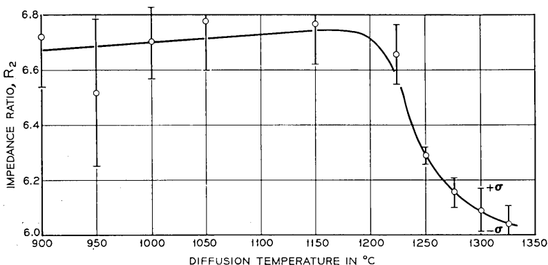
Fig. 9—Impedance ratio, R_2 = Z(50\mu A)/Z(300\mu A) , as a function of gold diffusion temperature. Diffusion time 10 minutes. Contact sinter time 3 minutes.
