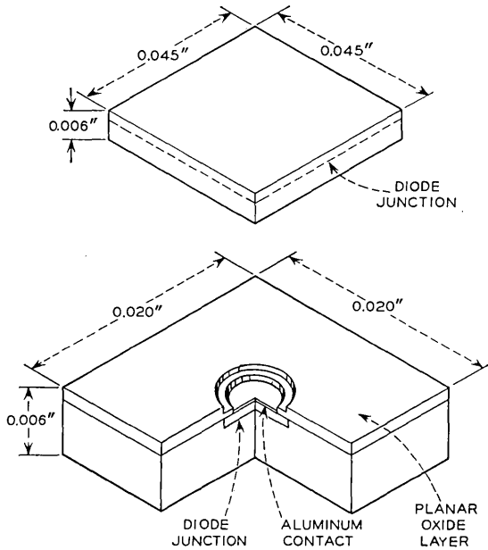
Fig. 3—(a) Mesa structure of component diodes. (b) Planar structure of component diodes.
