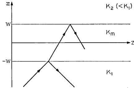
Fig. 4—A schematic diagram of the totally reflected wave in the asymmetric step model. The wave is incident on the junction region at x = -w where it is partly reflected and partly transmitted. The partly transmitted portion is then totally reflected at x = w .
