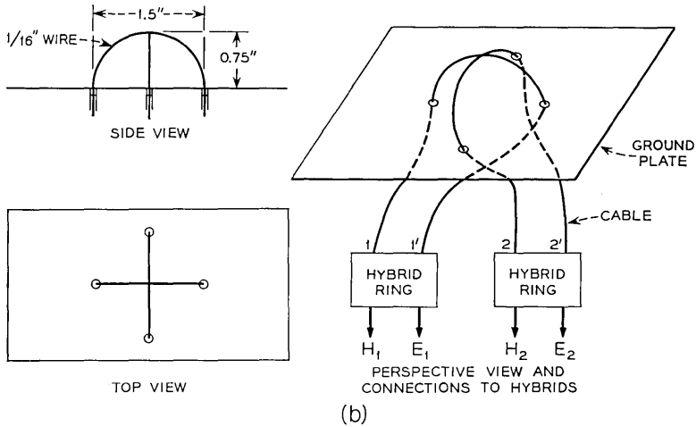
Fig. 1—(a) Experimental set-up. (b) Energy-density antenna—double orthogonal loop antenna.
