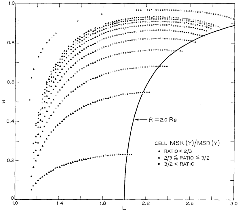
Fig. 60 — Positions of centers of regions in x,L space having certain ranges of cell MSR( Y )/MSD( Y ). The ranges are indicated in the legend. (Plotted points are mid-points for the cells. Points appearing to the right of the boundary R = 2.0 R_e represent cells which have data only in one corner.)
