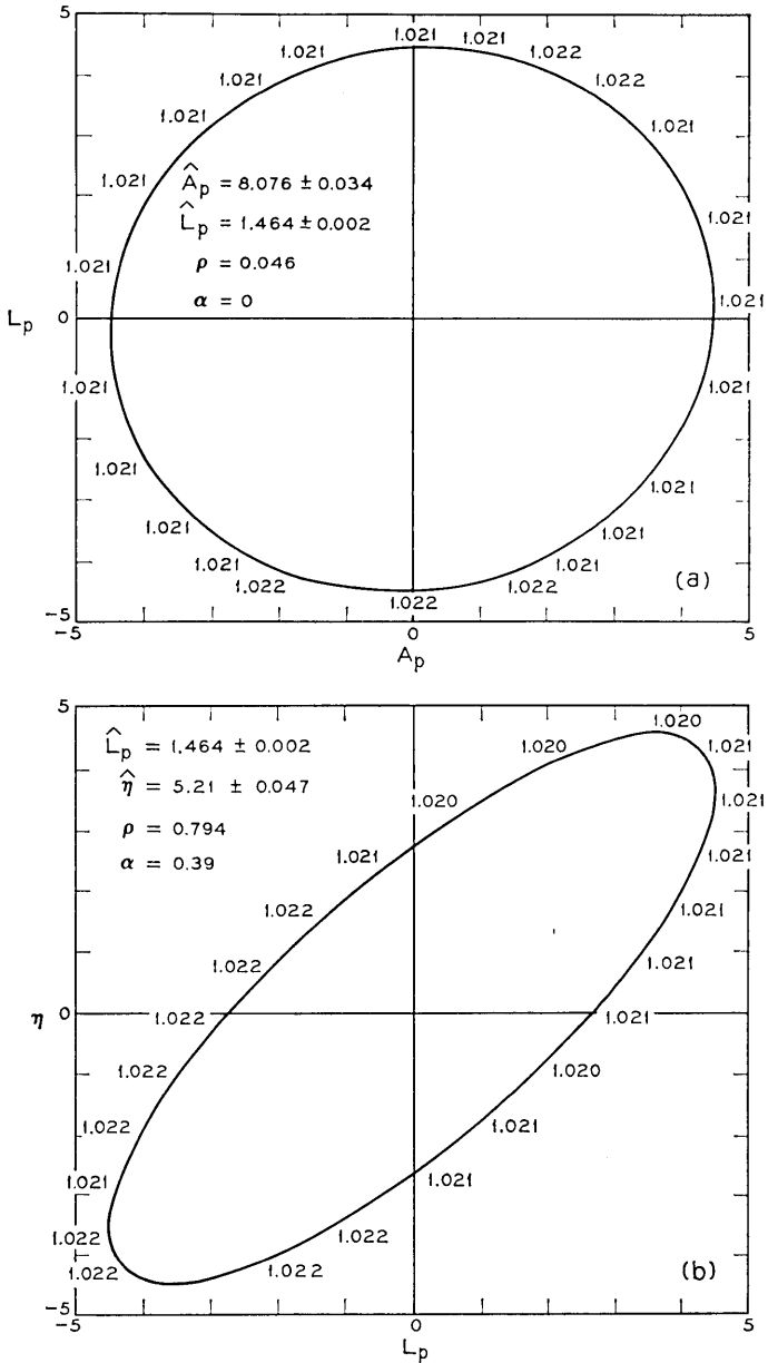
Fig. 39—Examples of projections of the approximate “0.99 joint confidence region” for the estimates of Model II. (Axes are scaled by standard errors.)
