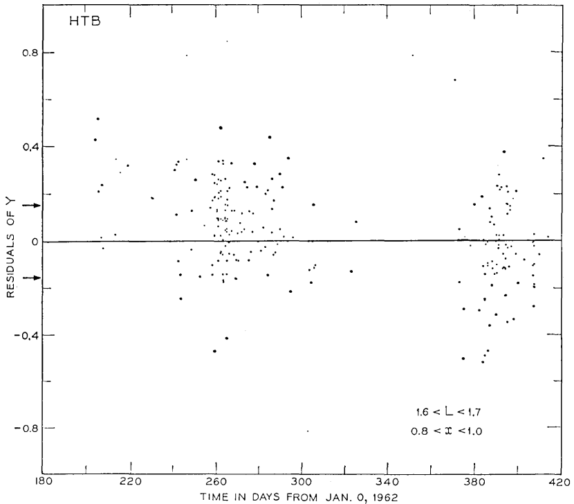
Fig. 41 — HTB residuals of Y (i.e., Y - y calculated from the HTB coefficients) plotted against time for 1.6 < L < 1.7 and 0.8 < x < 1.0 . The arrows indicate \pm the approximate standard deviation if Y^2 were Poisson distributed.
