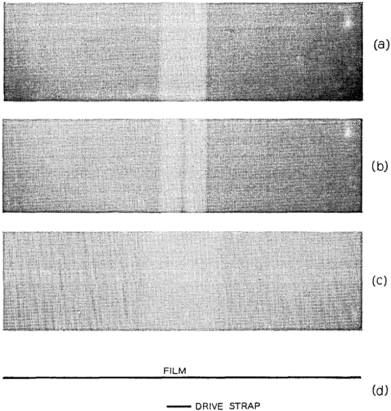
Fig. 20 — (a) Kerr effect picture showing reversed domain (light) in a flat film written in by an 11 mil drive strap situated 10 mils beneath the film. (b) When bias field is reversed, the domain is not completely erased. (c) Width of domain written after first demagnetizing film with a large uniform hard axis field. (d) Shows the drive strap arrangement to the same scale.
