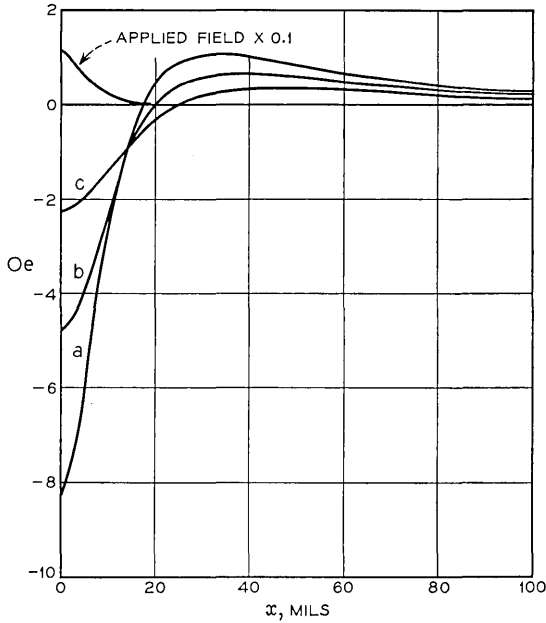
Fig. 13 — External axial component of field due to the distribution of magnetization along a cylindrical film. (The field due to the drive strap is not included.) The field is plotted along lines parallel to the film axis, at several distances from the axis. The film has a thickness of 1\mu\text{m} , H_K = 3.0 Oe, diameter 5.2 mils, and is subject to the field from a one turn circular loop of diameter 15 mils. Curves a, b, and c refer to distances of 2.6, 5.0, and 10 mils from the axis, respectively.
