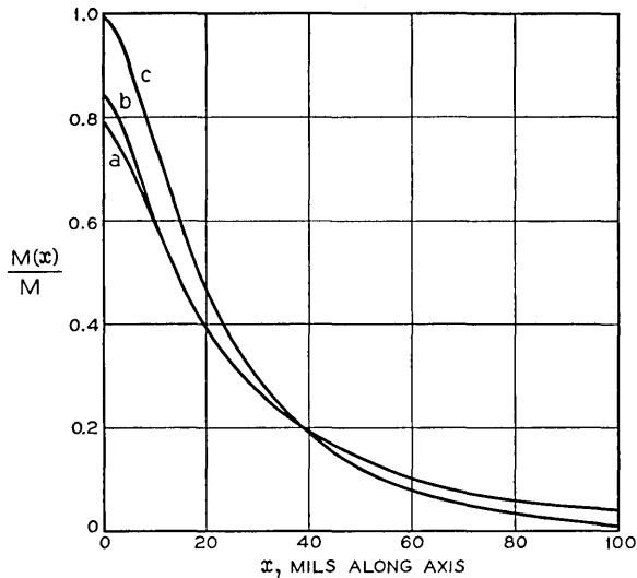
Fig. 18—Effect of a cylindrical keeper layer on the axial magnetization distribution in a cylindrical film of thickness 1.0\mu\text{m} , H_K = 3.0 \text{ oe} , diameter 5.2 mils. Field is applied by a one turn loop of radius 7.5 mils. Keeper radius is taken to be 10 mils. Curve a shows the distribution with no keeper present, curve b shows the effect of the keeper in modifying the applied field, and curve c shows the final result when field modification and flux closure are taken into account.
