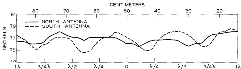
Fig. 2 — Amplitude of signal strength along the slot receiving from one transmitting antenna only.
