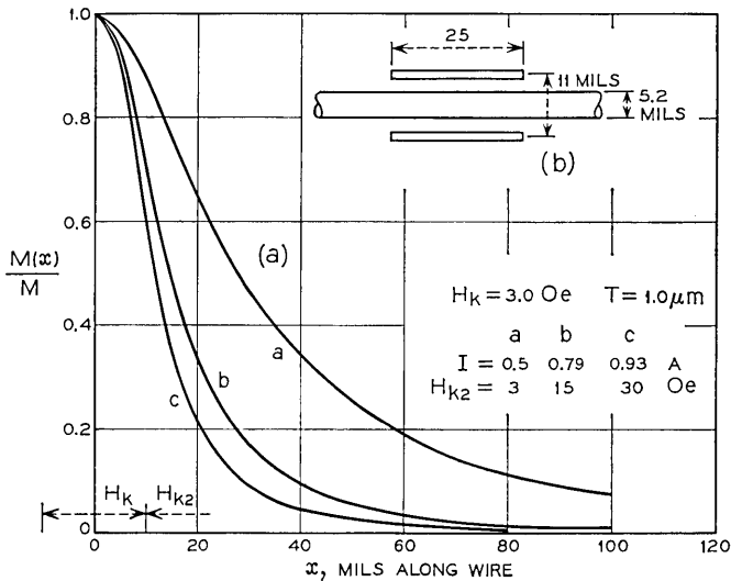
Fig. 12 — (a) Effect of high H_K buffer region surrounding a normal H_K section of cylindrical film. Curve a shows the magnetization component for a uniform film with H_K = 3.0 . Curves b and c show the result when H_K is increased to 15 and 30 Oe, respectively for distances greater than 10 mils to either side of the drive strap centerline. (b) Details of drive strap arrangement. The currents required to just saturate the film at x = 0 are 0.5, 0.79, and 0.93 A for the cases a, b, and c, respectively.
