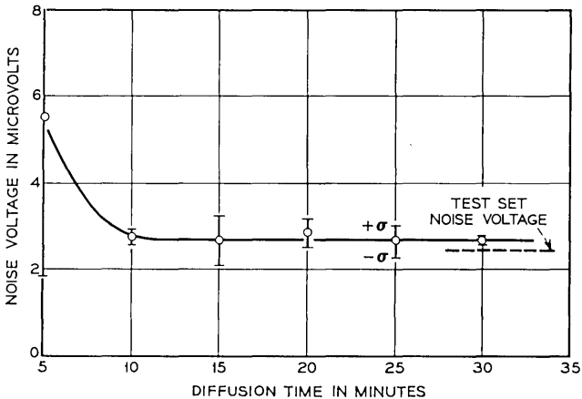
Fig. 15—Noise voltage (200–3500 Hz) at 2.5\mu\text{A} bias current as a function of gold diffusion time. Diffusion temperature 1300^\circ\text{C} . Contact sinter time 10 minutes.
