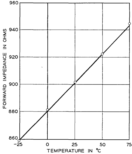
Fig. 18—Typical forward impedance at 50 \mu A bias current as a function of temperature.
