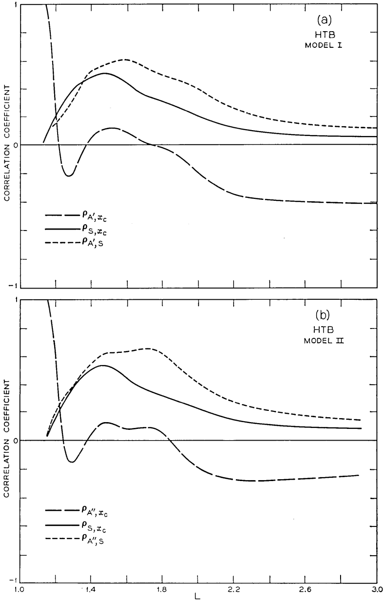
Fig. 30—Correlation coefficients of A with S , S with x_c , and A with x_c , calculated from the fits to the HTB sample and plotted as functions of L . (a) Model I. (b) Model II.
