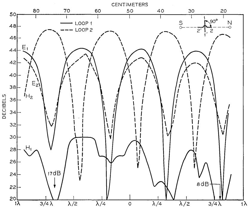
Fig. 7—Standing waves of H fields and E fields along the slot by using a double orthogonal semiloop antenna unconnected at the top point (oriented at 90^\circ ).
