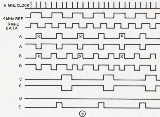
for 6-MHz data rate (b). Any reference less than half the clock frequency could be used.
