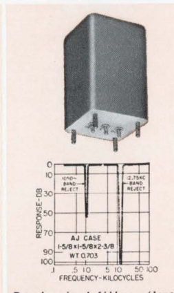
Band reject filters (two shown). The 1050 filter has 50 db attenuation and is only 3 db at 950 and 1150 cycles. The 12.75 KC filter has more than 100 db attenuation and is only 3 db at 10.8 and 15 KC. Source and load 600 ohms, both are MIL-F-18327B.
