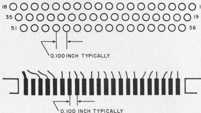
2. Typical pin-type and finger-type connectors used for input-output terminals in multilayer designs. Pin-types offer greater flexibility if additional contacts are needed in the final stages of design.
