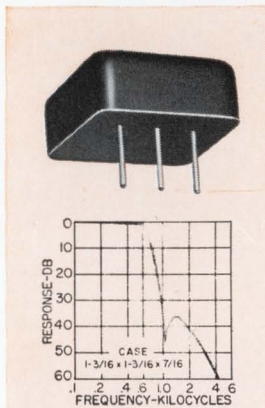
560 — Telemetry low pass filter. Available from 400 to 70 KC. \pm 7.5\% bandwidth flat to 1 db. Attenuation greater than 35 db beyond the 2nd harmonic of \pm 7.5\% frequency. Impedance 47K ohms. MIL-F-18327B. Wt. 0.8 oz.
