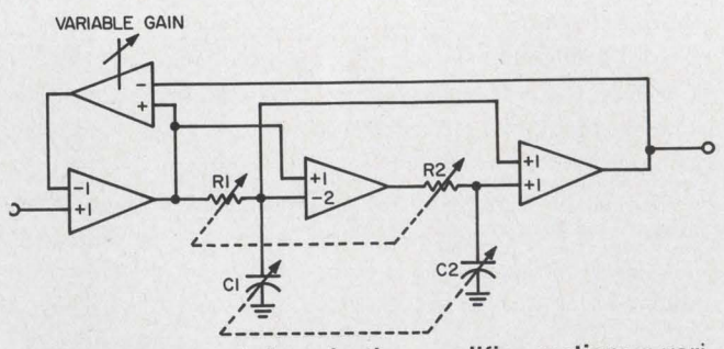
3. Block diagram of the selective amplifier section: a variable-gain amplifier controls Q from 1 to 100.
