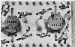
Top view of CTS hybrid integrated circuit showing attached discrete components and terminal pins soldered through holes in substrate.
