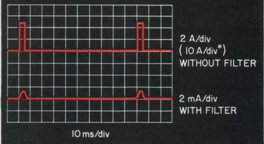
Typical example of A-B Active Filter performance
