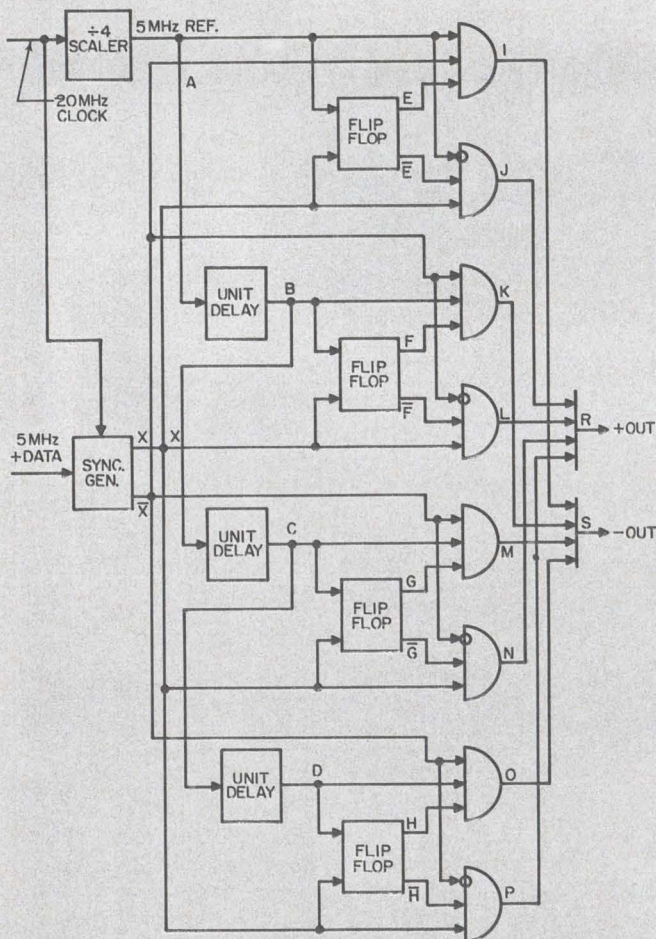
3. The digitizer's resolution can be increased by the addition of logic circuitry that will generate more than one pulse per cycle of phase difference. The number of output pulses obtained is equal to the number of channels added to the basic digitizer.
