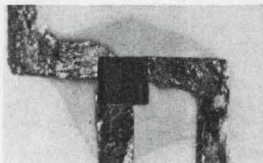
Enlarged view of flip chip assembly to ceramic substrate with platinum gold conductors.
