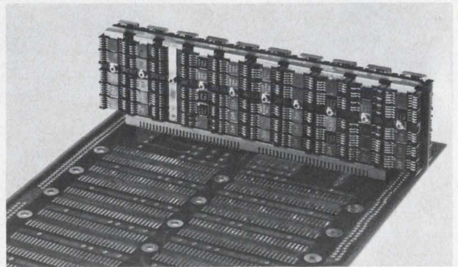
1. Multilayer "grandmother" board interconnects groups of smaller boards. Changes in logic design can often be incorporated by alteration of the external wiring of the "grandmother" board.
