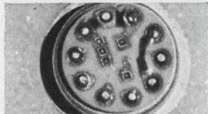
TO5 header showing cermet resistors and transistor dice.
