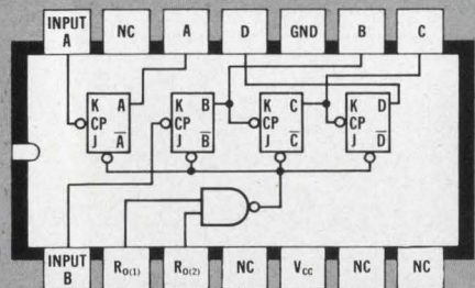
SN7493N FOUR BIT BINARY COUNTER
