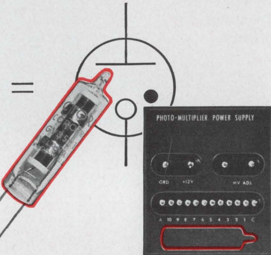
Corotron actual size: Photo-multiplier power supply, showing Corotron location, \frac{2}{3} size.
