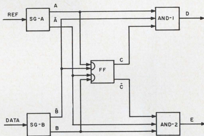
1. Readily available IC modules are used to build this synchronous bidirectional digitizer. The circuit is simple, compact, and requires no calibration.
