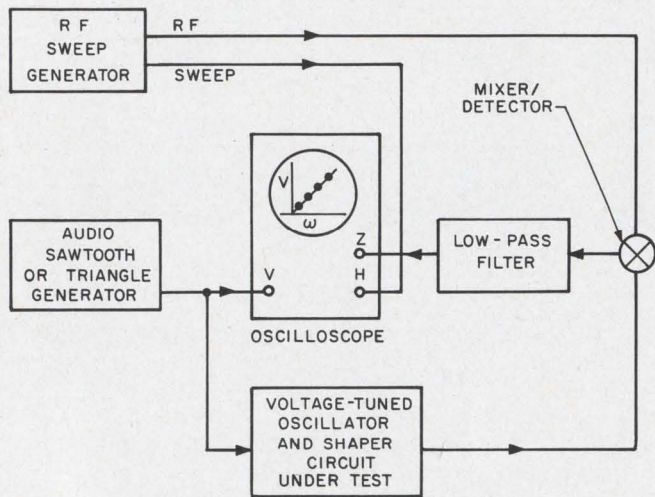
Visual adjustment of voltage-tuned oscillators is simple with the hook-up shown above.
