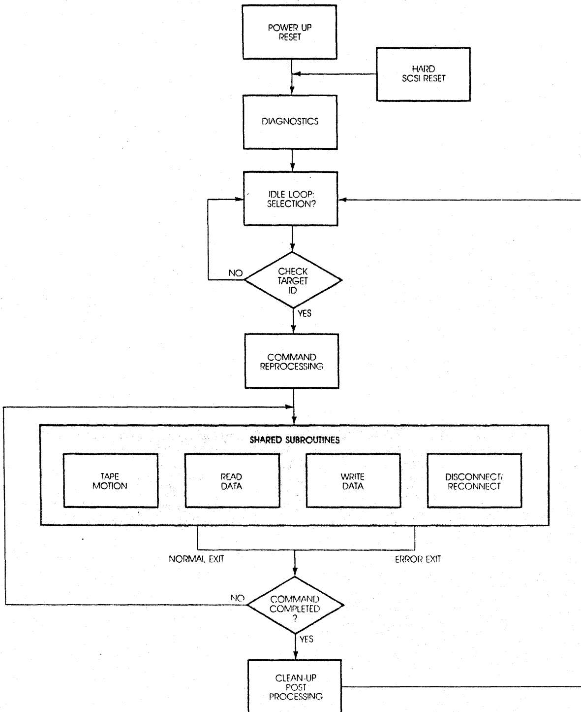
FIGURE 2-2. ACB-3530A CONTROLLING FIRMWARE
