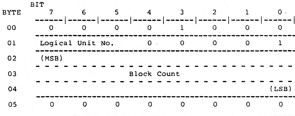
FIGURE 6-8. READ COMMAND
