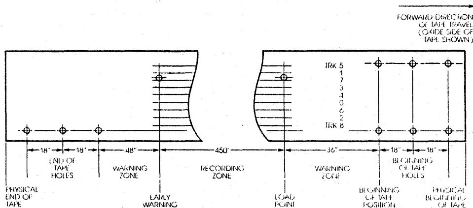
FIGURE 4-2. 1/4" TAPE LAYOUT
