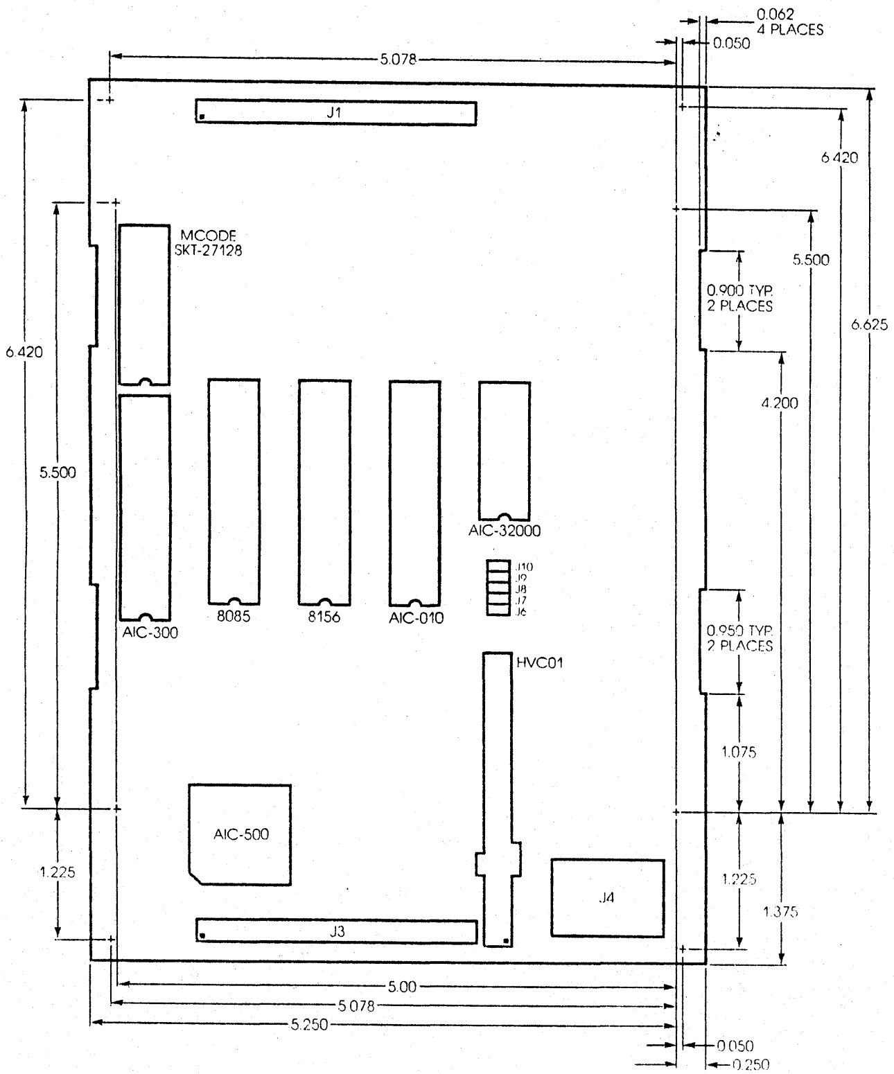
FIGURE 1-1. ACB-3530A BOARD LAYOUT
