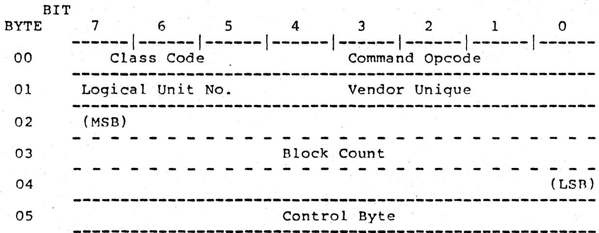
FIGURE 5-5. CLASS 0 CDB SUPPORTED BY THE ACB-3530A
