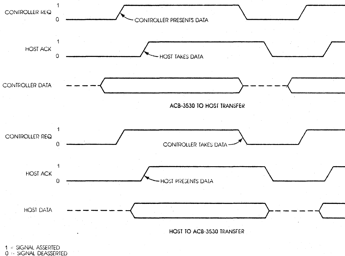
FIGURE 5-2. REQ/ACK HANDSHAKE
