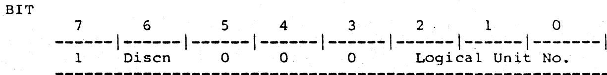
FIGURE 5-7. IDENTIFY MESSAGE
