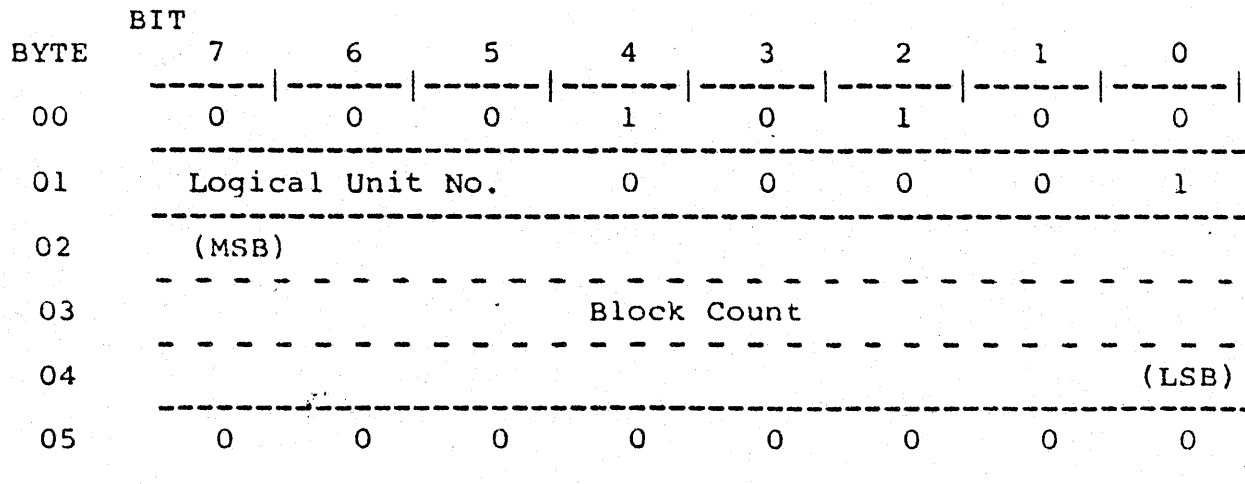
FIGURE 6-15. RECOVER BUFFER DATA COMMAND
