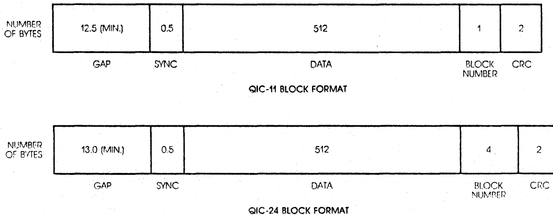
FIGURE 4-1. QIC-11 AND QIC-24 BLOCK FORMAT
