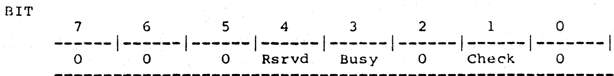
FIGURE 5-6. COMPLETION STATUS BYTE
