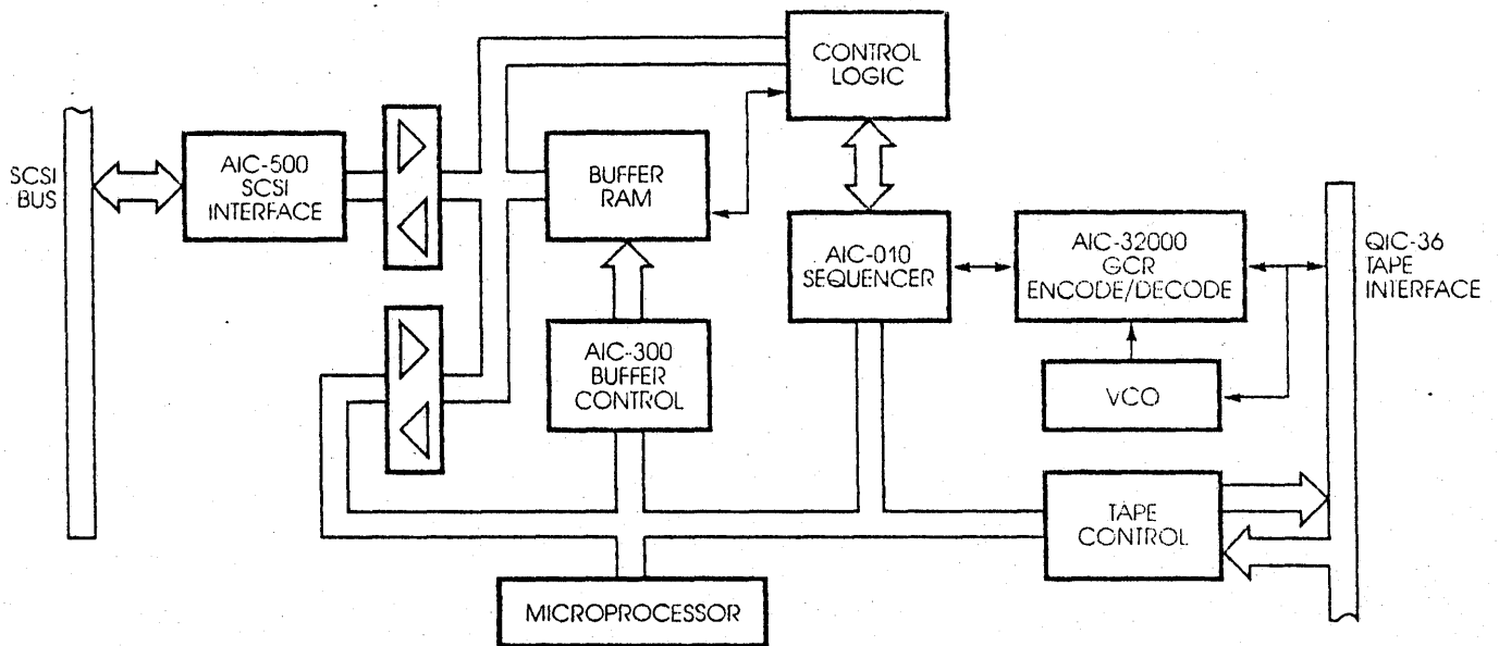
FIGURE 2-1. ACB-3530A BLOCK DIAGRAM
