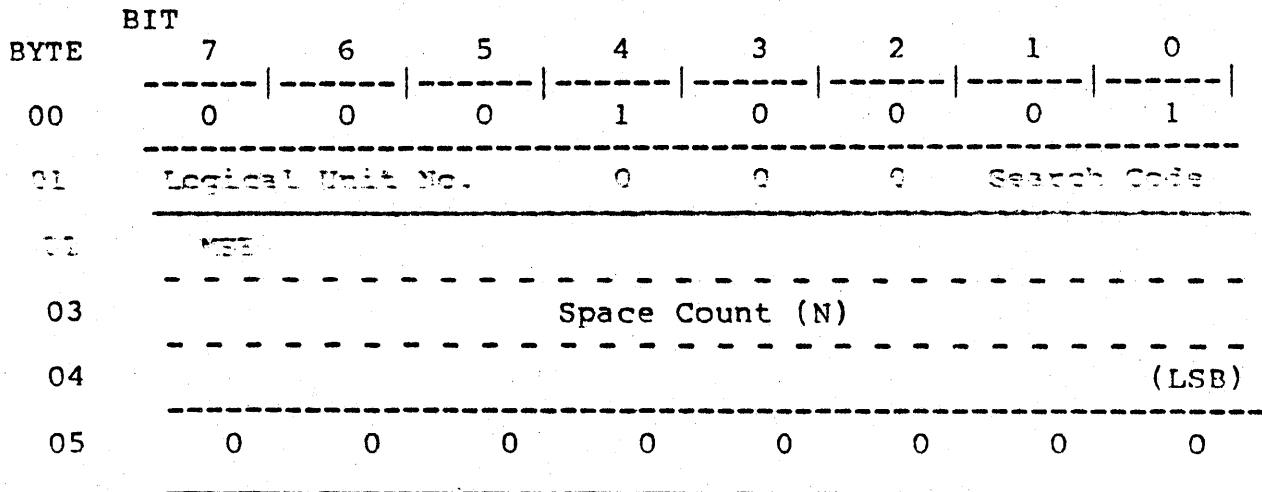
FIGURE 6-11. SPACE COMMAND
