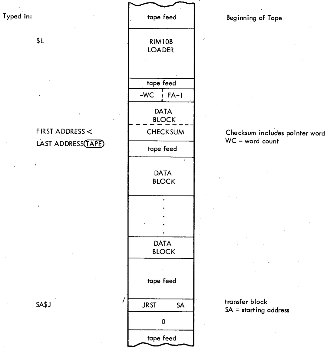
Figure 6-1 RIM10B Block Format
