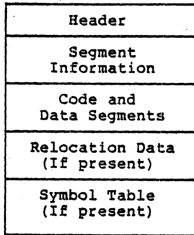
Figure 3-1. CP/M-8000 Command File Layout
