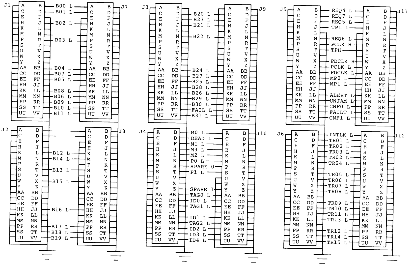
Figure 2-4 SBI Signal Names and Pin Assignments
