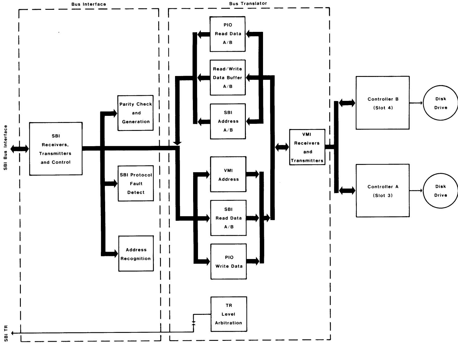
Figure 2-1 V-MASTER Block Diagram
