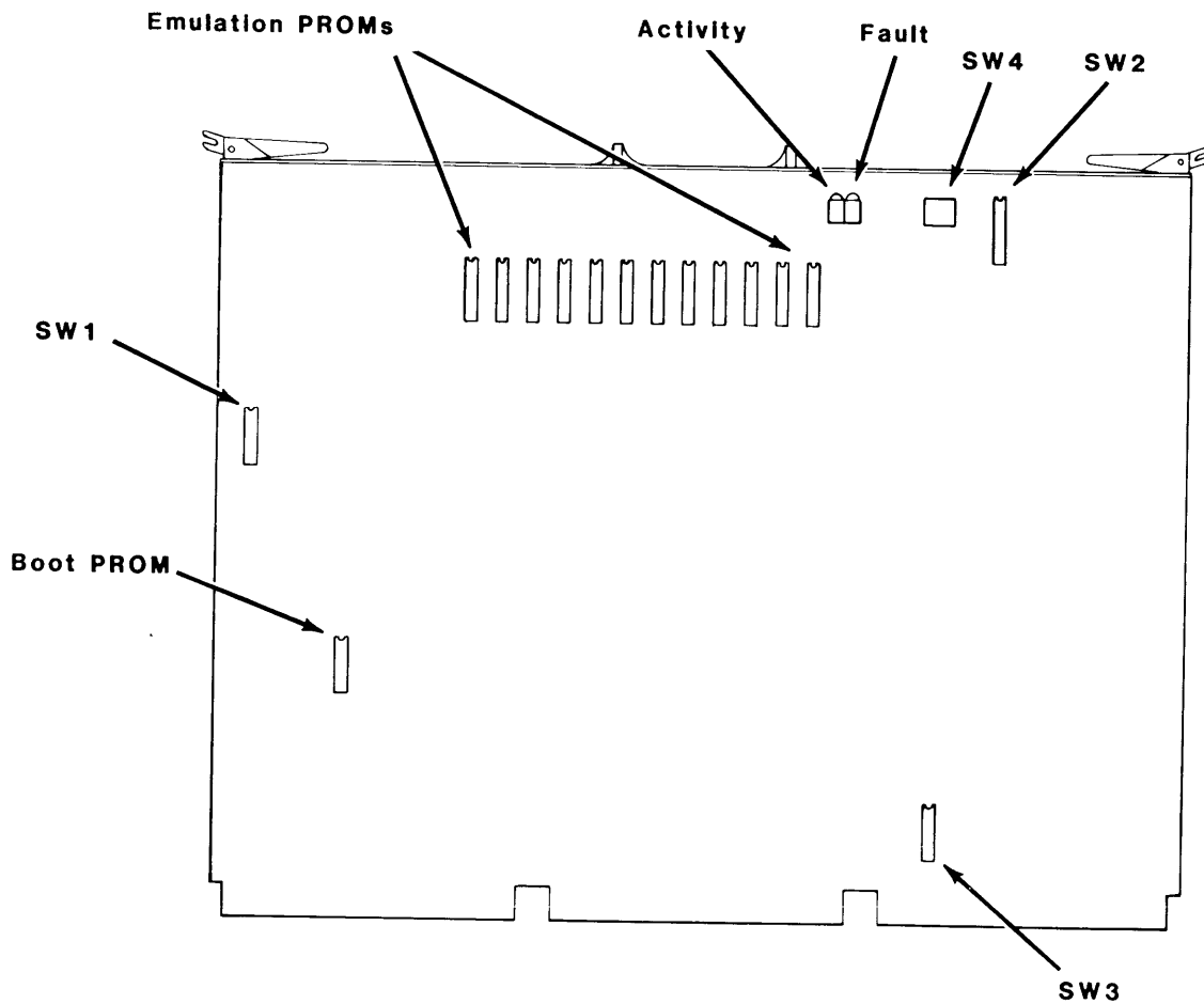
Figure 3-5 SC780 Controller Assembly
