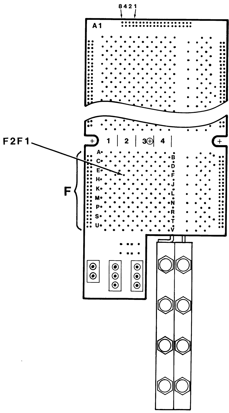
Figure 3-3 RH780 Backplane
