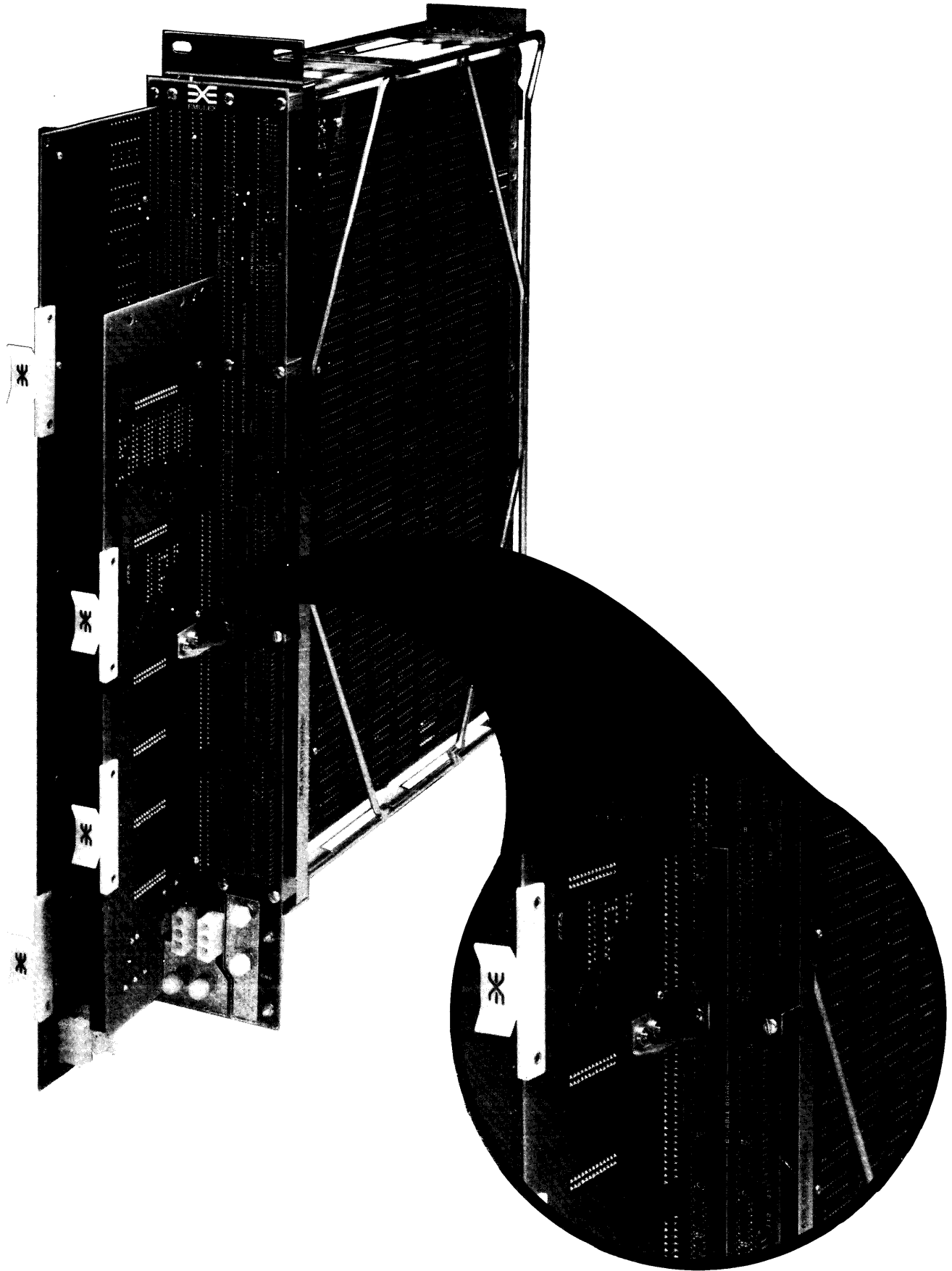
Figure 3-8 Paddle Board Mounting
