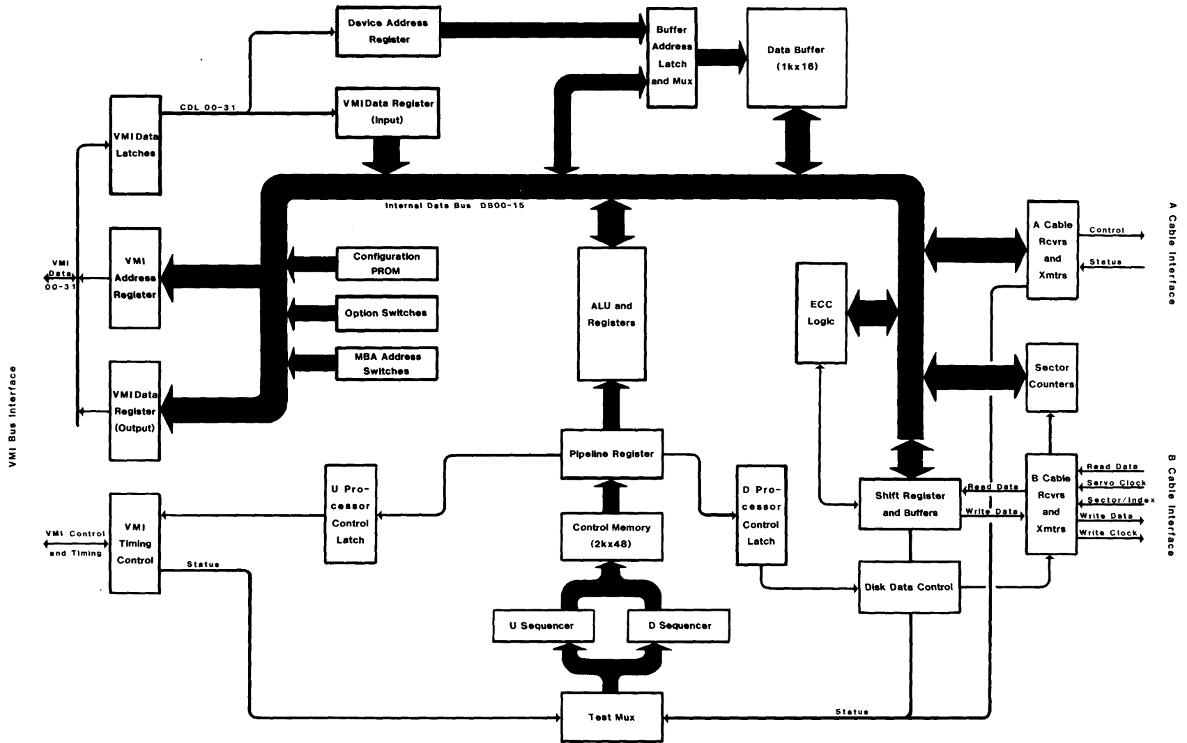
Figure 2-2 SC780 Block Diagram
