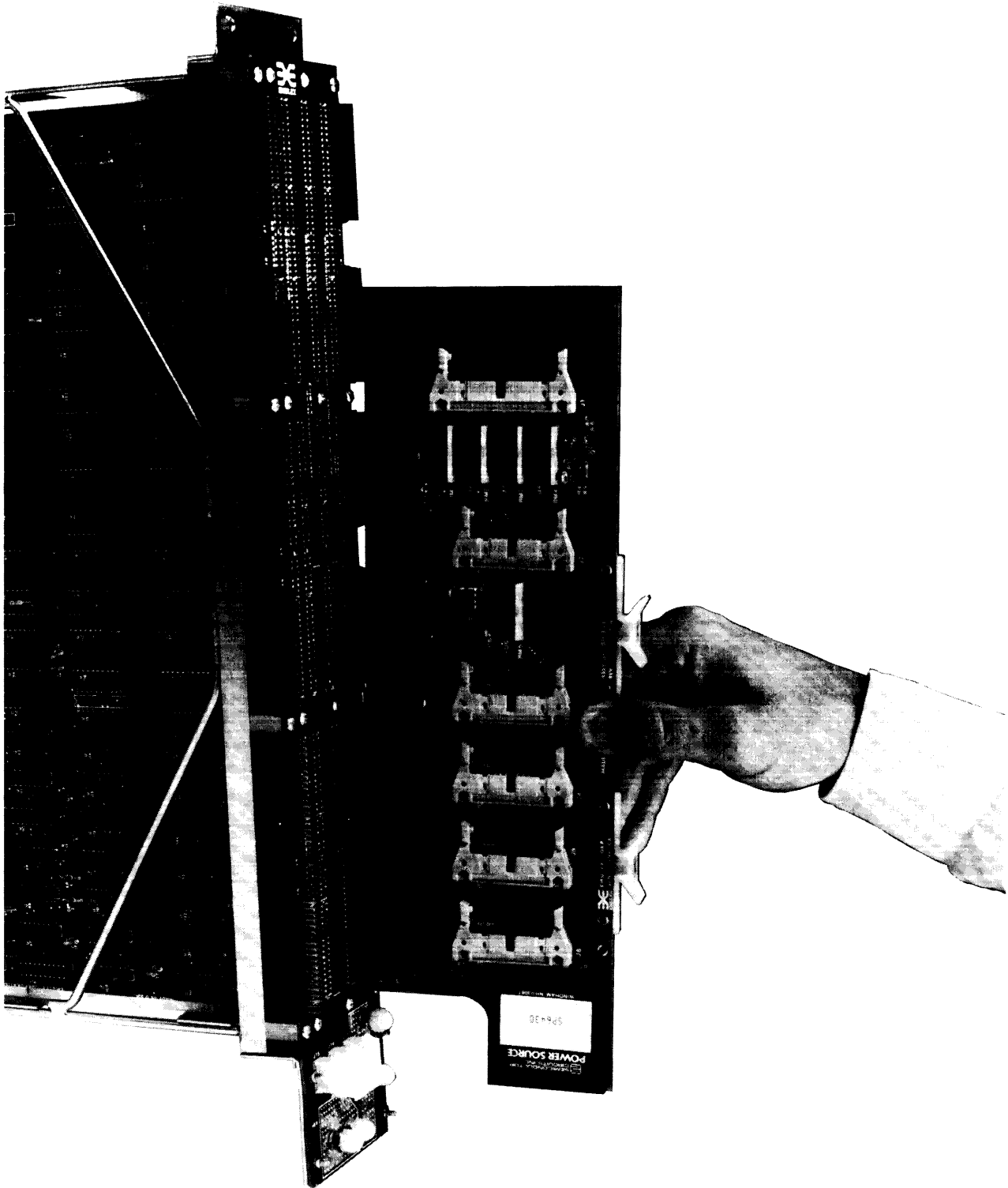
Figure 3-7 Paddle Board Installation
