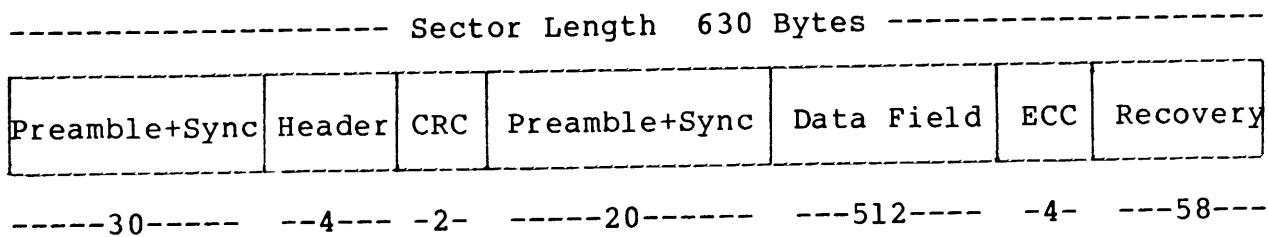
Figure 2-5 Sector Format
