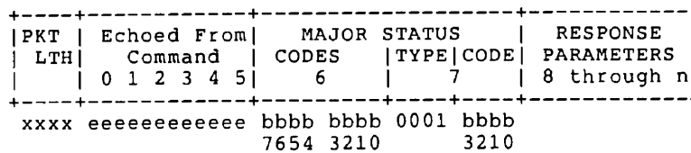
Figure 57 Response Packet for READ RAW DATA
