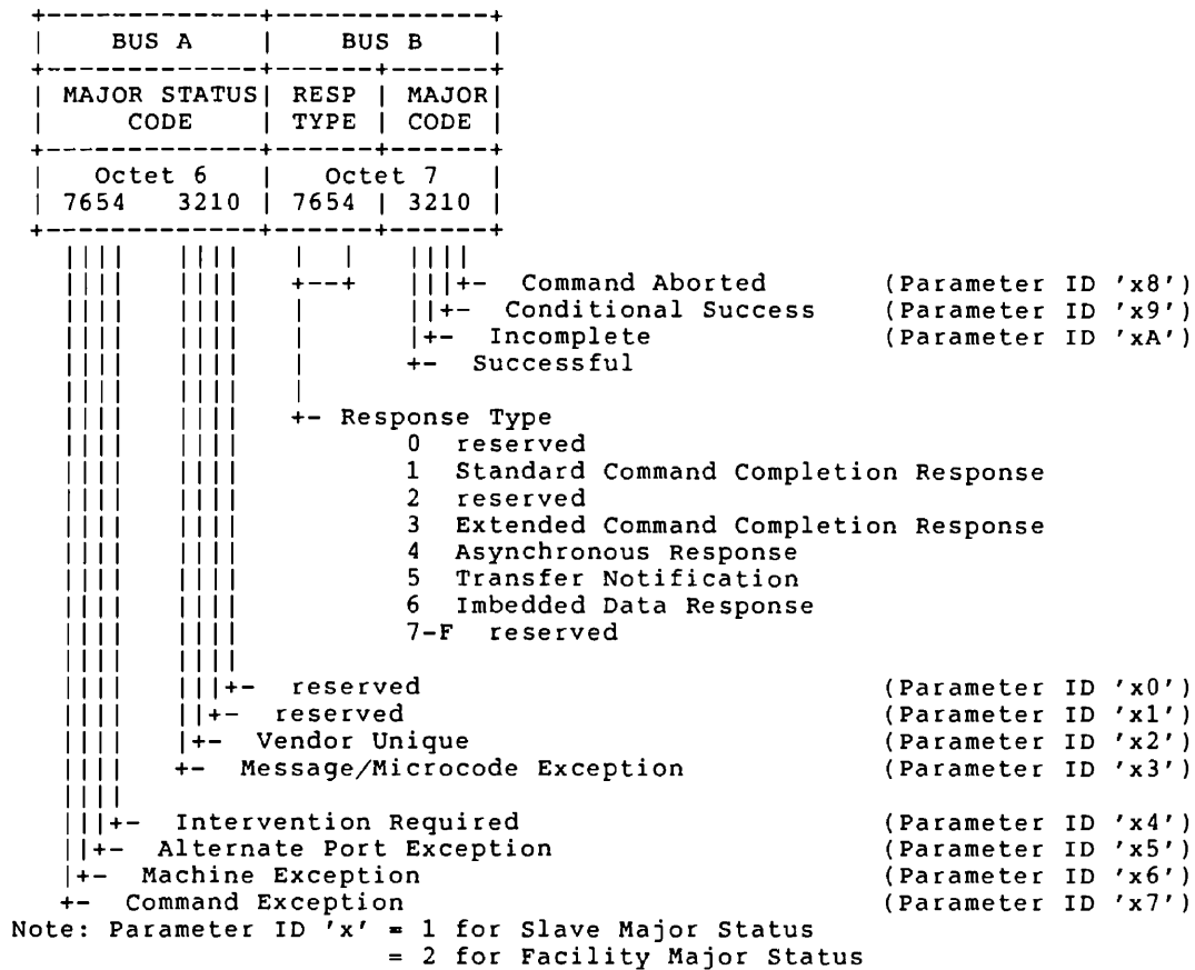
Figure 19 Types of Substatus and Responses
