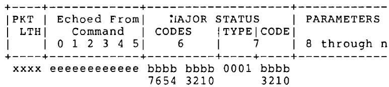
Figure 25 Response Packet for ATTRIBUTES
