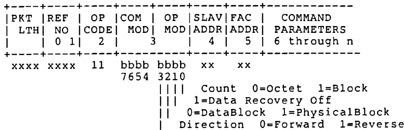
Figure 56 Command Packet for READ RAW DATA
