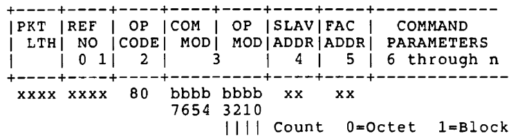
Figure 112 Command Packet for PERFORM SLAVE DIAGNOSTICS
