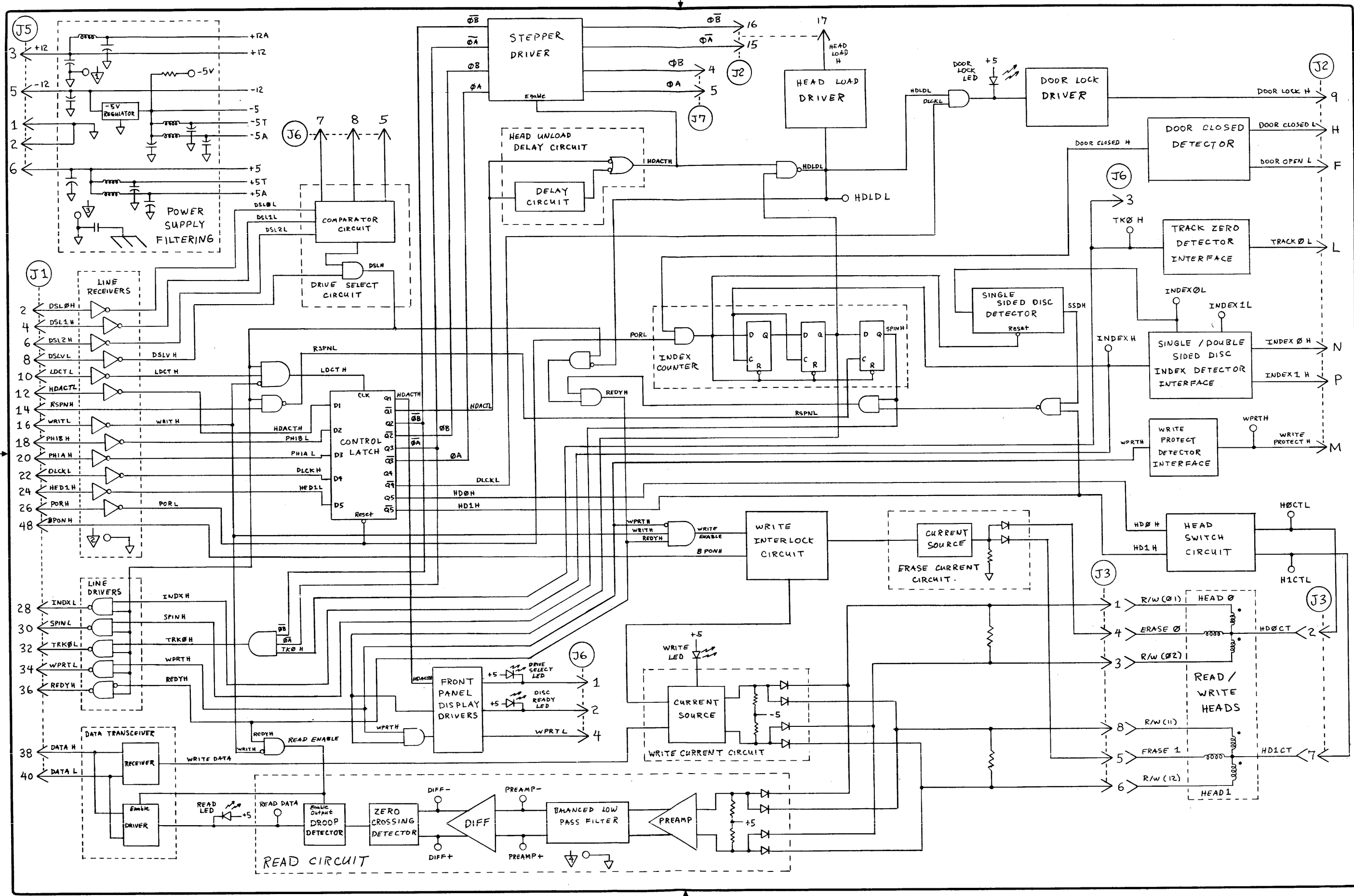
Figure 6-2. Drive PCA-A2 (07902-60023) Detailed Functional Block Diagram
