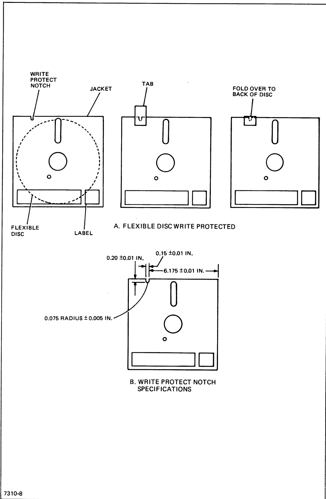
Figure 3-2. Write Protect Details
