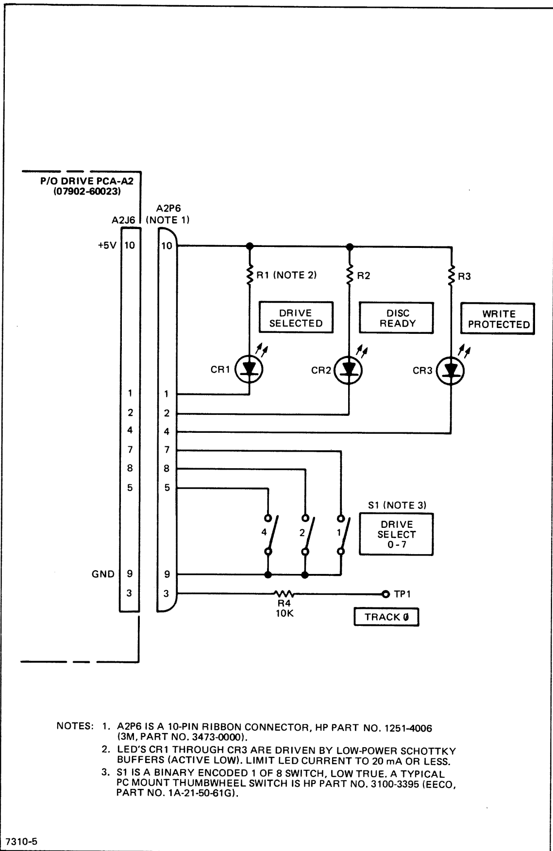
Figure 2-5. Typical Front Panel Indicator Display
