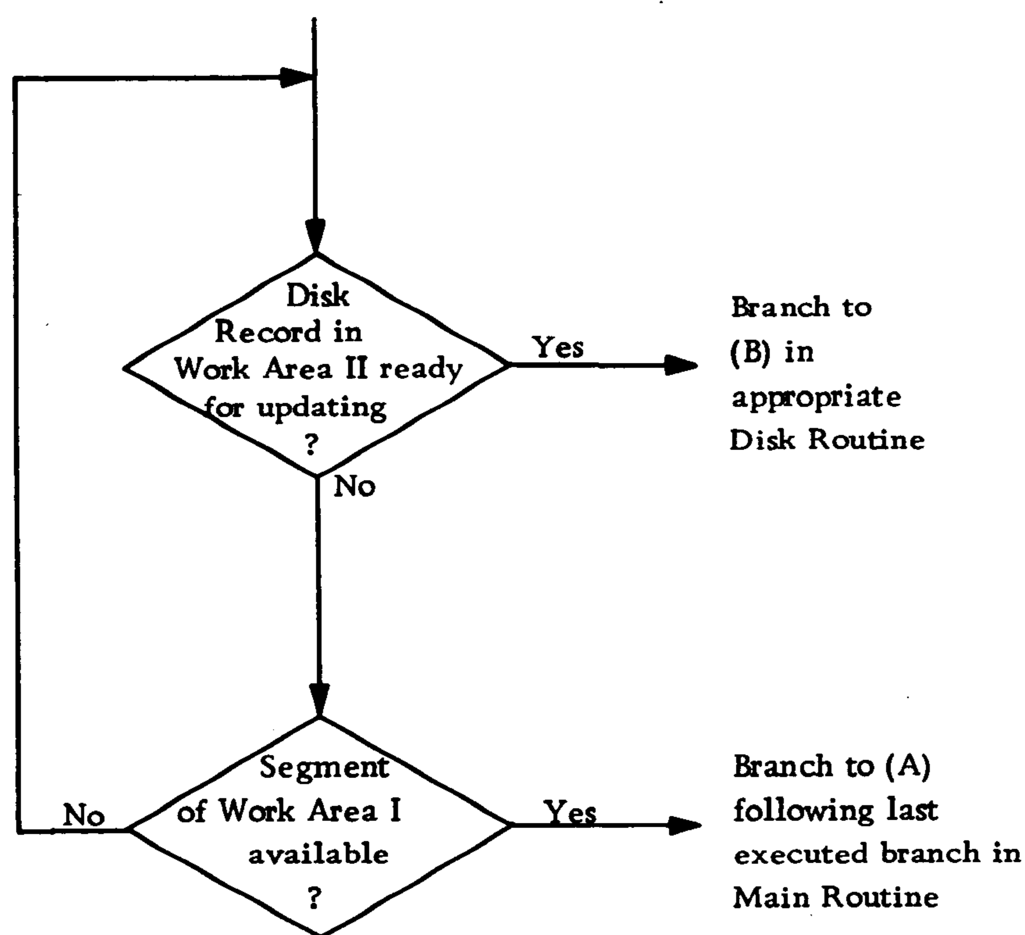
Figure 5. Control Switching
