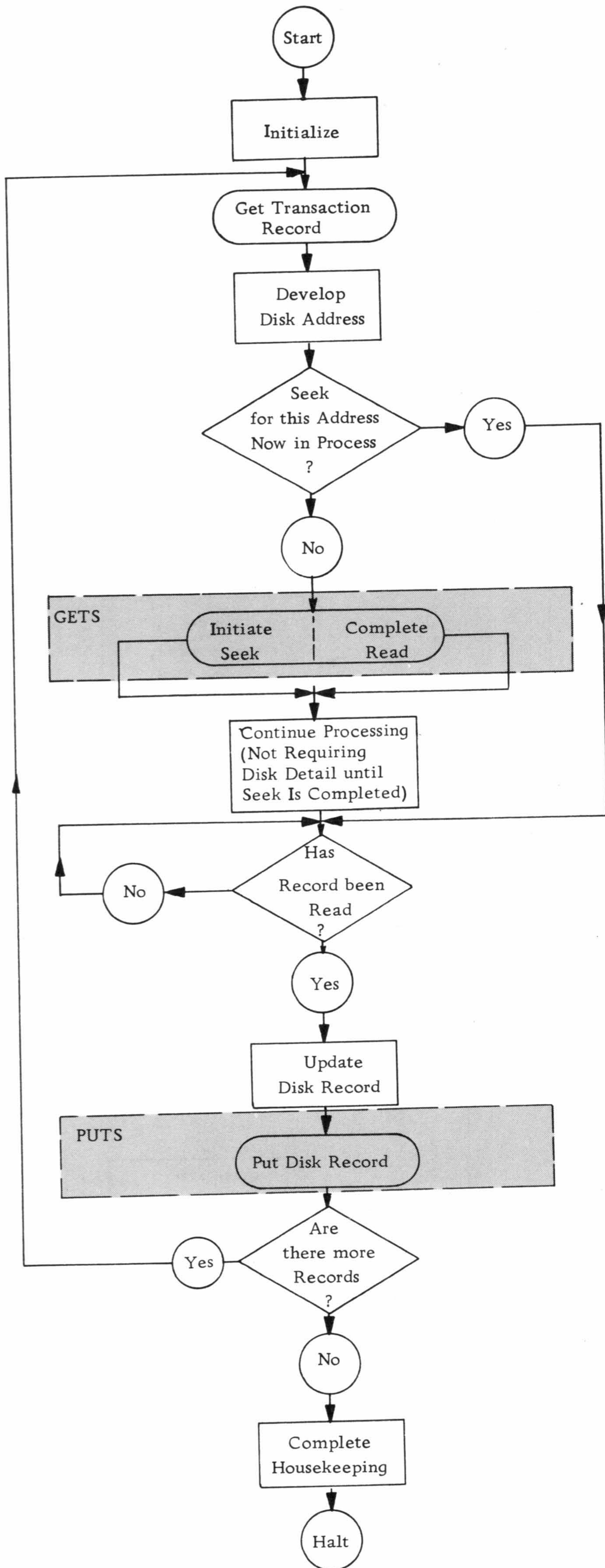
Figure 10. Method 2 of Single-Reference Processing
