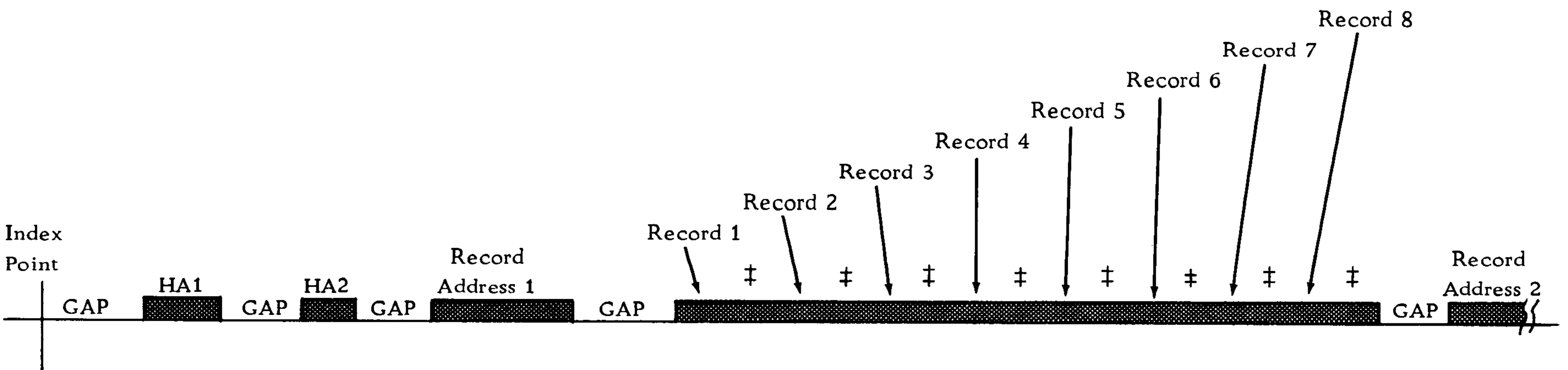
Figure 74. Disk Track with Form-2 Records
