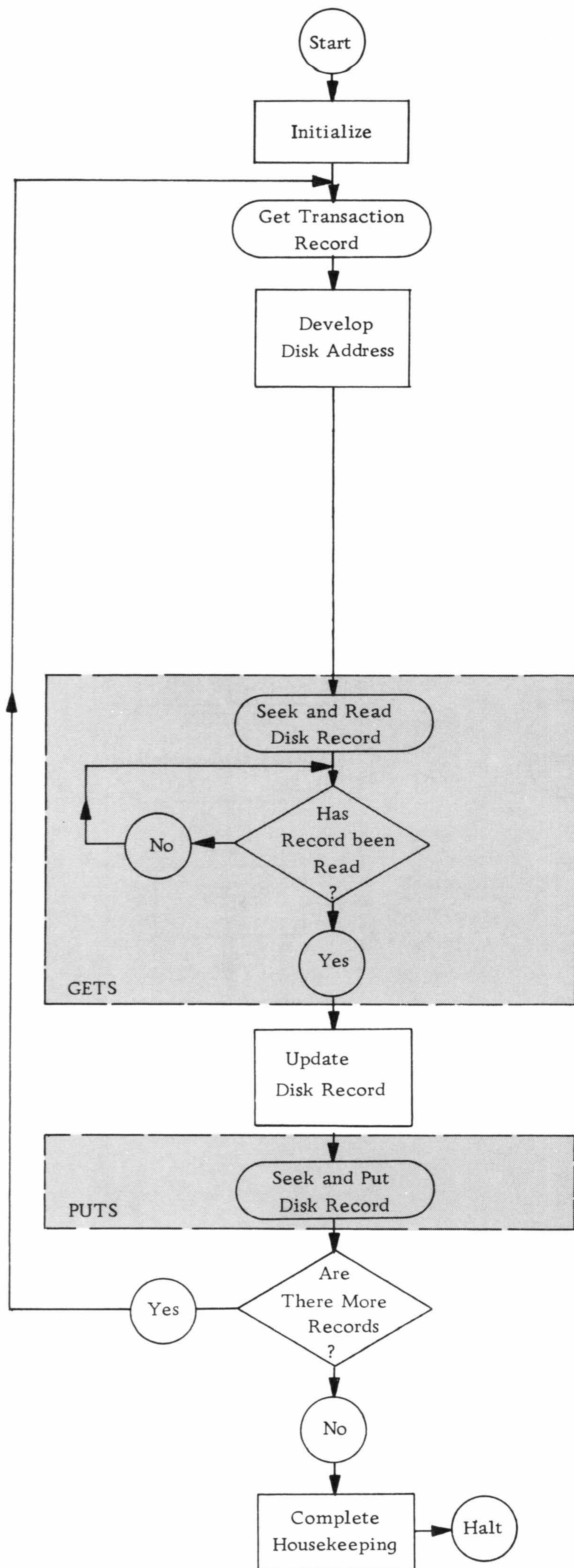
Figure 9. Method 1 of Single-Reference Processing
