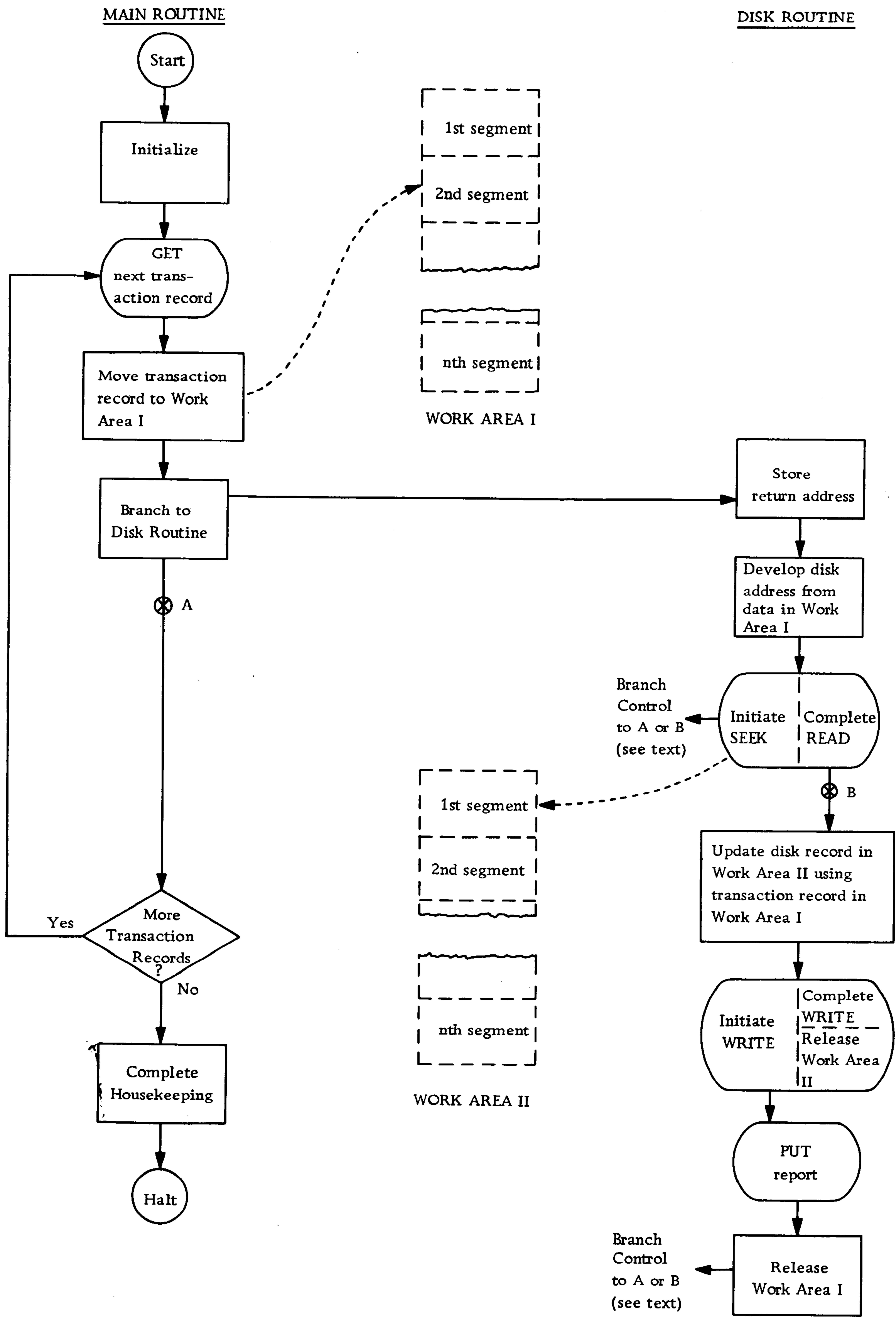
Figure 4. Separation of the Disk Routine from the Main Routine
