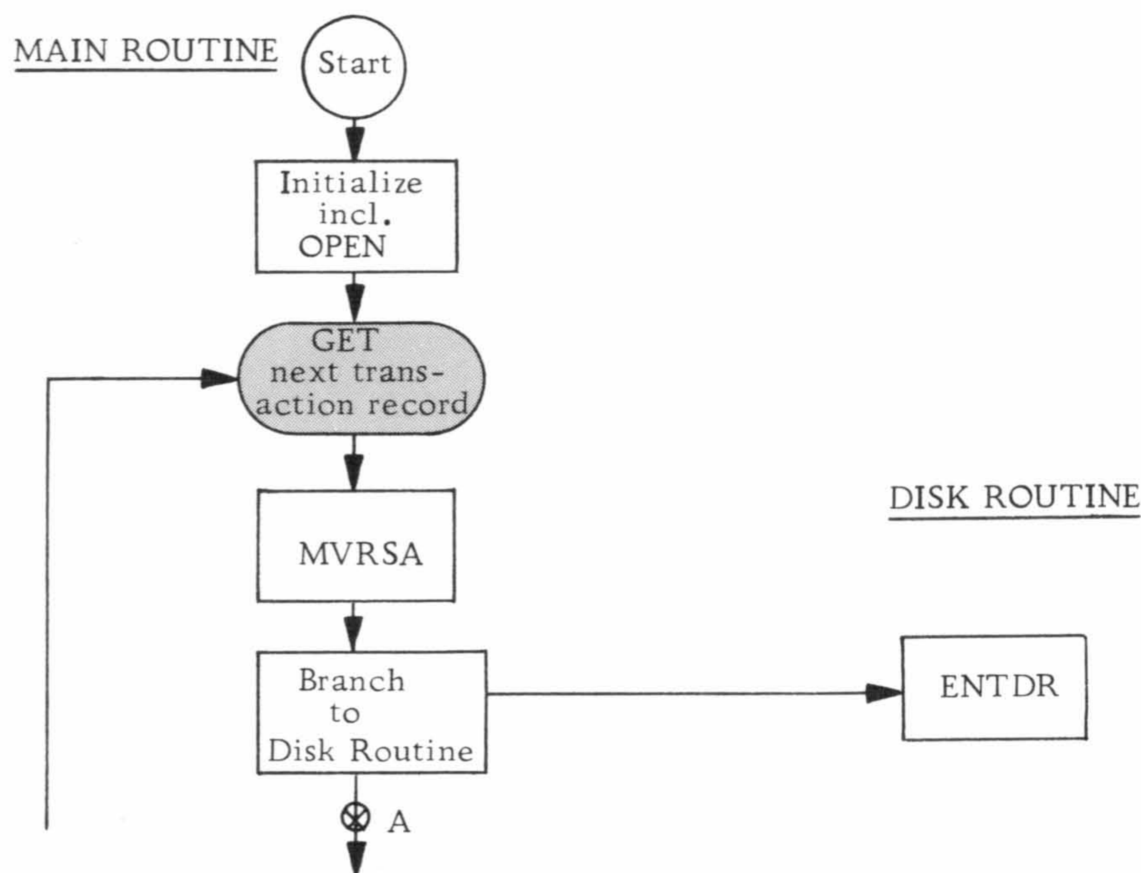
Figure 17. Use of the MVRSA Macro-Instruction
