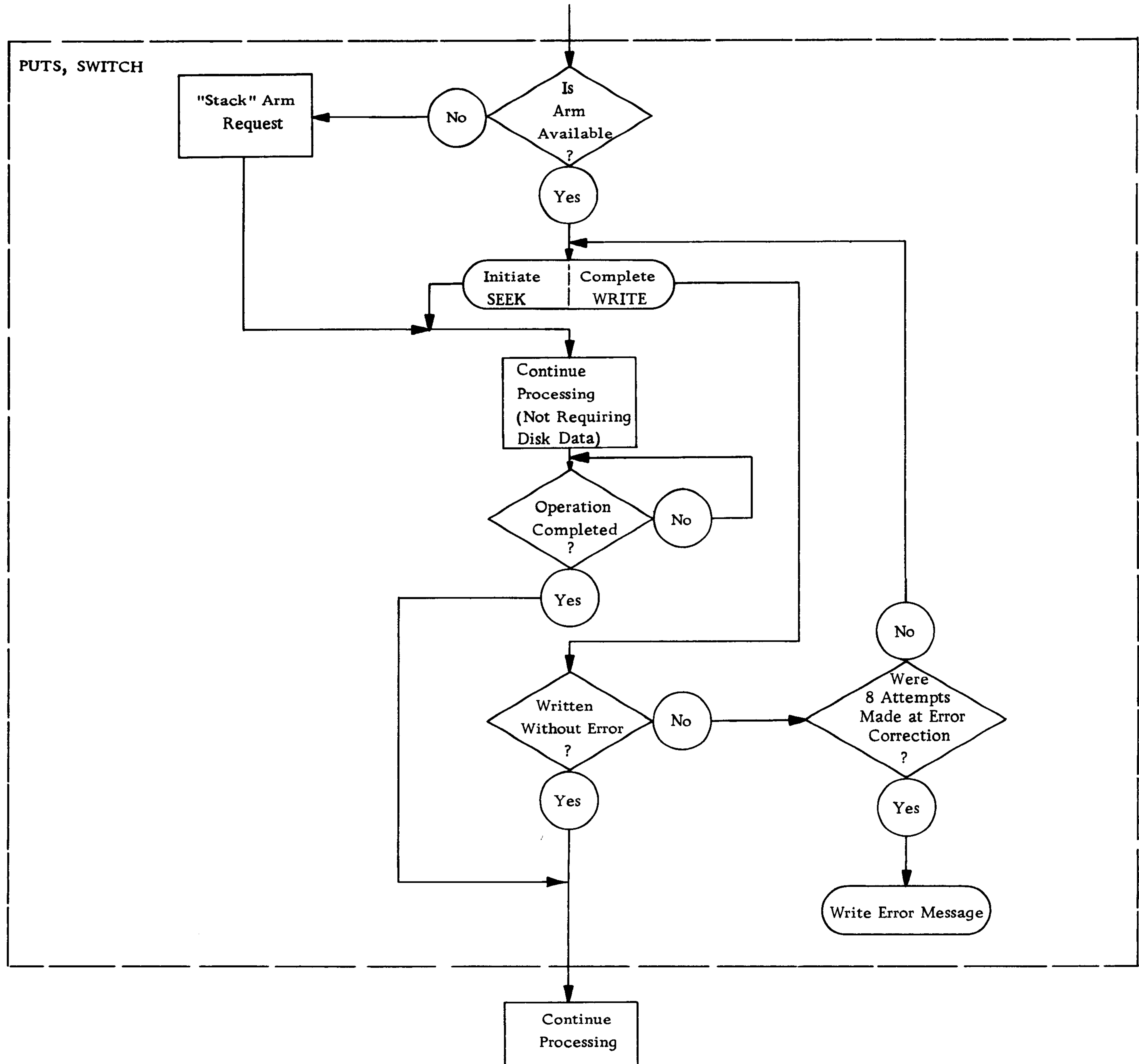
Figure 49. THE PUTS, SWITCH Macro-Instruction
