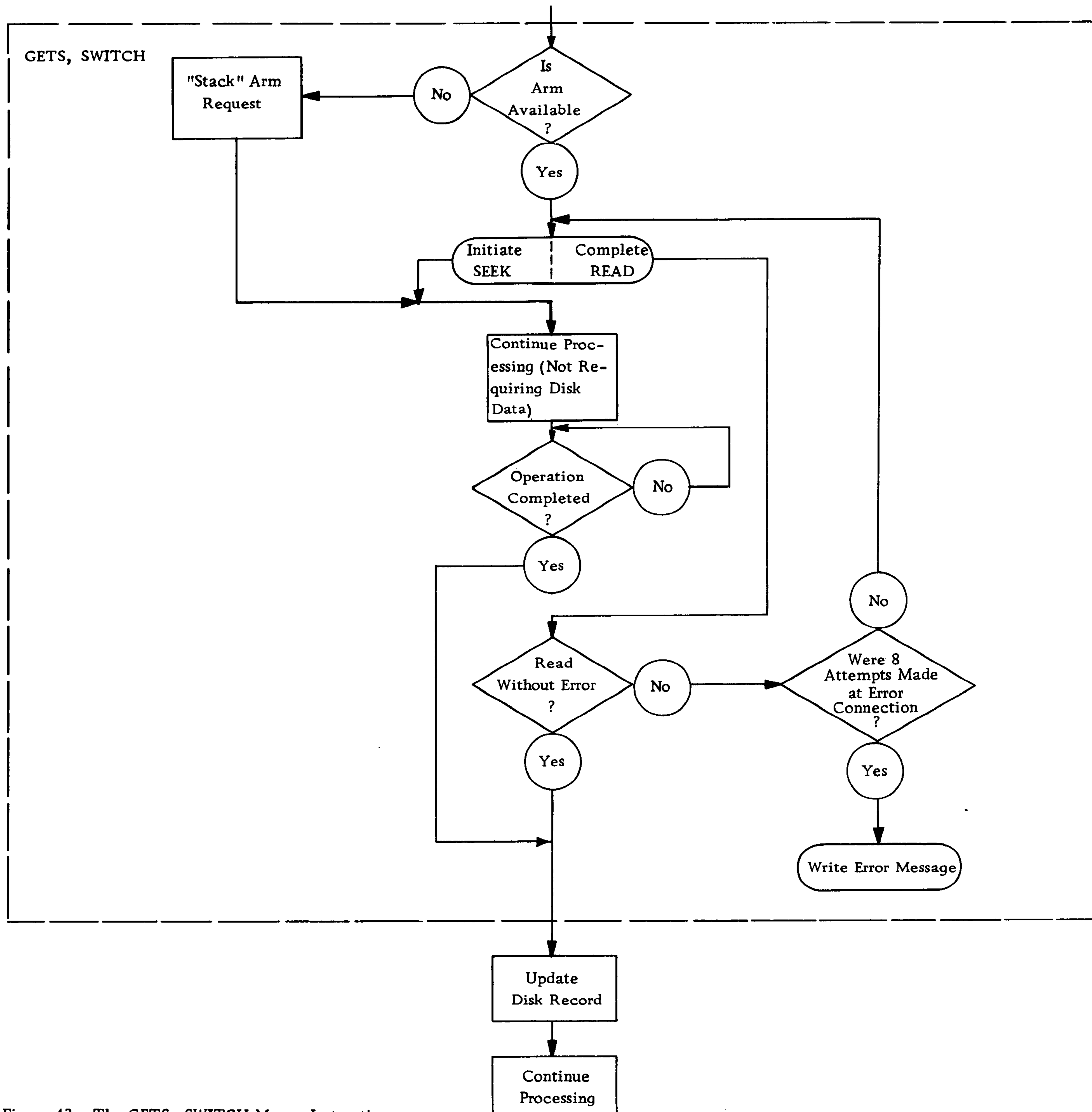
Figure 43. The GETS, SWITCH Macro-Instruction
