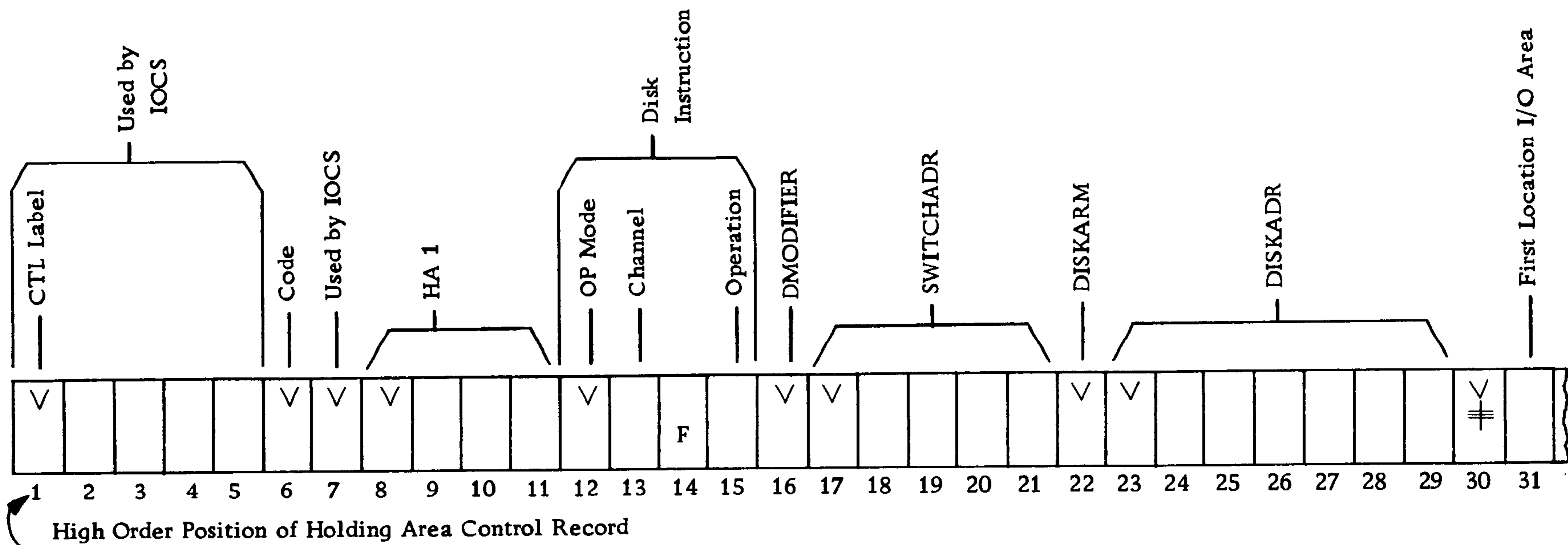
Figure 38. The Holding Area Control Record
