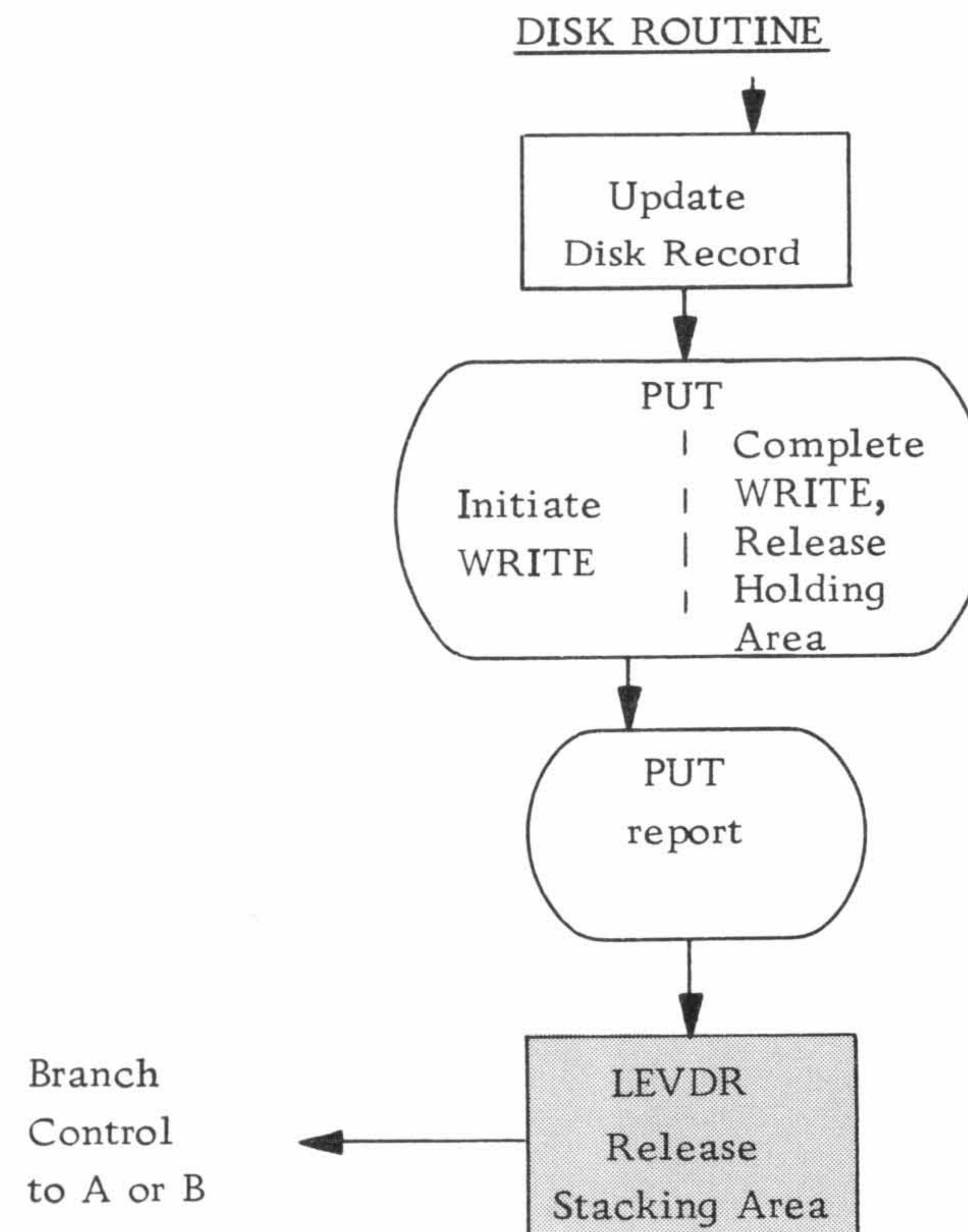
Figure 35. Use of the LEVDR Macro-Instruction
