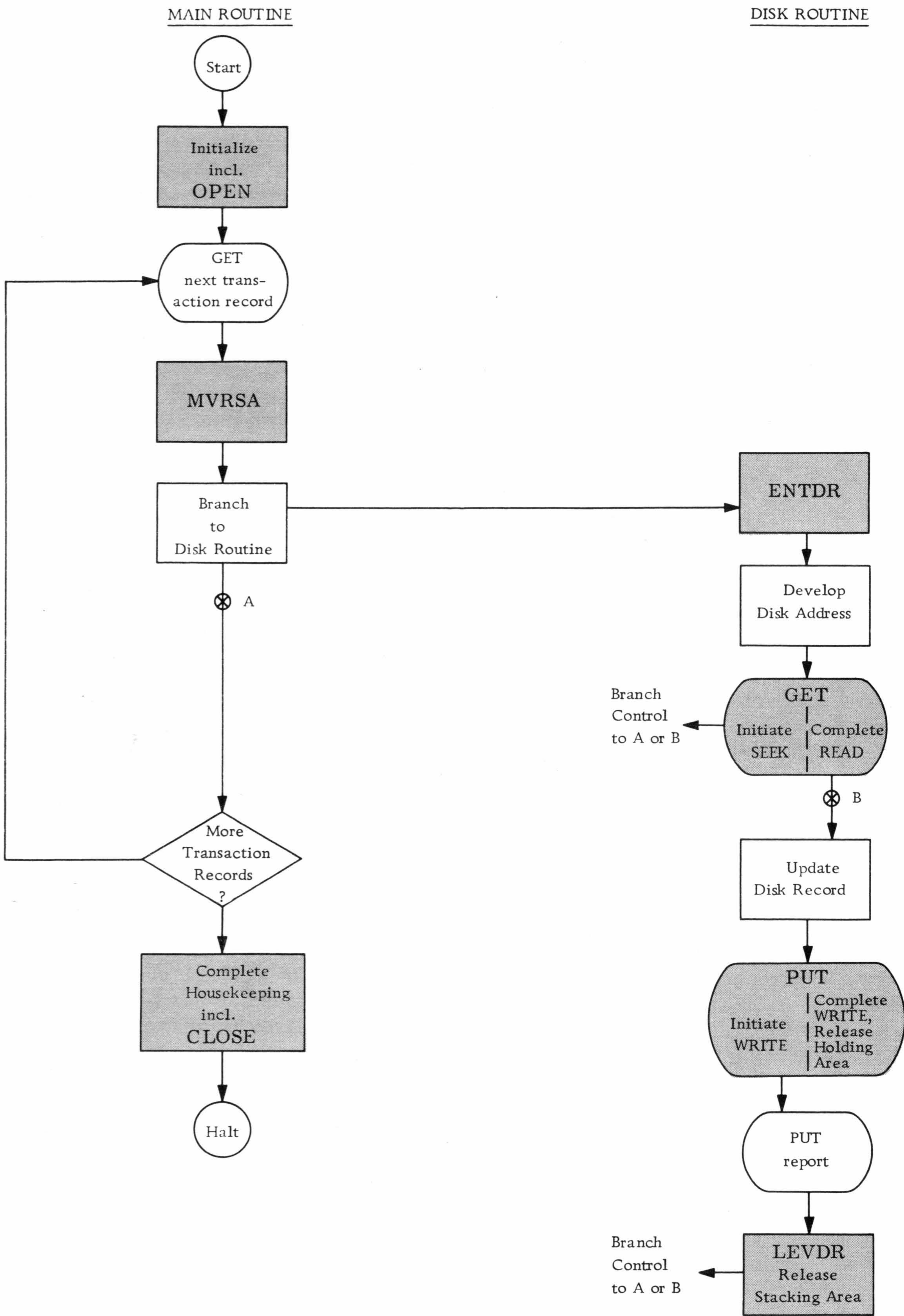
Figure 6. The 1301 IOCS Macro-Instructions for Random Processing
