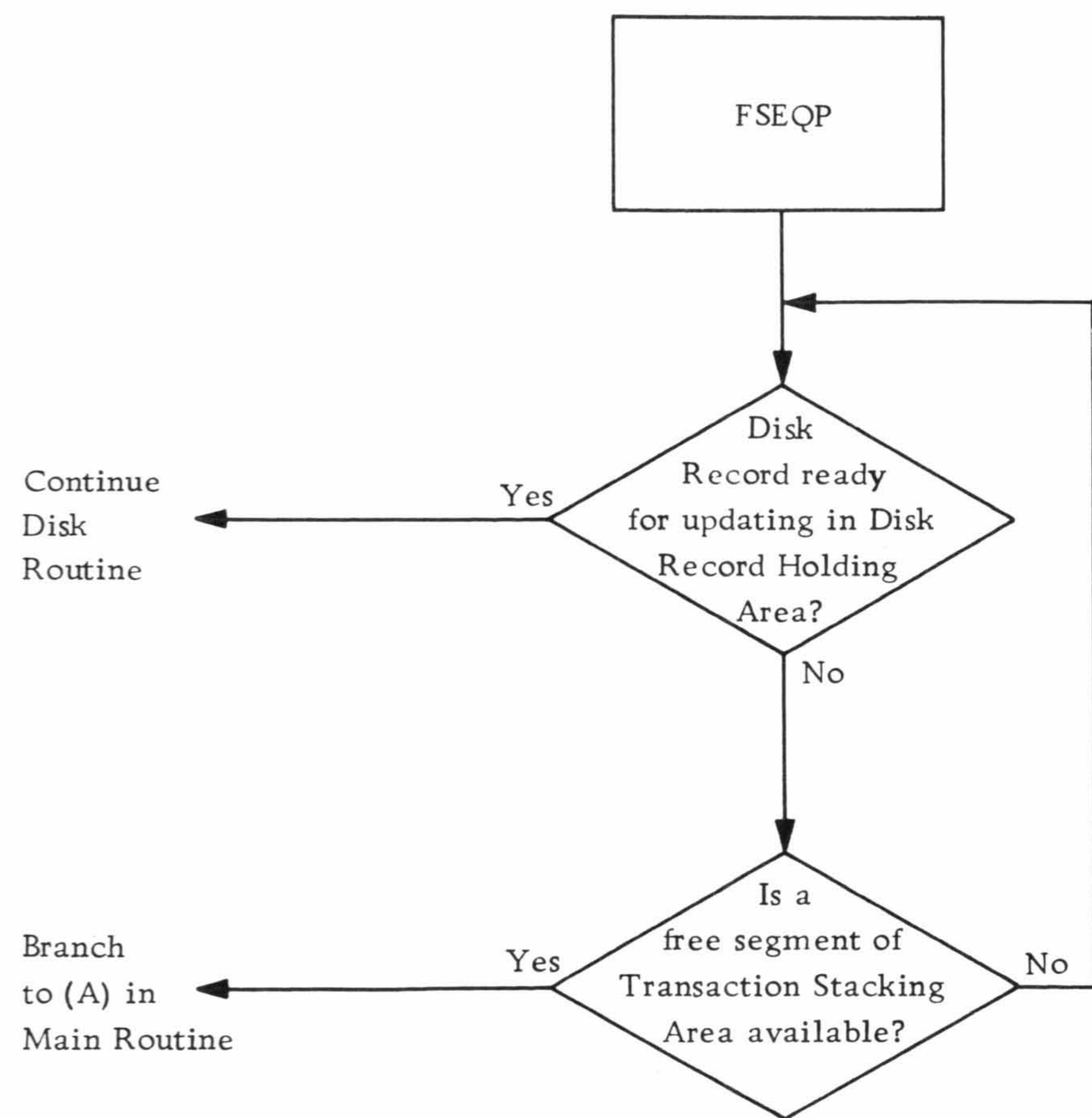
Figure 34. Control Functions of the FSEQP Macro-Instruction
