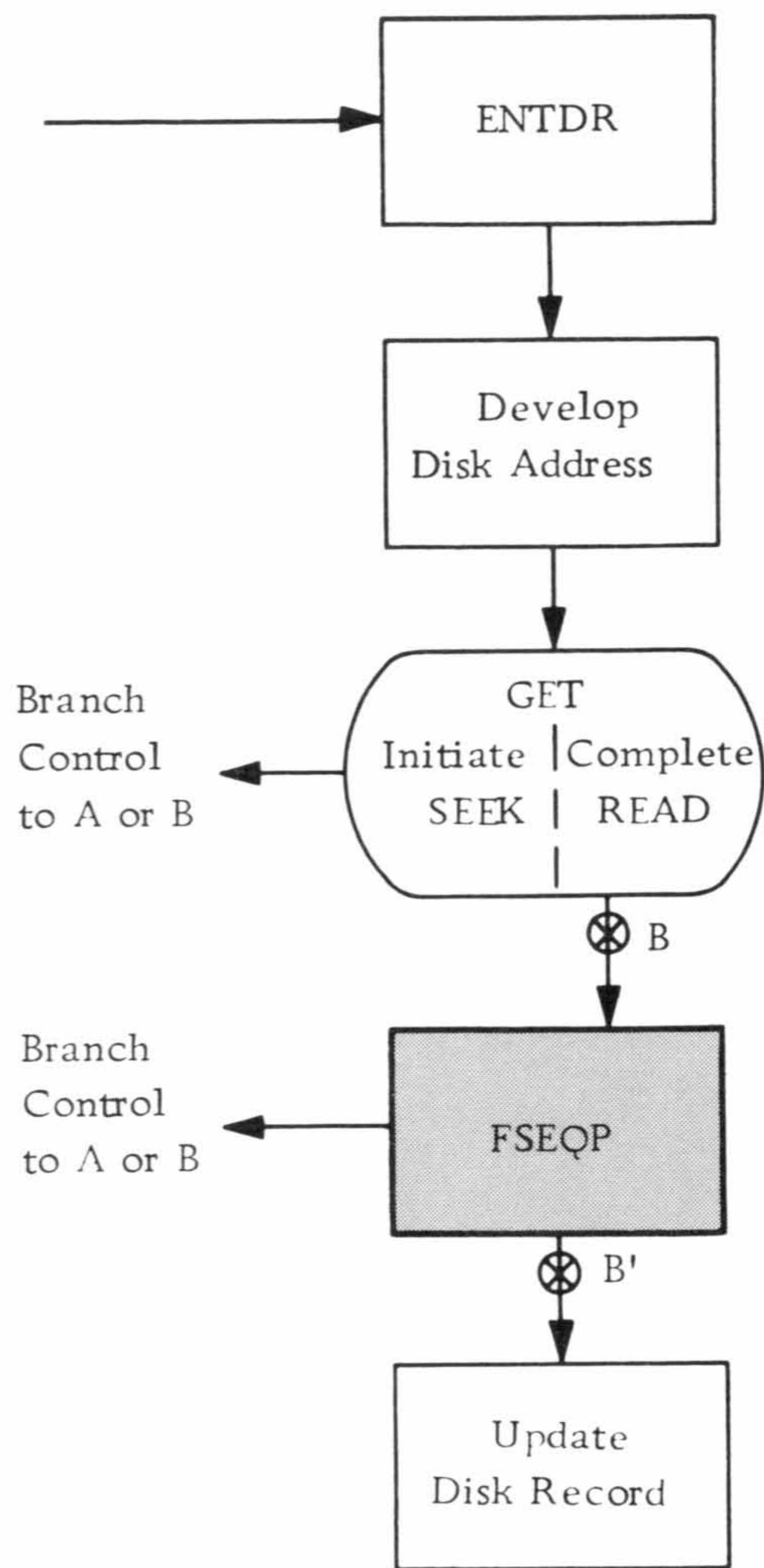
Figure 32. Use of the FSEQP Macro-Instruction
