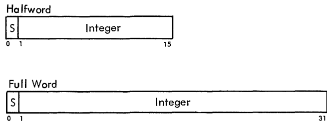
Figure 6. Fixed-Point Number Formats
