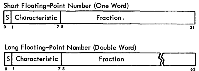
Figure 10. Short and Long Floating-Point Number Formats
