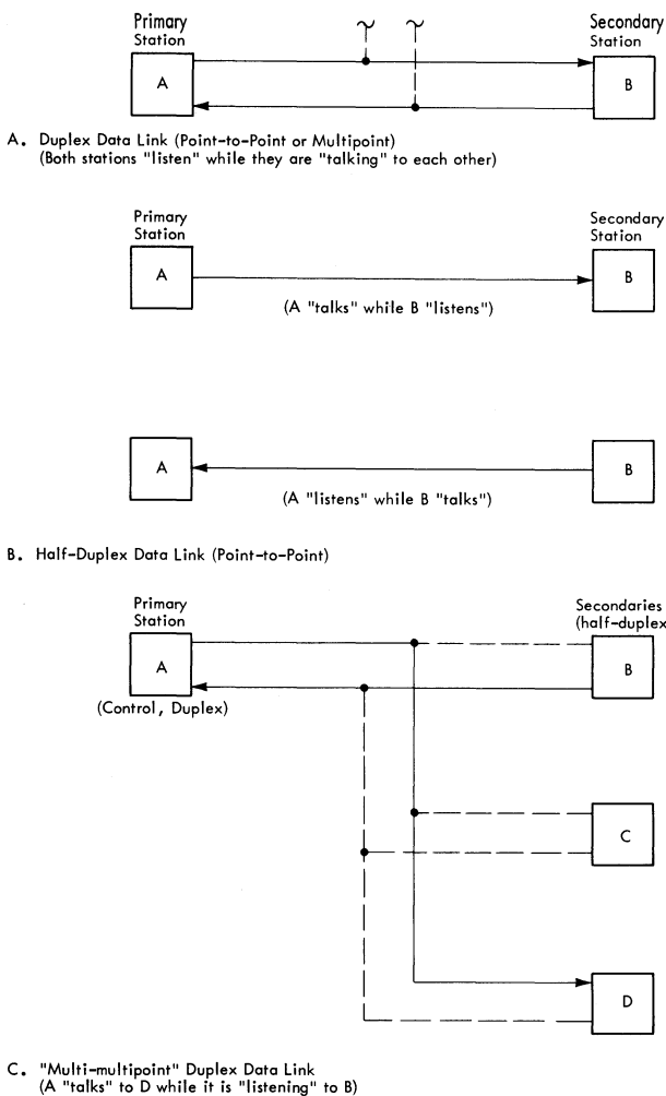
Figure 5-4. Data Link Configurations
