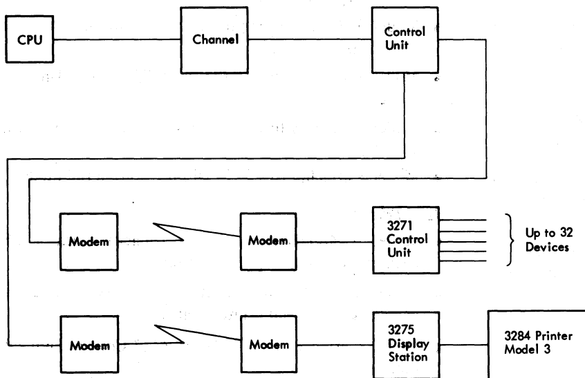
Figure 8-30. Information Path Comparison (Local and Remote) for IBM 3270 Information Display System
