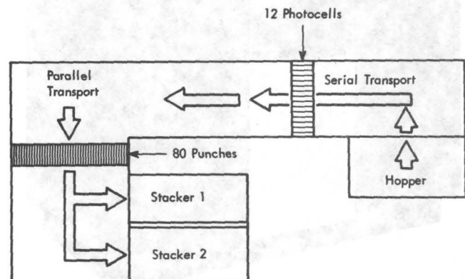
Figure 7-58. Card Path in IBM 2520 Card Read Punch Model B1
