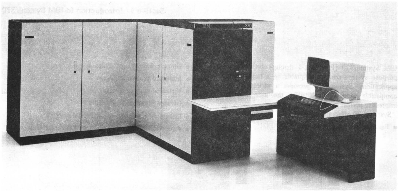
Figure 1-3. System/370 Model 158
