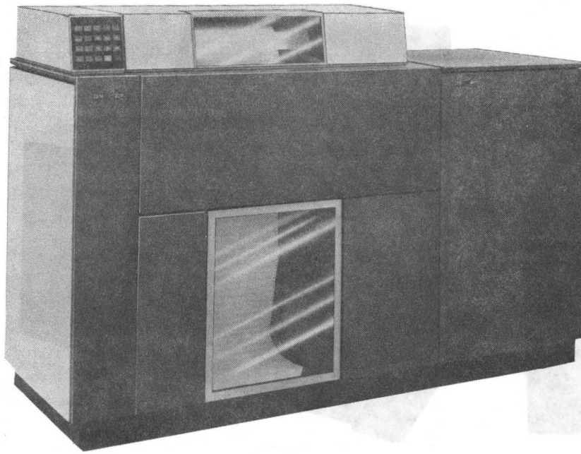
Figure 7-52. IBM 3211 Printer and IBM 3811 Control Unit
