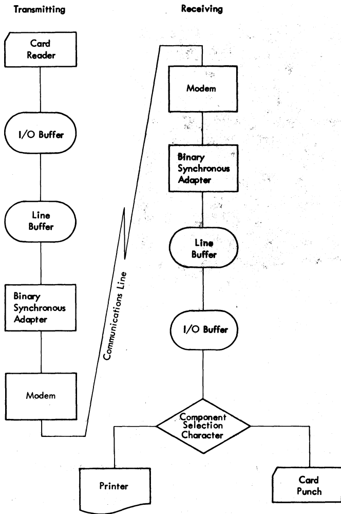
Figure 8-14. Data Flow, Terminal-to-Terminal Operation
