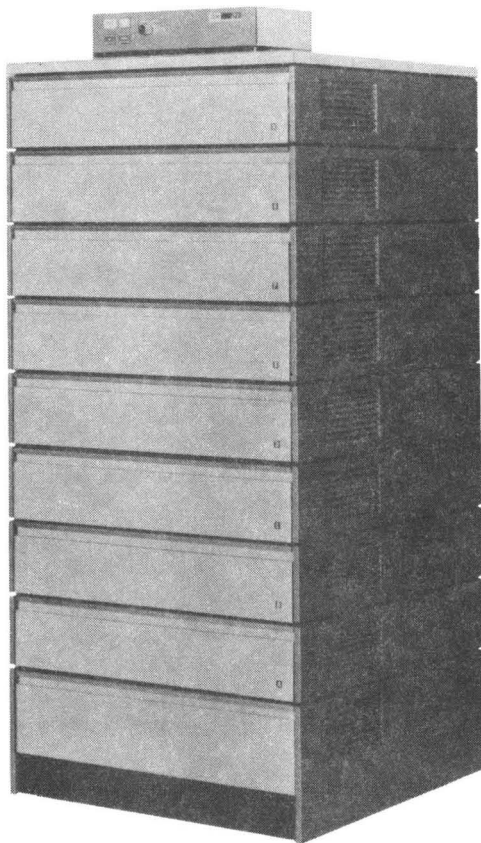
Figure 8-6. IBM 2711 Line Adapter Unit (with Maximum Number of Line Adapter Modules)
