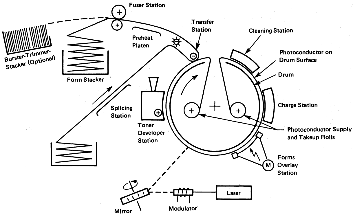
Figure 7-52.2. Path of Paper Forms through the IBM 3800 Printing Subsystem
