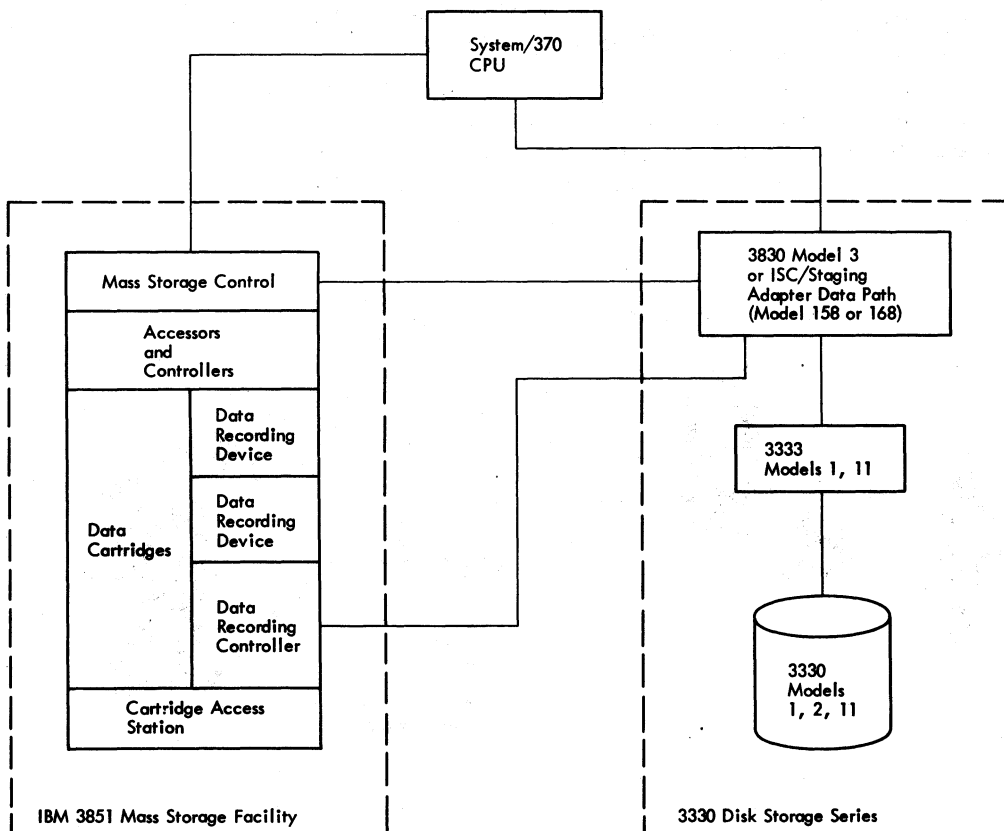
Figure 7-72. Logical Components of IBM 3850 Mass Storage System
