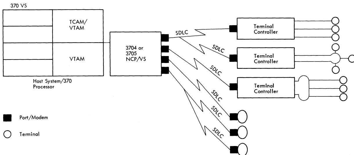
Figure 5-6. Systems Network Architecture
