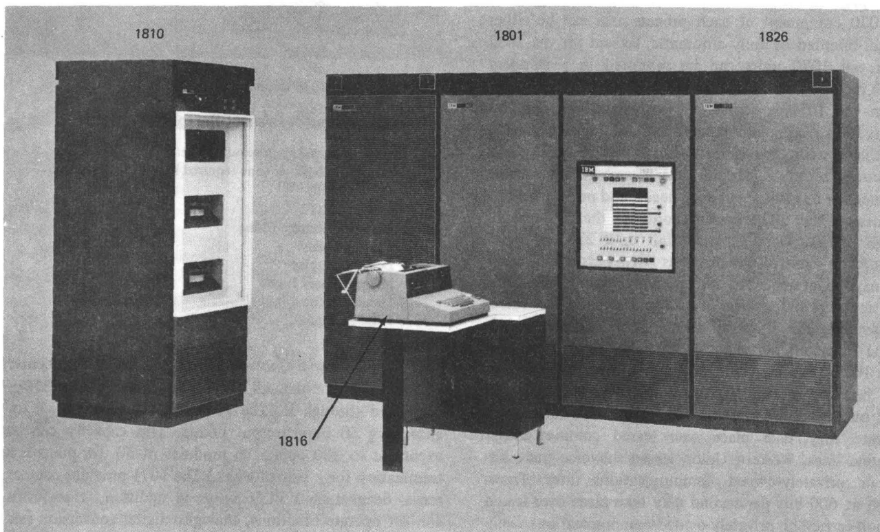
Figure 8-42. IBM 1800 Data Acquisition and Control System
