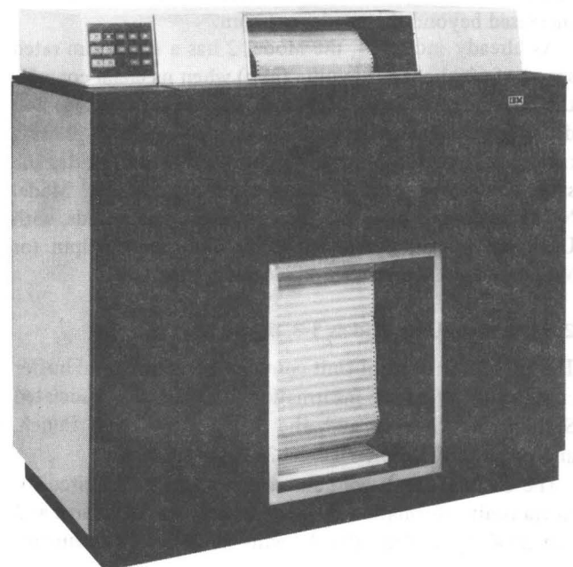
Figure 7-49. IBM 1403 Printer Model N1
