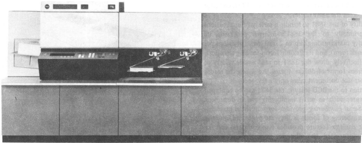
Figure 7-40. IBM 1288 Optical Page Reader
