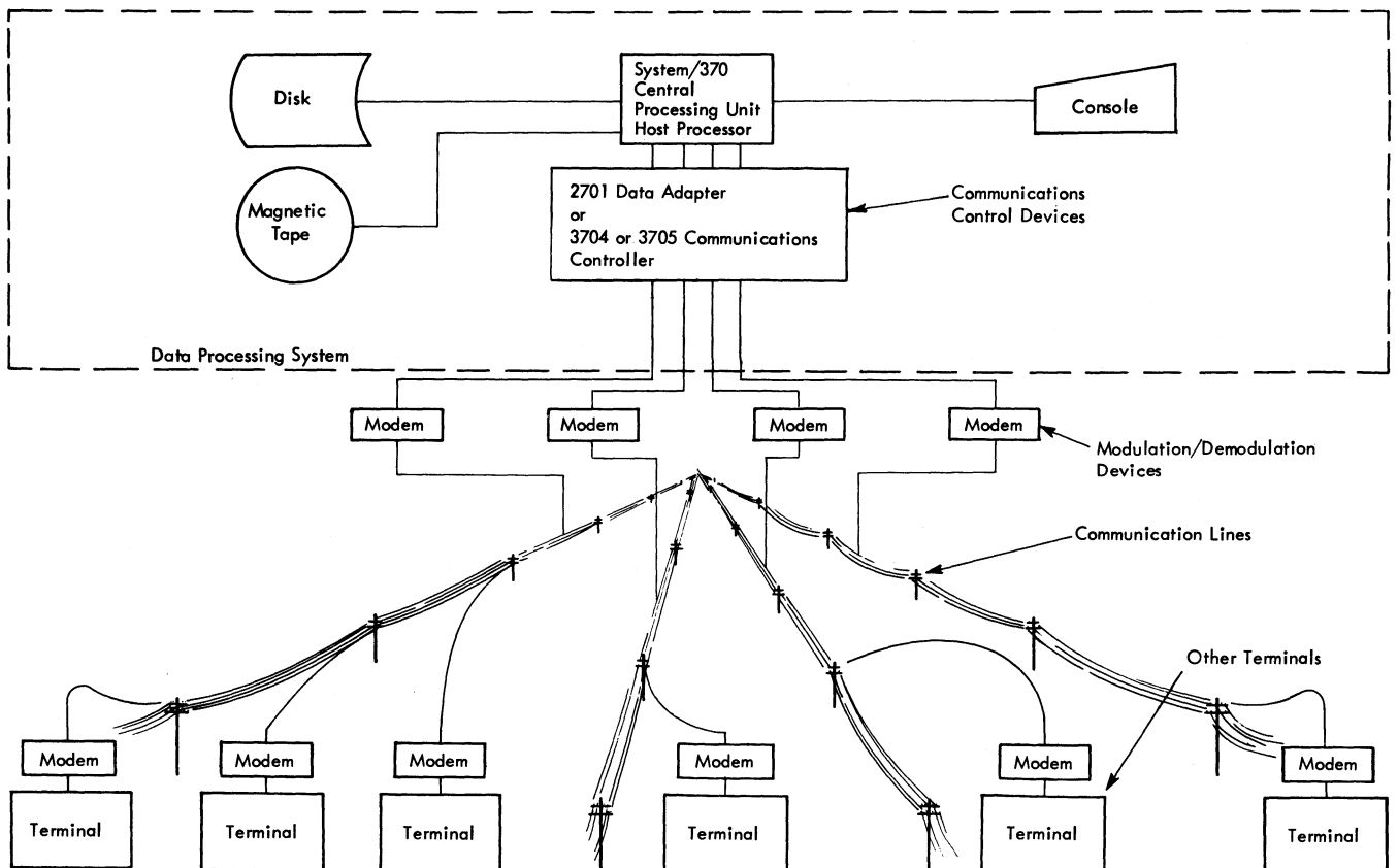
Figure 5-1. A Teleprocessing Network
