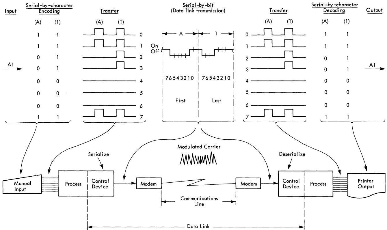
Figure 5-2. Data Conversion for Data Transmission
