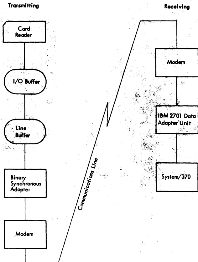
Figure 8-15. Data Flow, Terminal-to-Computer Operation
