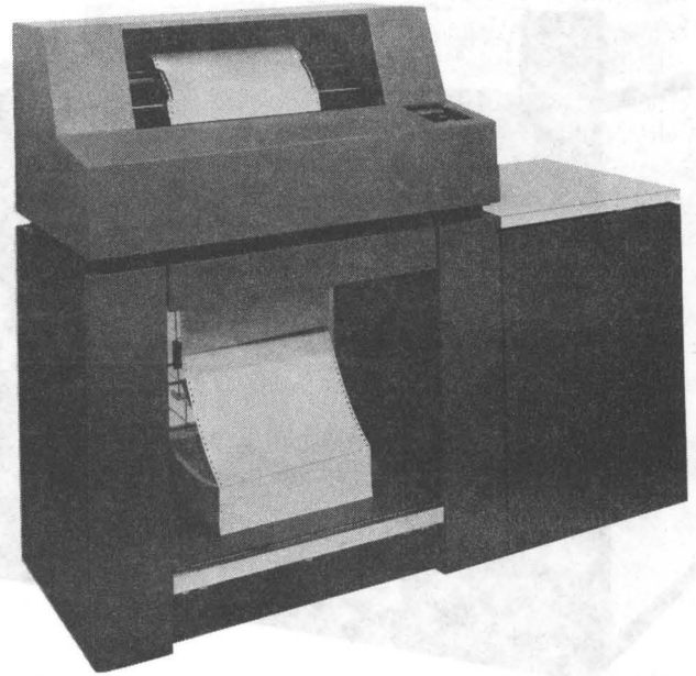
Figure 7-51. IBM 3203 Printer
