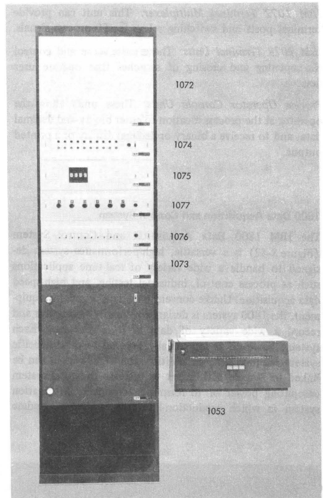
Figure 8-41. IBM 1070 Communication System
