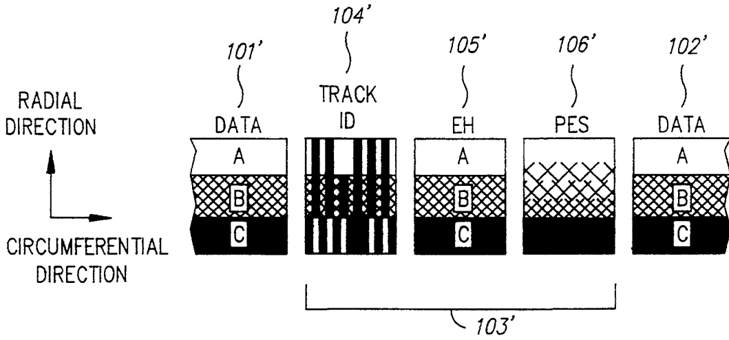
SECTOR SERVO HEAD POSITIONING INFORMATION WITH ERROR HANDLING
