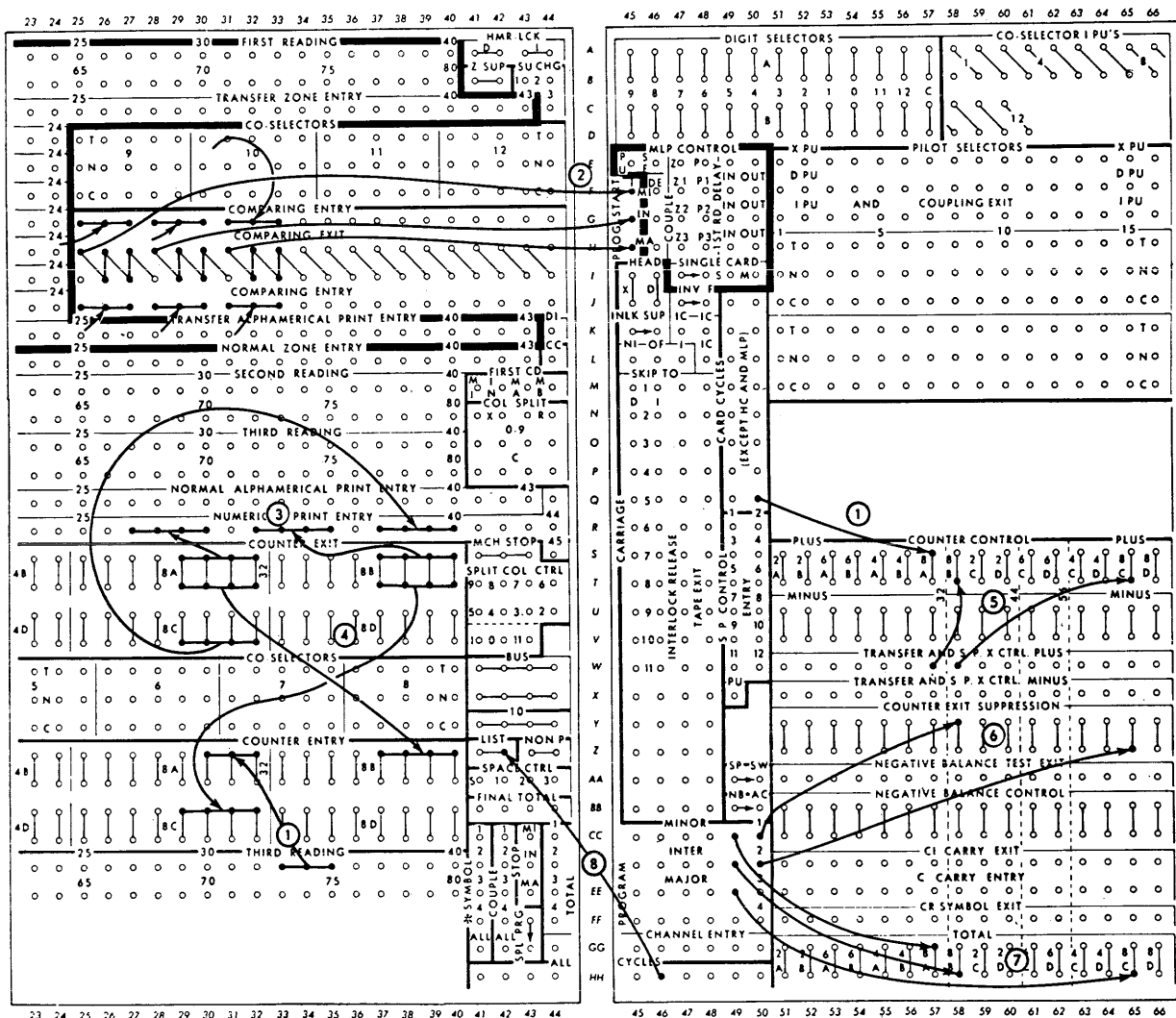
FIGURE 45. MINOR, INTERMEDIATE, MAJOR TOTALS — DIFFERENT TYPE BARS
