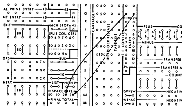
FIGURE 58. SPACE CONTROL
