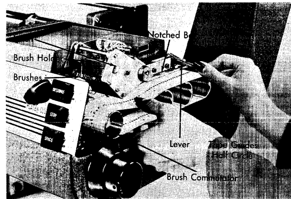
FIGURE 87. INSERTING TAPE IN CARRIAGE
