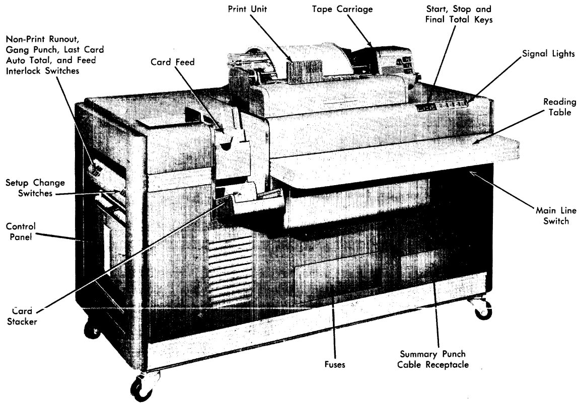
IBM ACCOUNTING MACHINE TYPE 402
