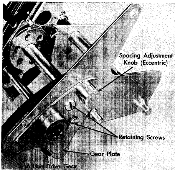
FIGURE 128. 6 OR 8 LINE DRIVE (MODEL F-3)
