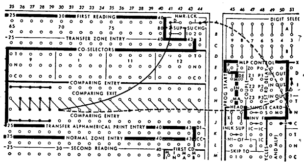
FIGURE 36. HAMMERLOCKING FROM COMPARING EXIT
