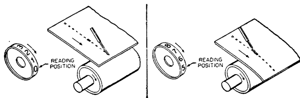
FIGURE 22. MOVEMENT OF COUNTER WHEEL WHEN SUBTRACTING
