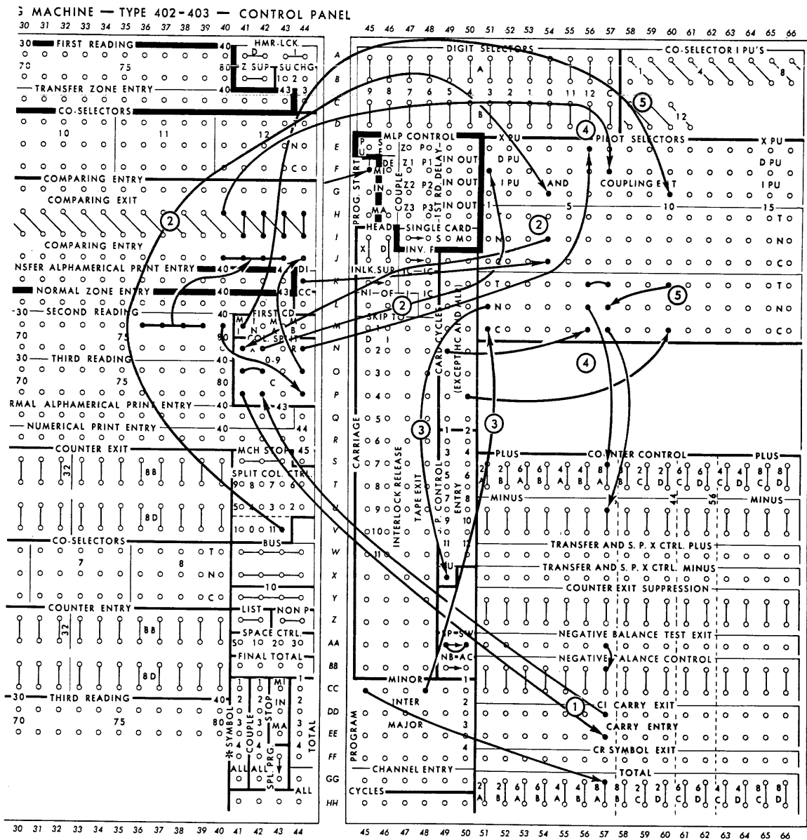
FIGURE 75. SUMMARY PUNCH ELIMINATION OF ZERO BALANCES
