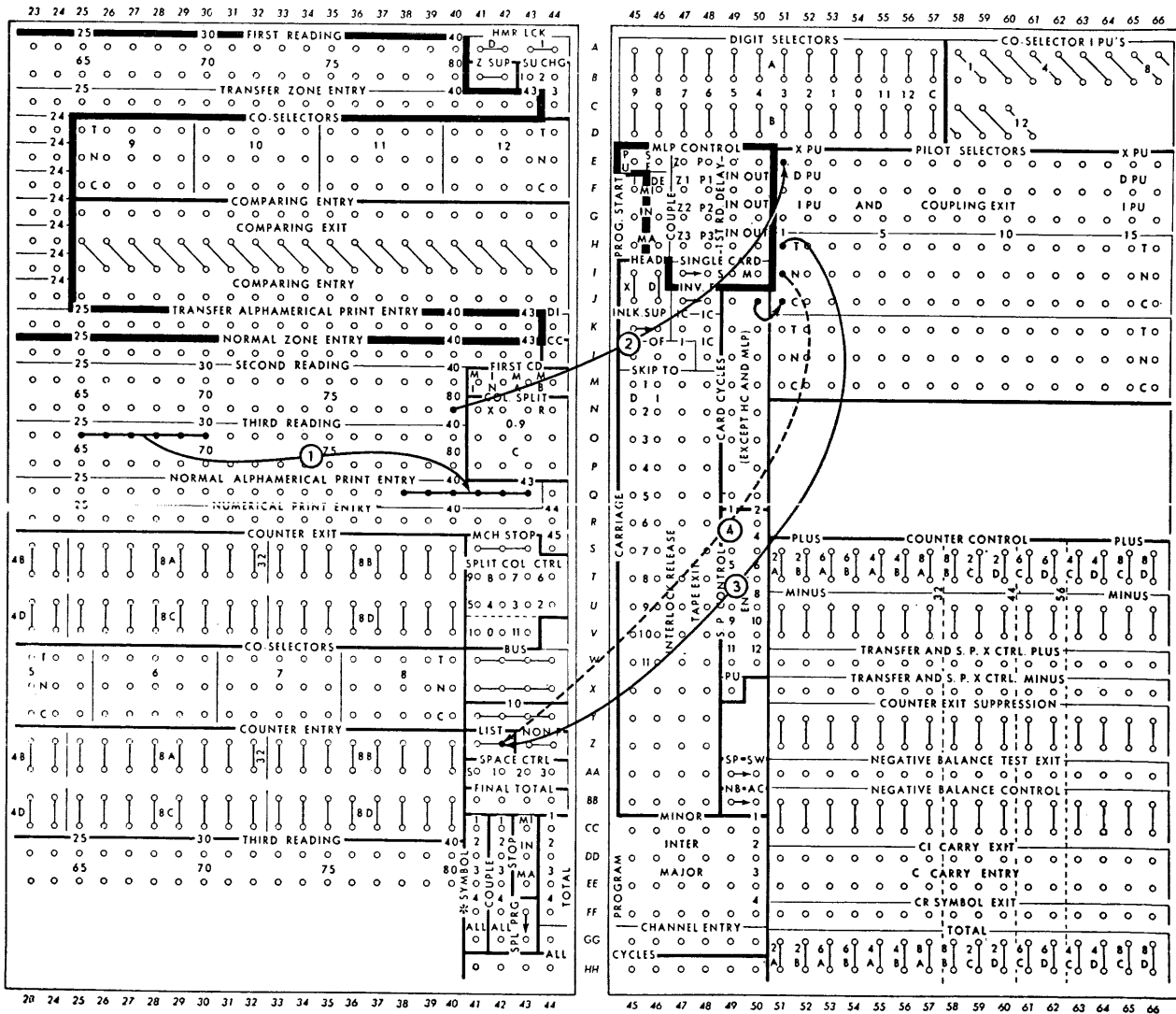
FIGURE 30. SELECTIVE PRINTING
