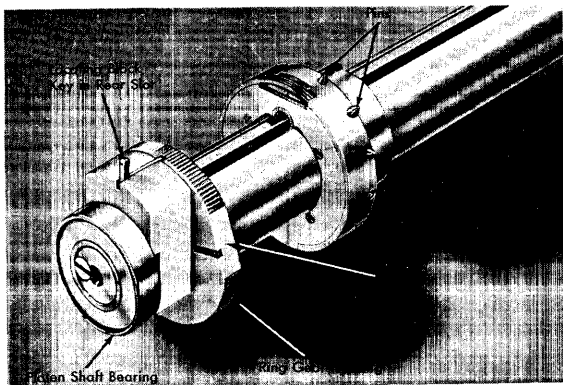
FIGURE 124. MODEL P-2 PINS IN THE OPERATING POSITION
