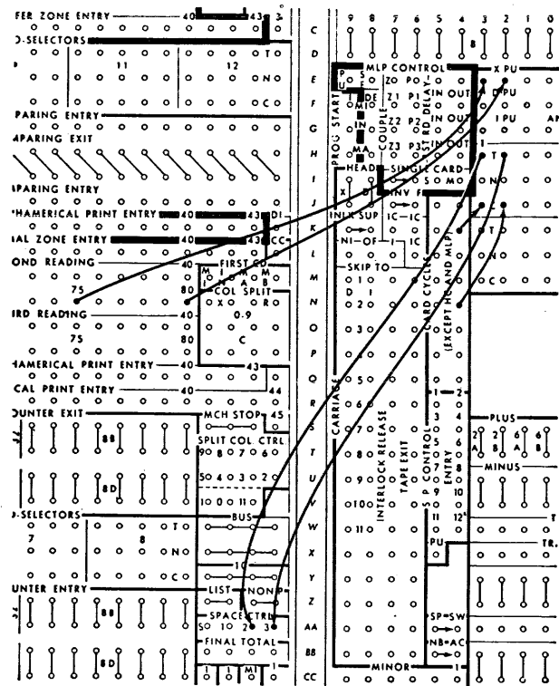
FIGURE 59. SELECTED SPACE CONTROL
