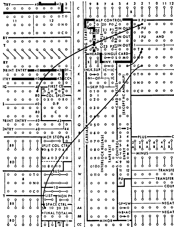
FIGURE 60. SPACE SUPPRESS
