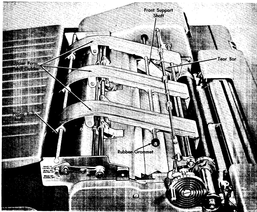
FIGURE 126. FORM FEED GUIDES
