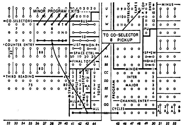
FIGURE 64. EXPANDING PROGRAM EXIT
