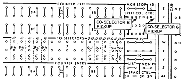
FIGURE 70. SPLIT COLUMN CONTROL
