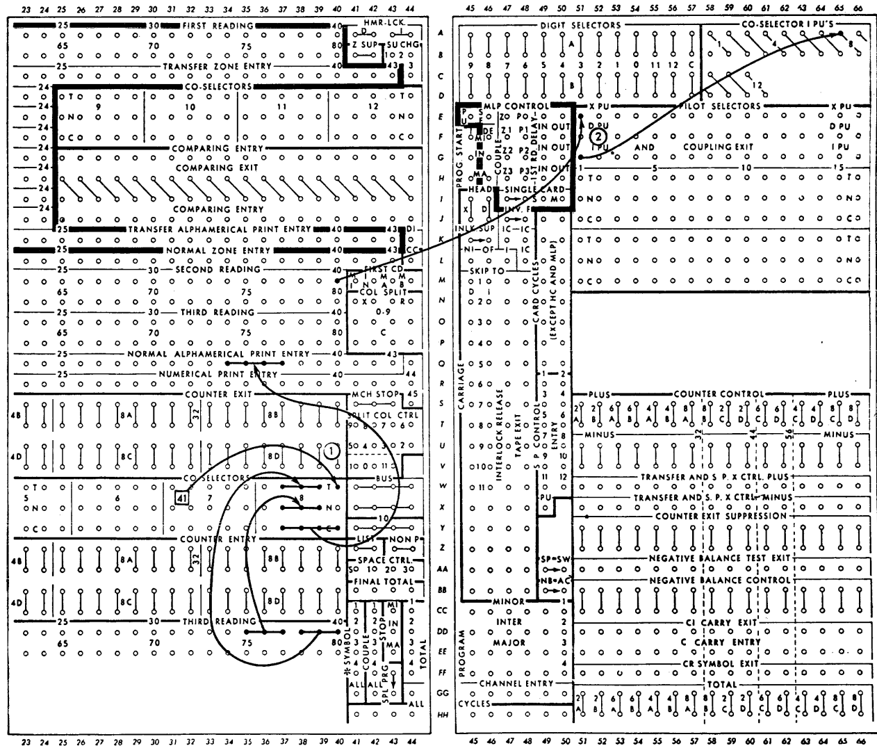
FIGURE 51. NUMERICAL FIELD SELECTION
