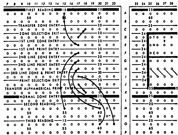
FIGURE 106. COMBINED ZONE AND PRINT SELECTION — SINGLE COLUMN
