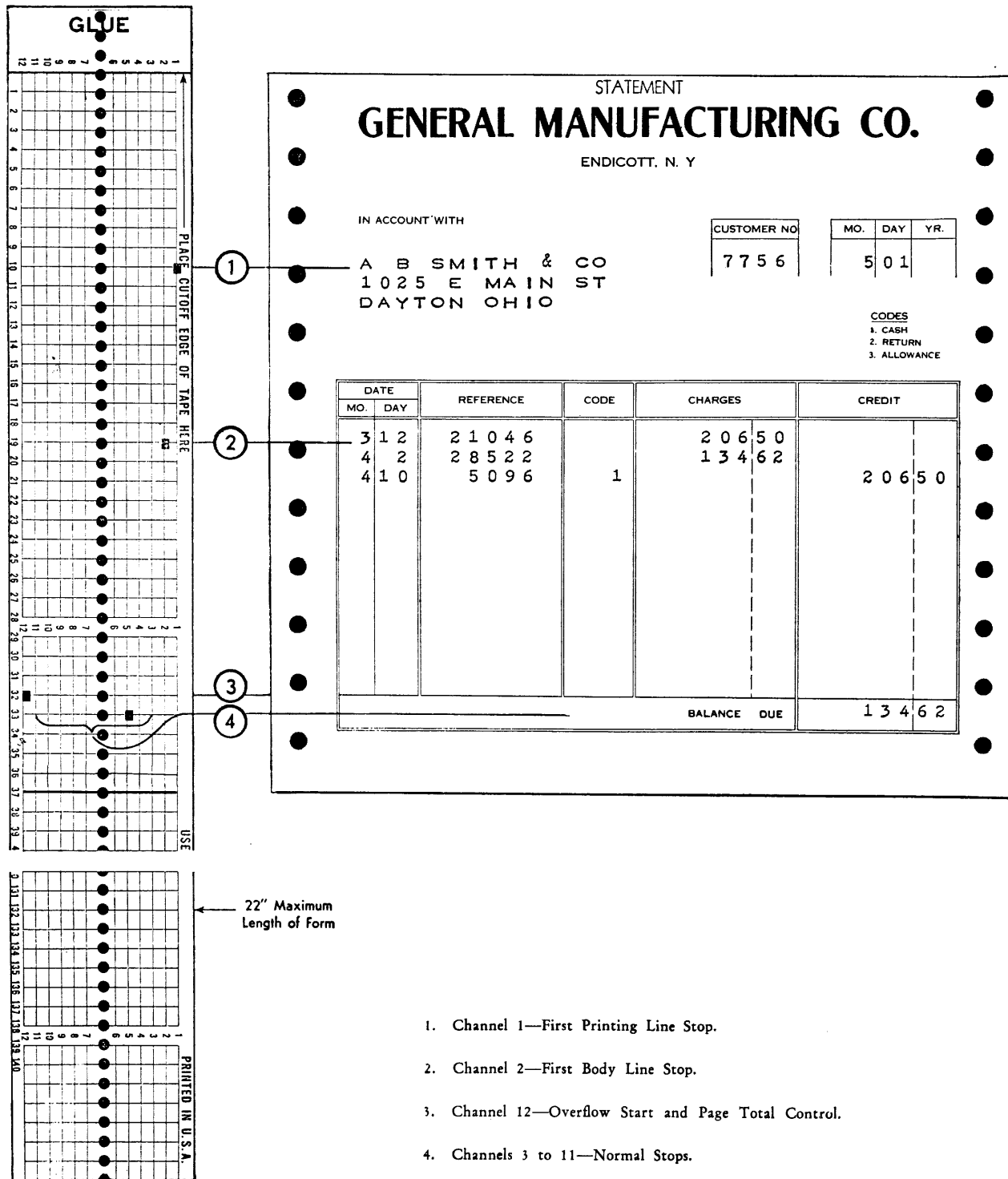
FIGURE 84. CONTROL TAPE
