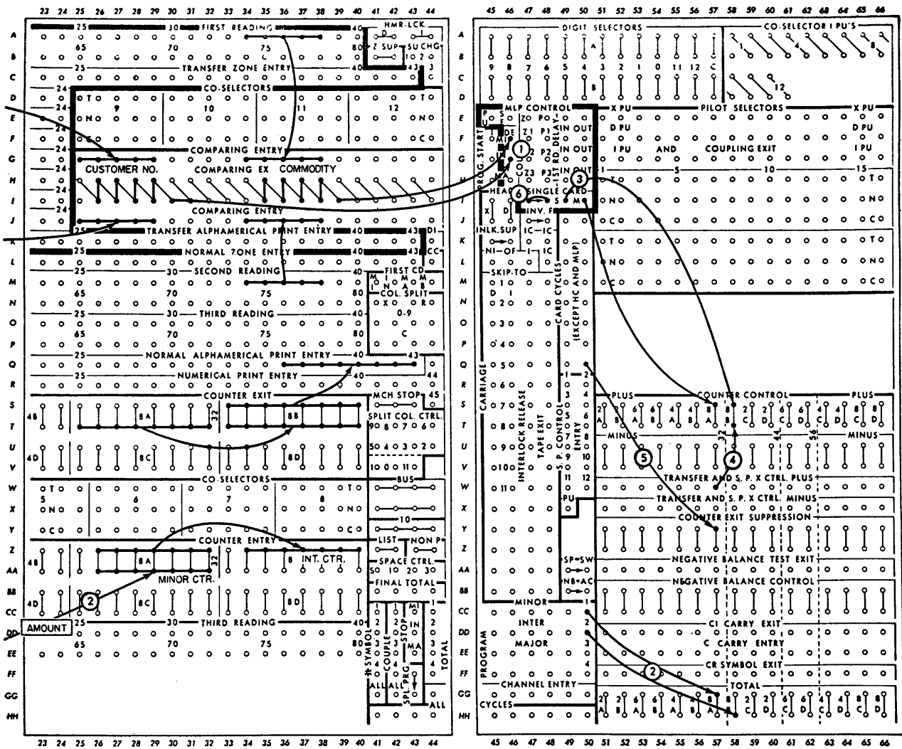
FIGURE 116. SINGLE CARD TOTAL ELIMINATION
