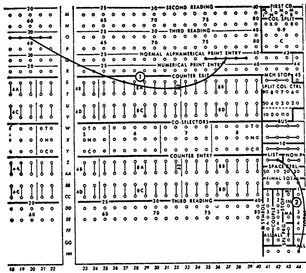
FIGURE 8. DETAIL PRINTING, NUMERICAL
