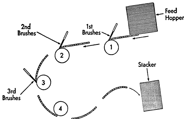
FIGURE 99. PATH OF CARD THROUGH THE TYPE 403
