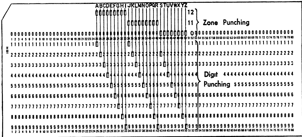
FIGURE 9. ALPHABETIC PUNCHING
