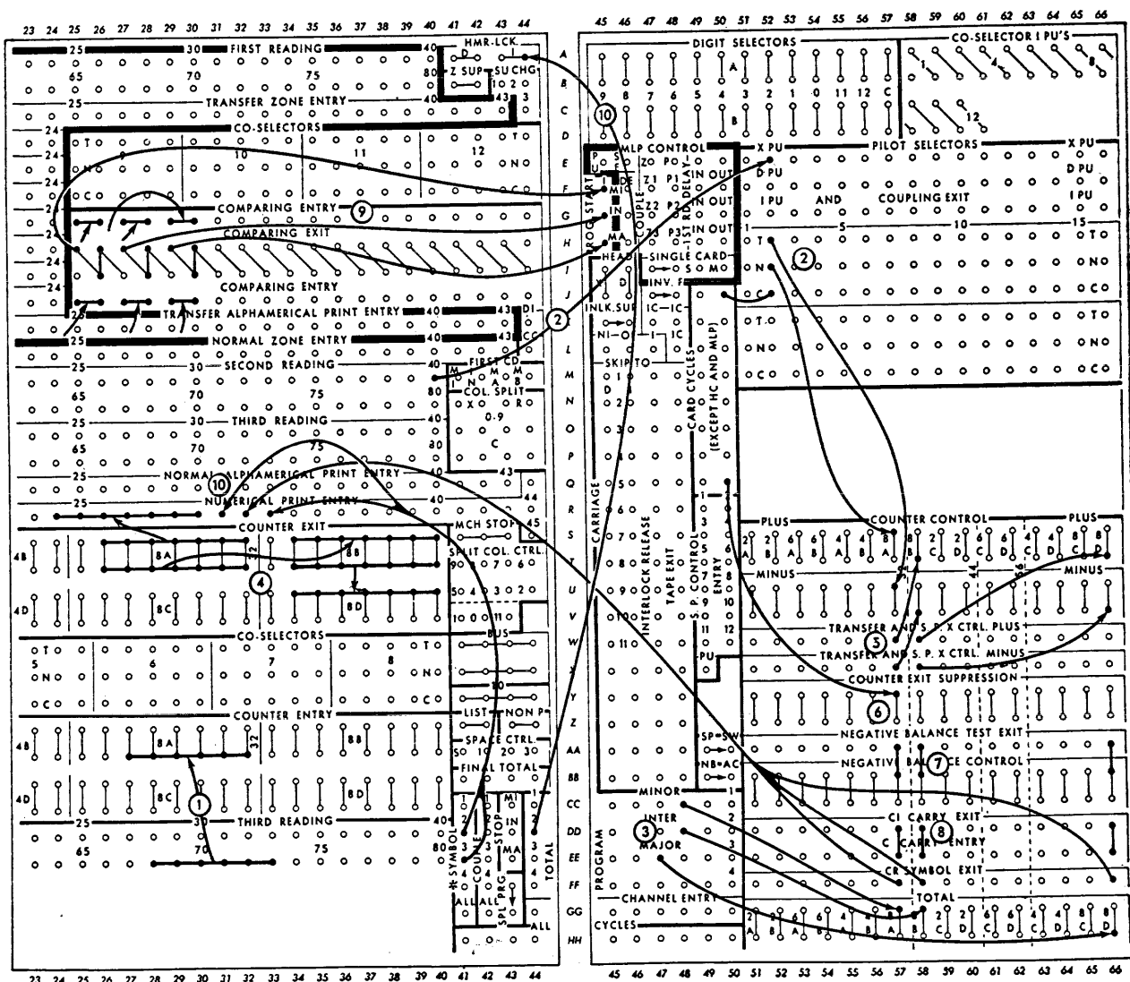
FIGURE 44. TOTAL TRANSFER — NET BALANCE
