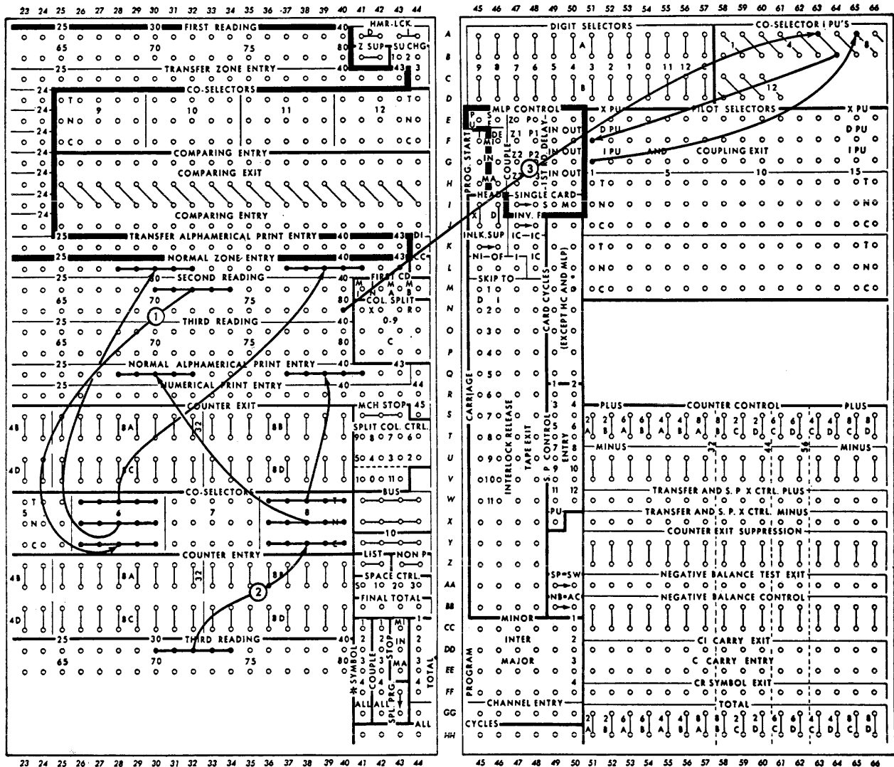
FIGURE 57. ALPHABETIC CLASS SELECTION
