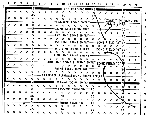
FIGURE 104. ZONE SELECTION — SINGLE COLUMN
