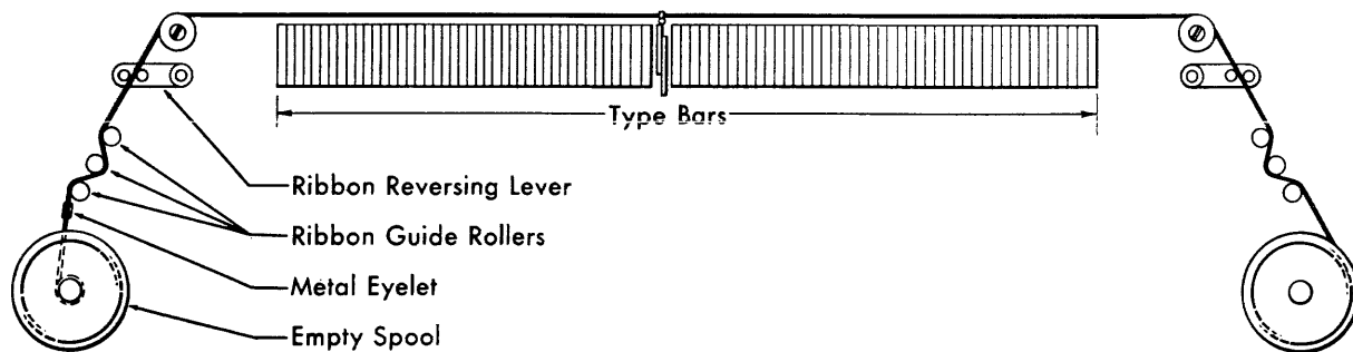
FIGURE 129. SCHEMATIC OF RIBBON FEED
