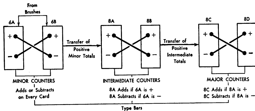
FIGURE 47. SCHEMATIC DIAGRAM OF TOTAL TRANSFER ON NON-NET BALANCE MACHINE
