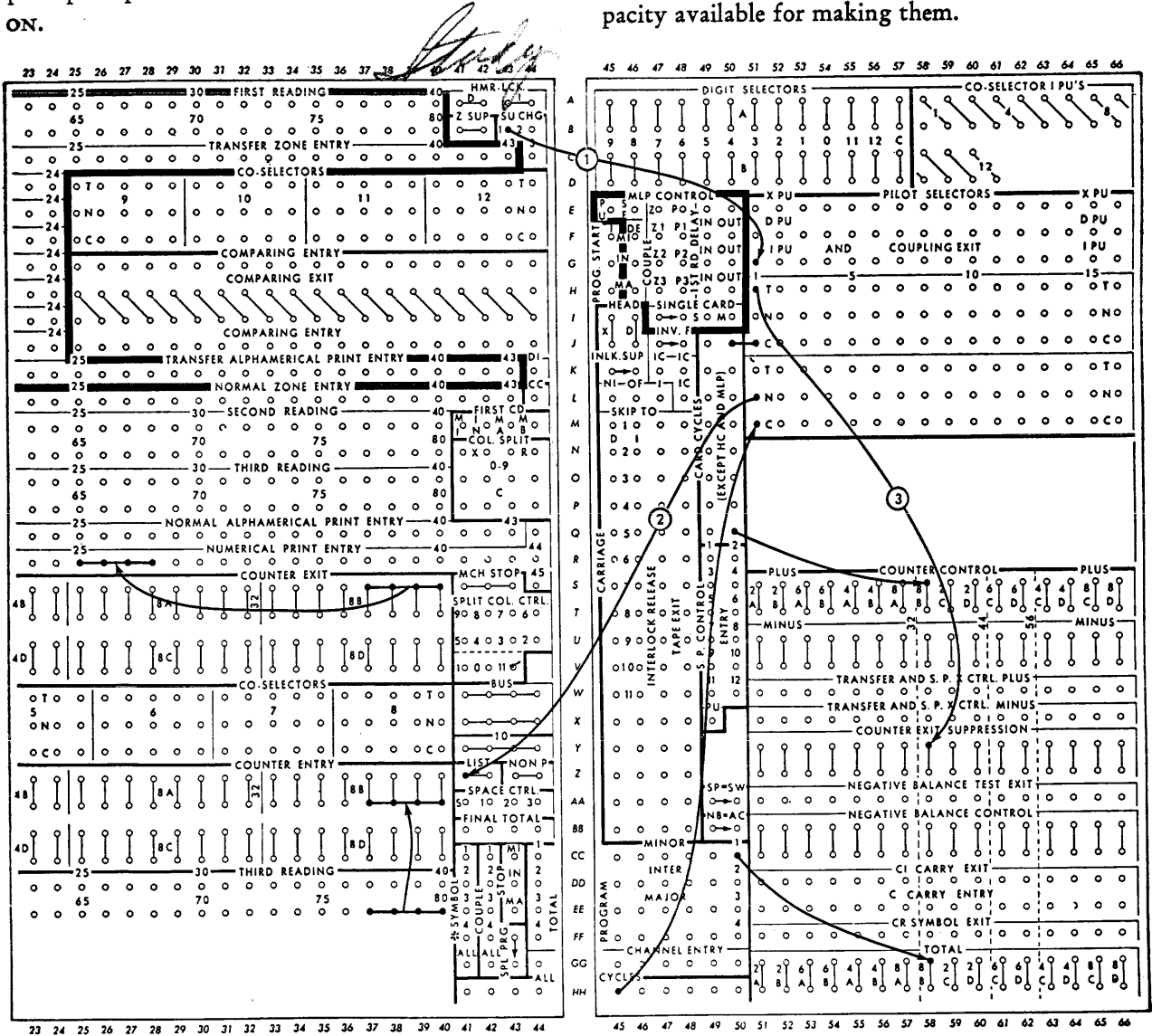
FIGURE 42. CHANGING FROM DETAIL PRINT TO GROUP PRINT
