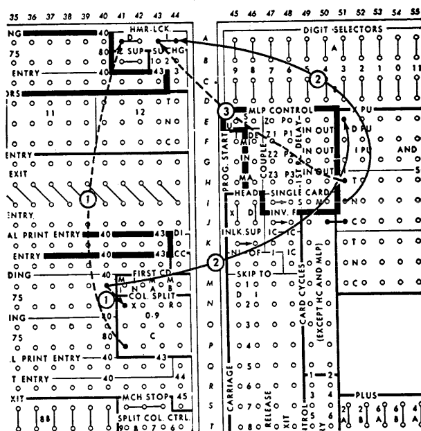
FIGURE 34. HAMMERLOCKING FOR X OR NX CARDS
