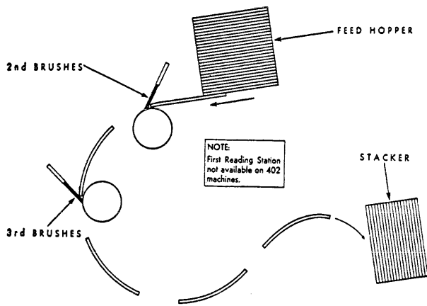
FIGURE 5. PATH OF CARD THROUGH THE TYPE 402
