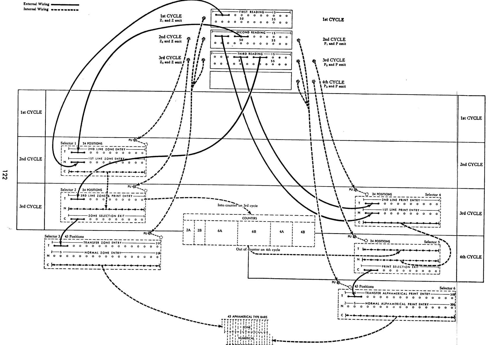
FIGURE 109. MLP SELECTOR SYSTEM
