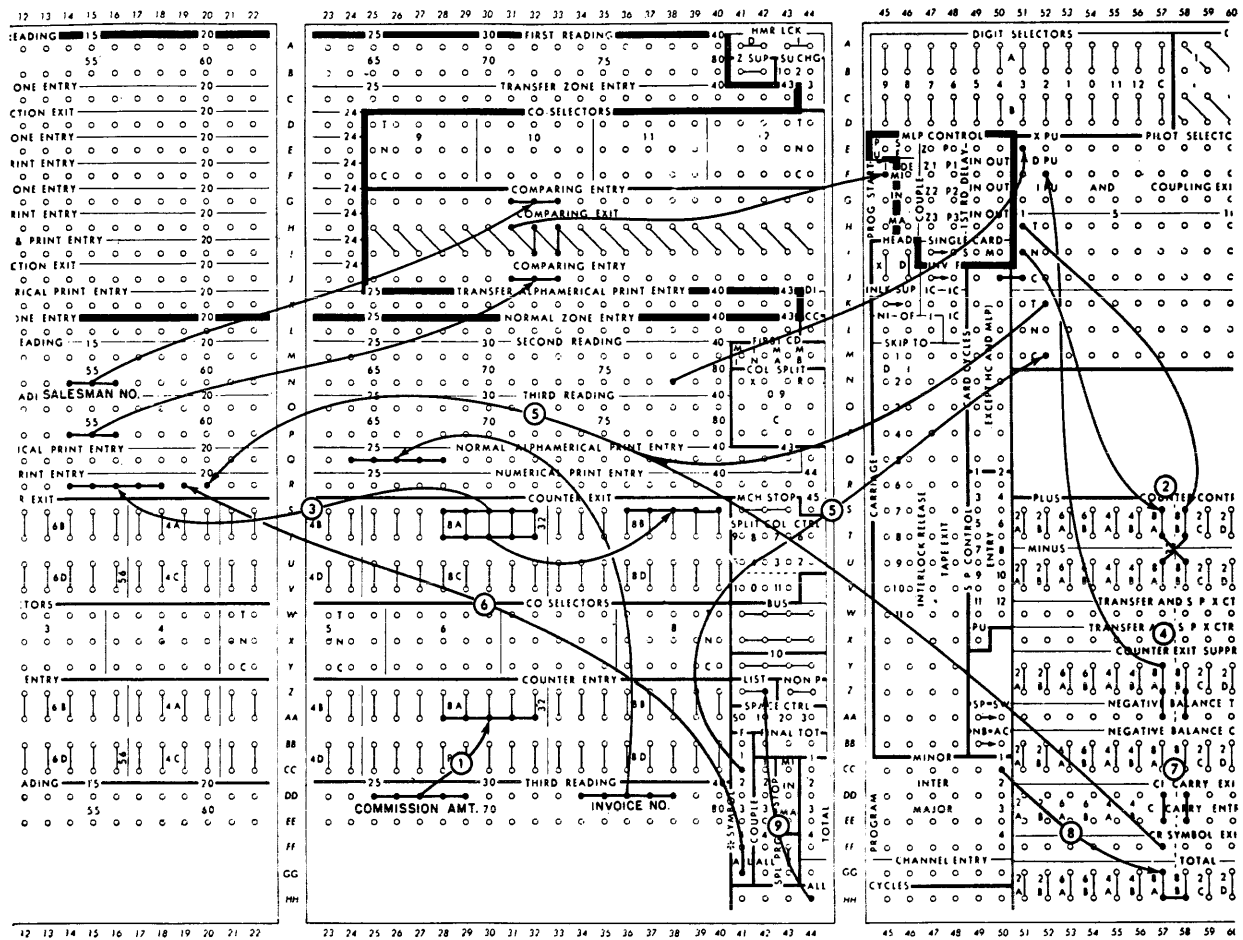
FIGURE 25. NON-NET BALANCE SUBTRACTION
