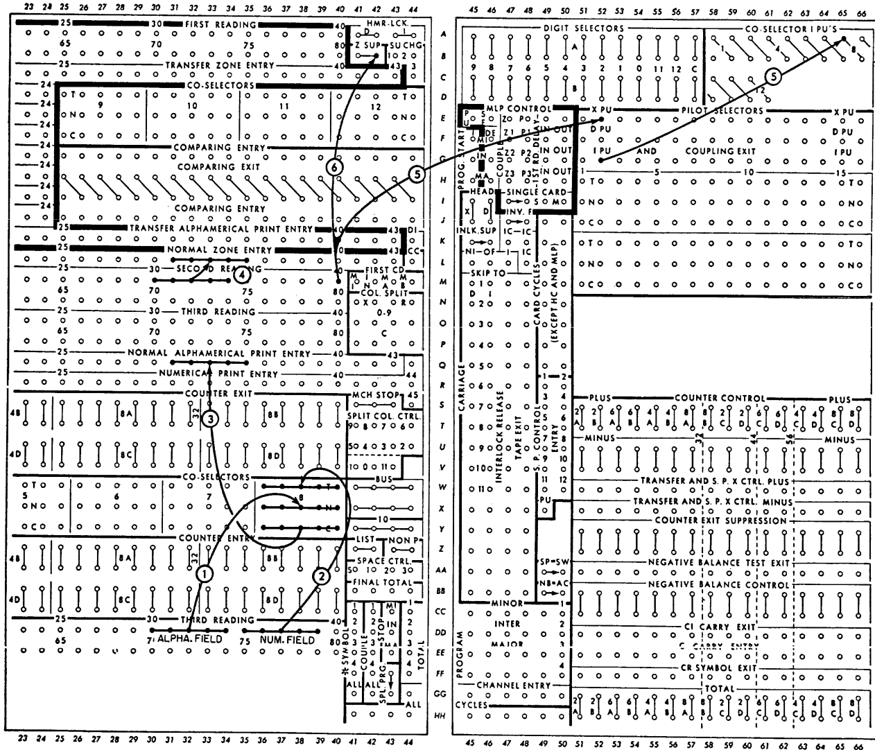
FIGURE 54. FIELD SELECTION OF ALPHABETIC AND NUMERICAL FIELDS
