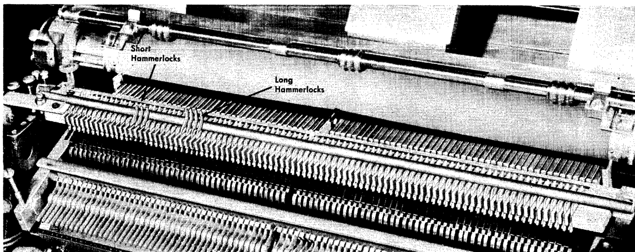
FIGURE 33. HAMMERLOCK LEVERS
