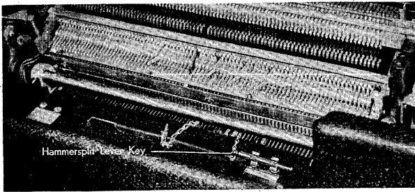
FIGURE 12. HAMMERSPLIT LEVERS
