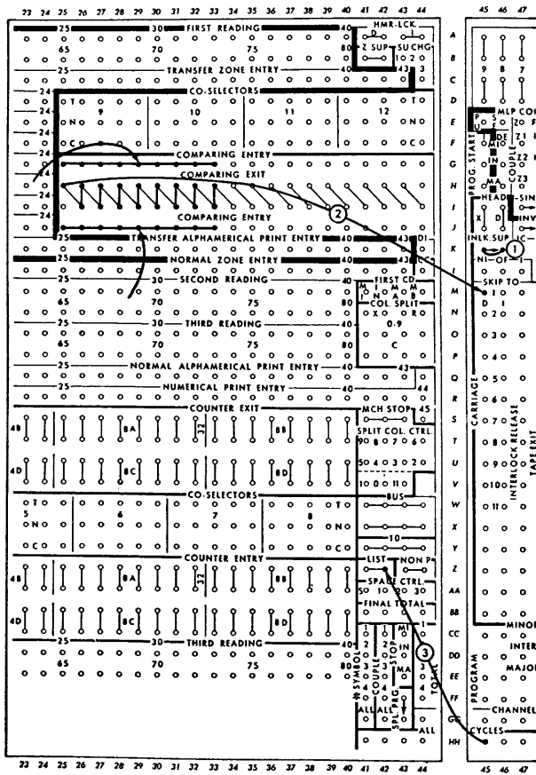
FIGURE 92. SHORT FORM SKIPPING
