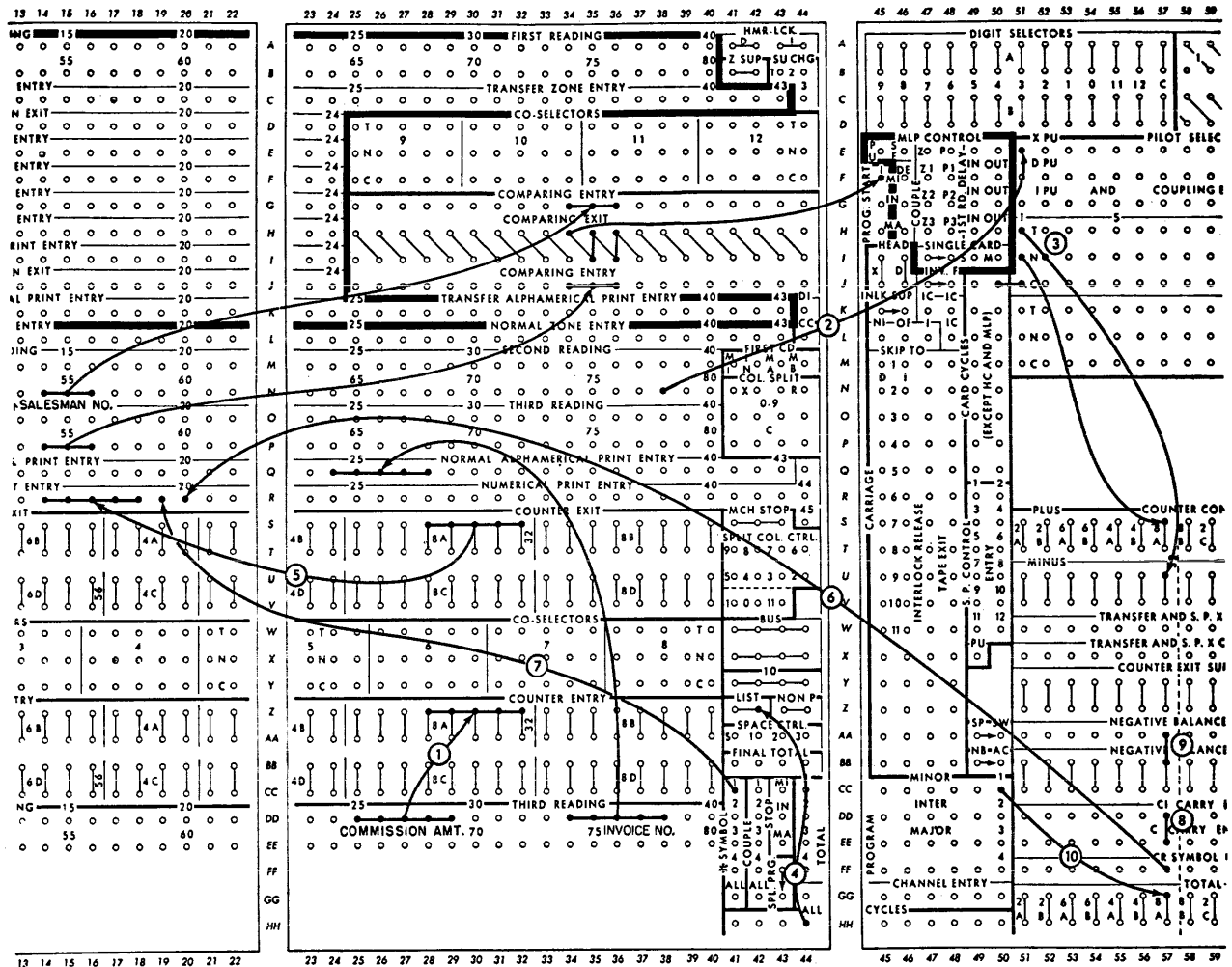
FIGURE 24. NET BALANCE SUBTRACTION
