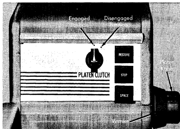
FIGURE 86. CARRIAGE FEATURES
