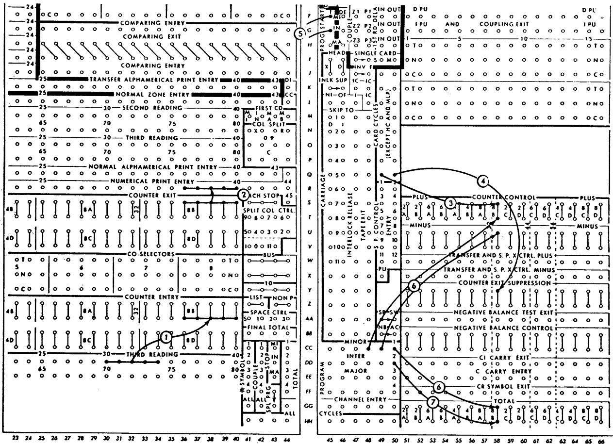
FIGURE 78. PROGRESSIVE TOTAL PRINTING
