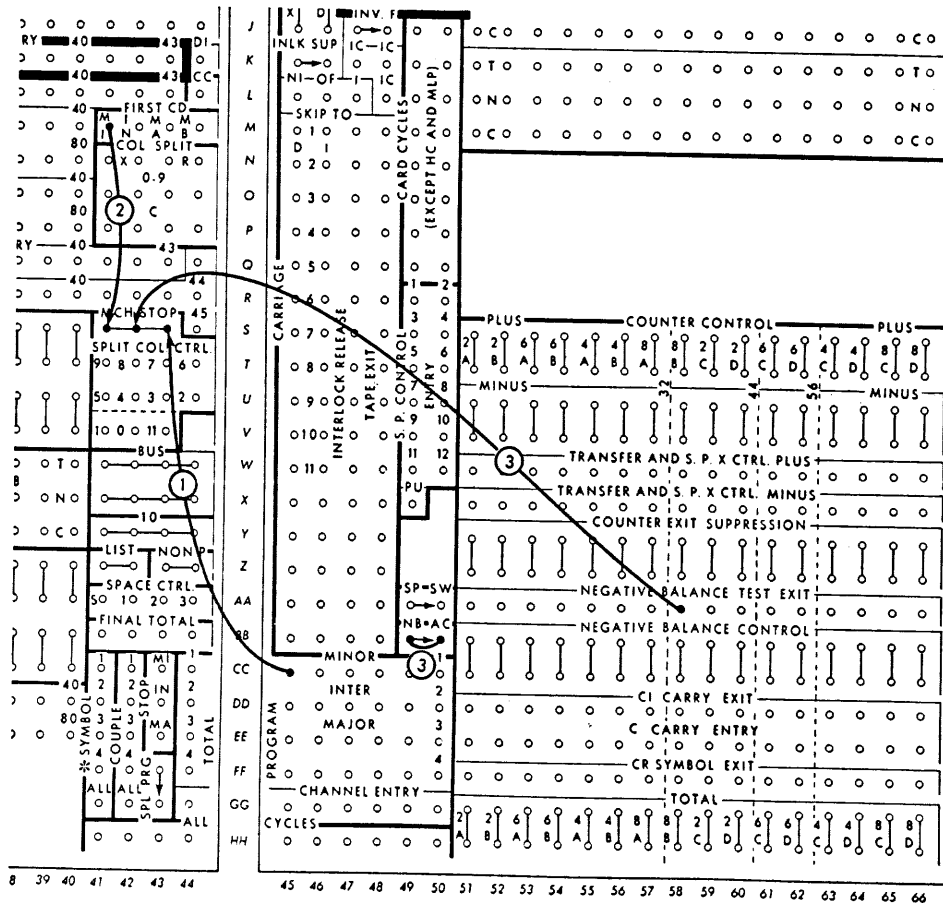
FIGURE 67. MACHINE STOP
