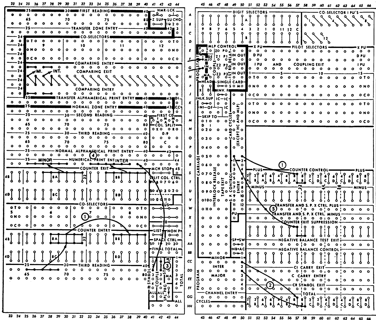
FIGURE 62. MINOR AND INTERMEDIATE TOTALS ON THE SAME LINE
