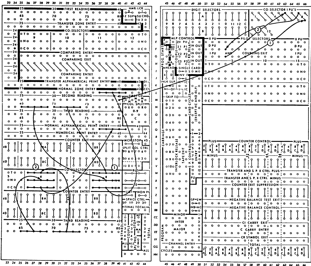
FIGURE 52. ALPHABETIC FIELD SELECTION
