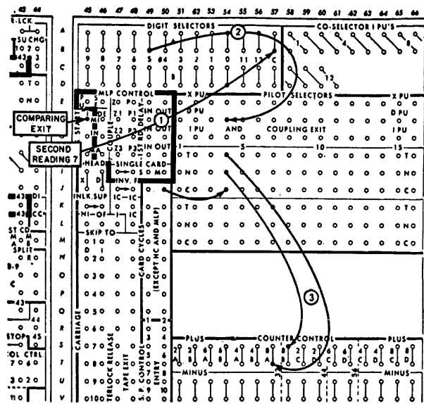
FIGURE 28. DIGIT SELECTION
