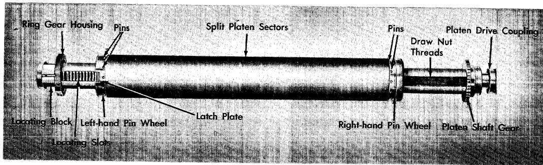
FIGURE 122. MODEL P-2 IBM PIN FEED PLATEN
