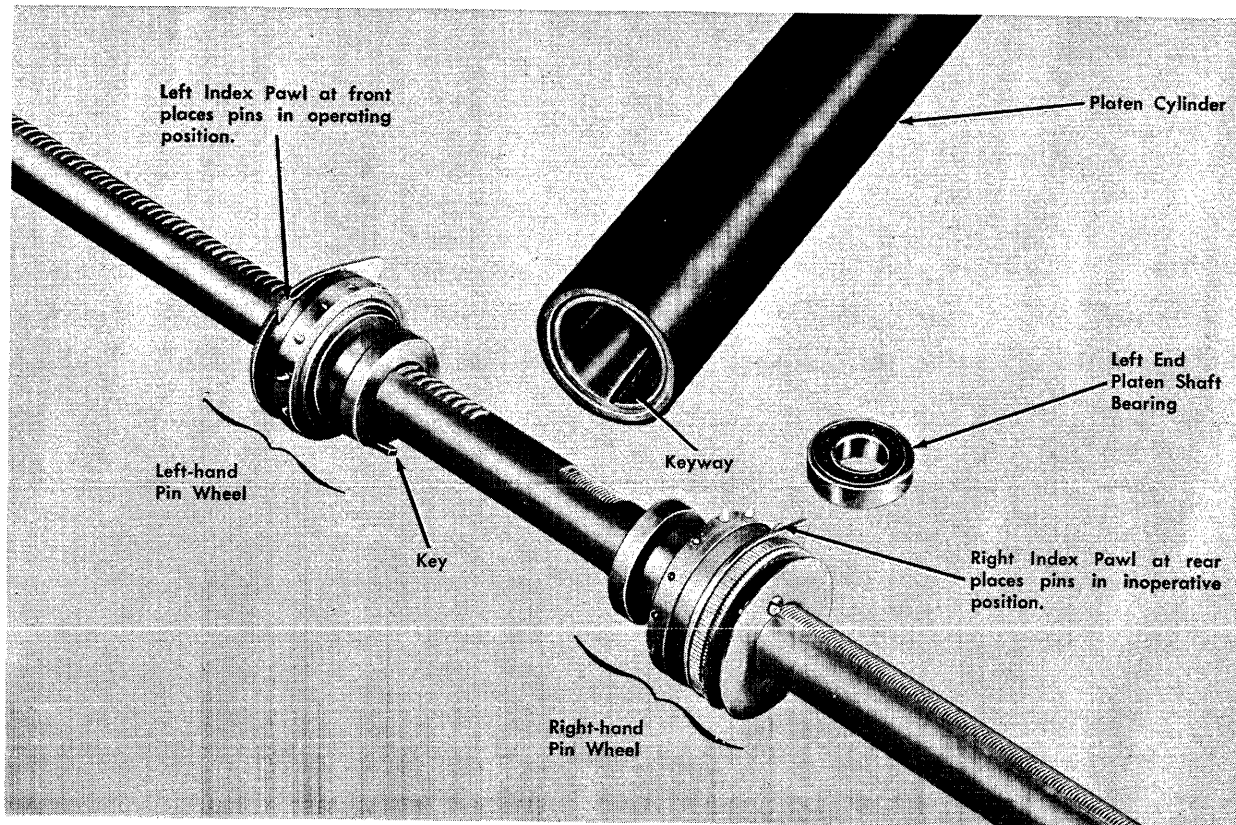
FIGURE 123. MODEL P-3 PINS IN OPERATING AND INOPERATIVE POSITION
