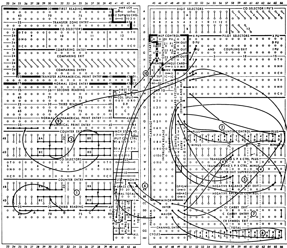
FIGURE 49. THREE FIELD CROSSFOOTING — NON-NET BALANCE
