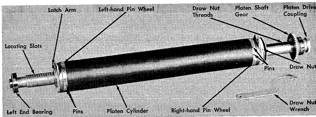
FIGURE 121. MODEL P-3 IBM PIN FEED PLATEN
