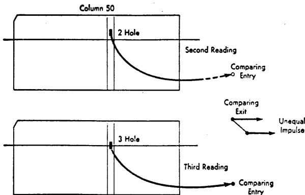
FIGURE 16. COMPARING
