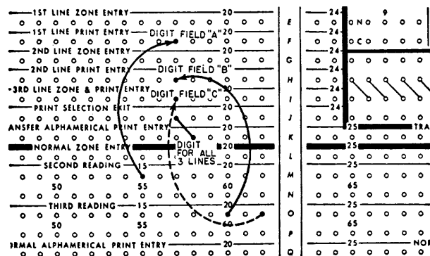
FIGURE 105. PRINT SELECTION — SINGLE COLUMN
