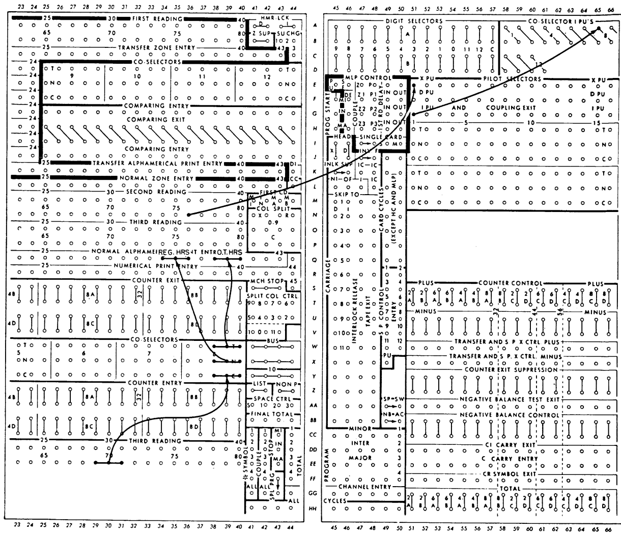
FIGURE 56. NUMERICAL CLASS SELECTION
