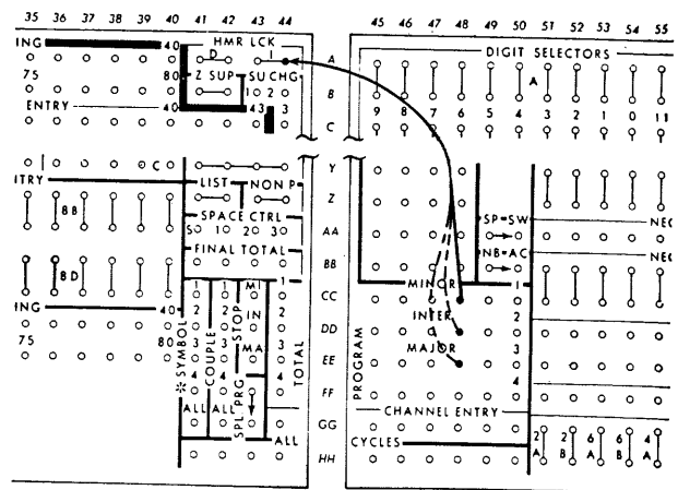
FIGURE 37. HAMMERLOCKING FROM TOTAL PROGRAM EXITS
