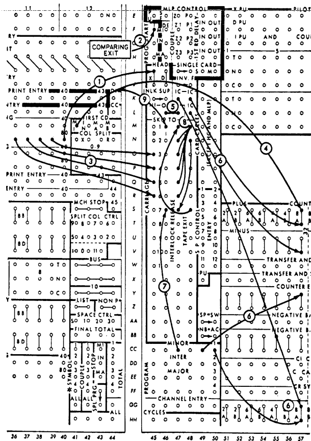
FIGURE 96. MULTIPLE HEADING GROUPS
