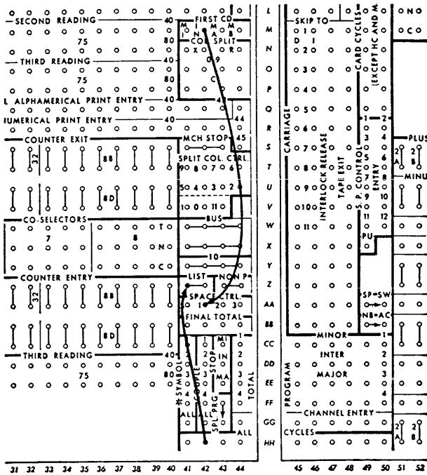
FIGURE 63. FIRST CARD SPACE CONTROL
