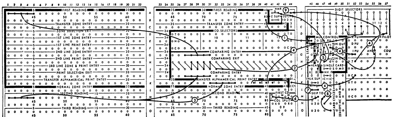
FIGURE 111. MLP FOLLOWED BY NORMAL CARDS
