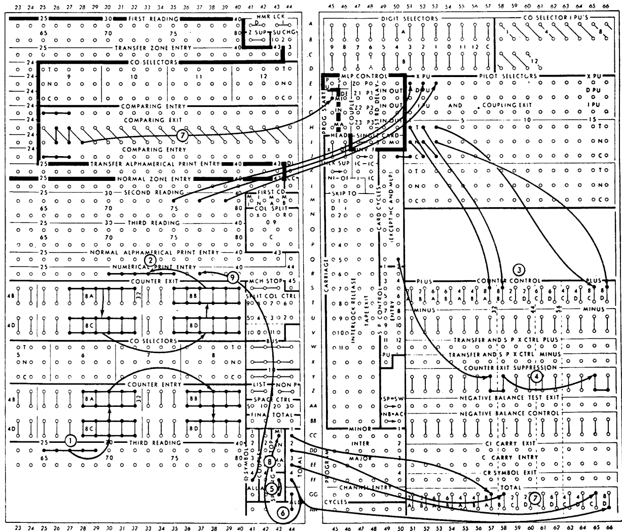
FIGURE 81. FOUR MINOR TOTALS — SAME TYPE BARS
