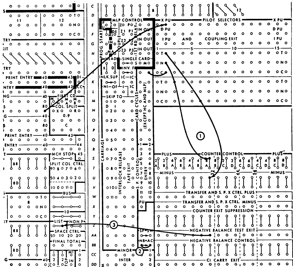
FIGURE 68. DETAIL PRINTING NB-AC
