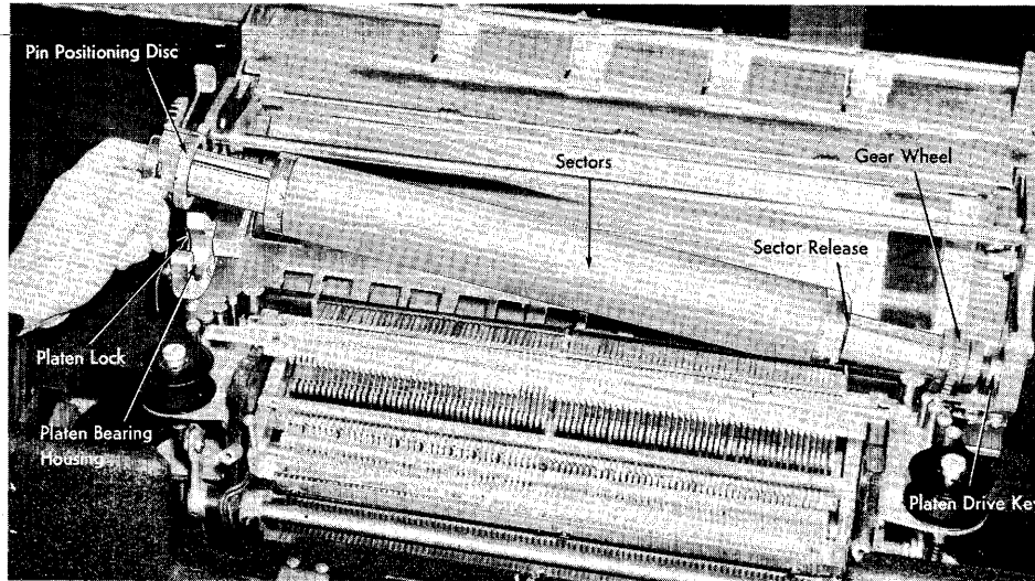
FIGURE 88. PLATEN ASSEMBLY
