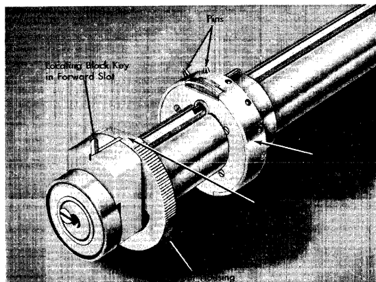
FIGURE 125. MODEL P-2 PINS IN THE INOPERATIVE POSITION
