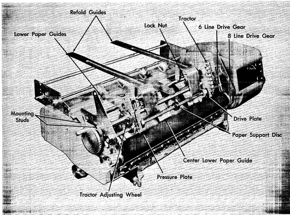
FIGURE 127. MODEL F-3 IBM FORMS TRACTOR ON TAPE-CONTROLLED CARRIAGE
