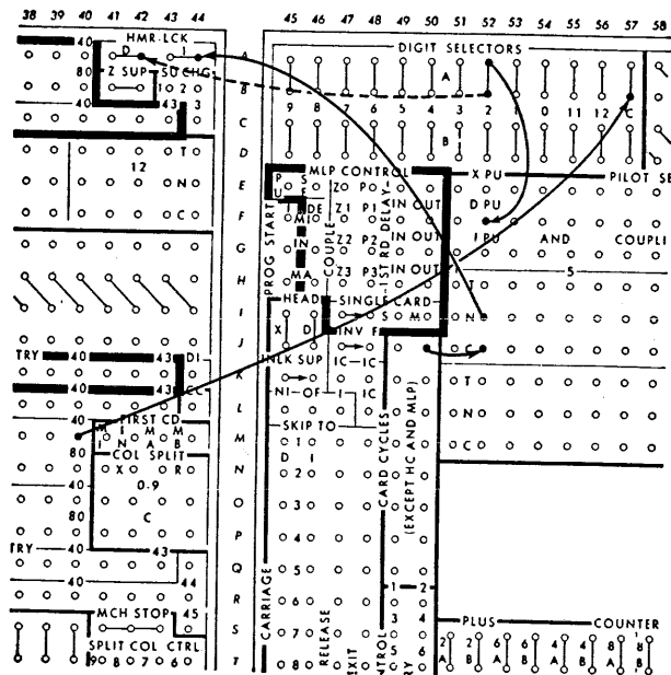
FIGURE 35. HAMMERLOCKING FOR D OR NO D CARDS
