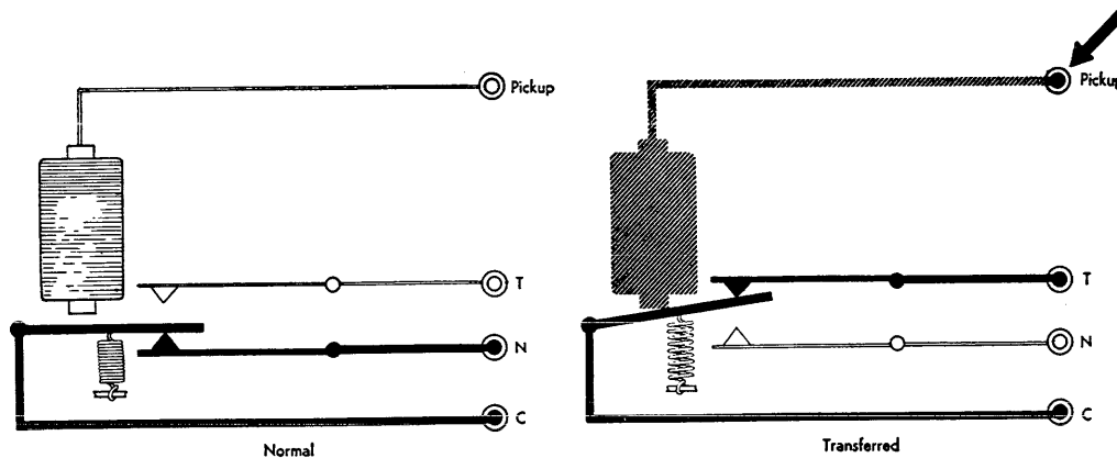
FIGURE 21. SCHEMATIC DIAGRAM OF A SELECTOR
