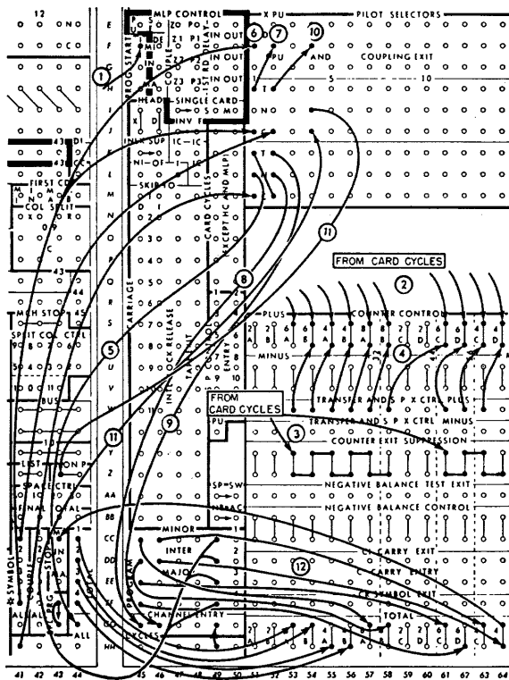
FIGURE 83. CROSSFOOTING TEN TOTALS
