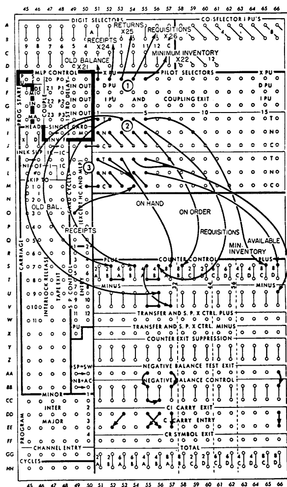
FIGURE 66. MULTIPLE X SELECTION
