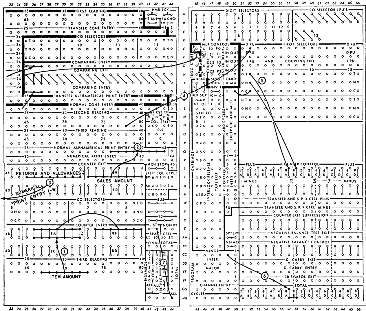
FIGURE 27. X SELECTION
