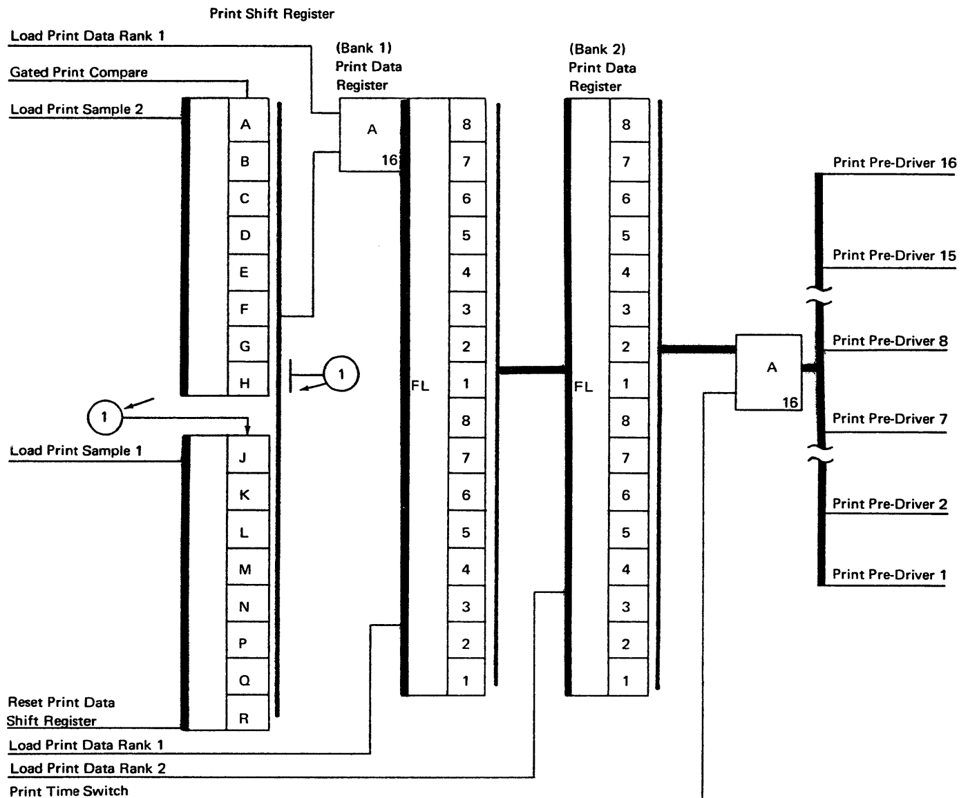
Figure 2-15. Print Shift Register and Print Data Registers
