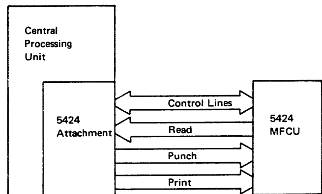
Figure 1-1. 5424 Data Flow
