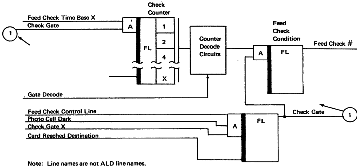
Figure 2-21. Check Counters
