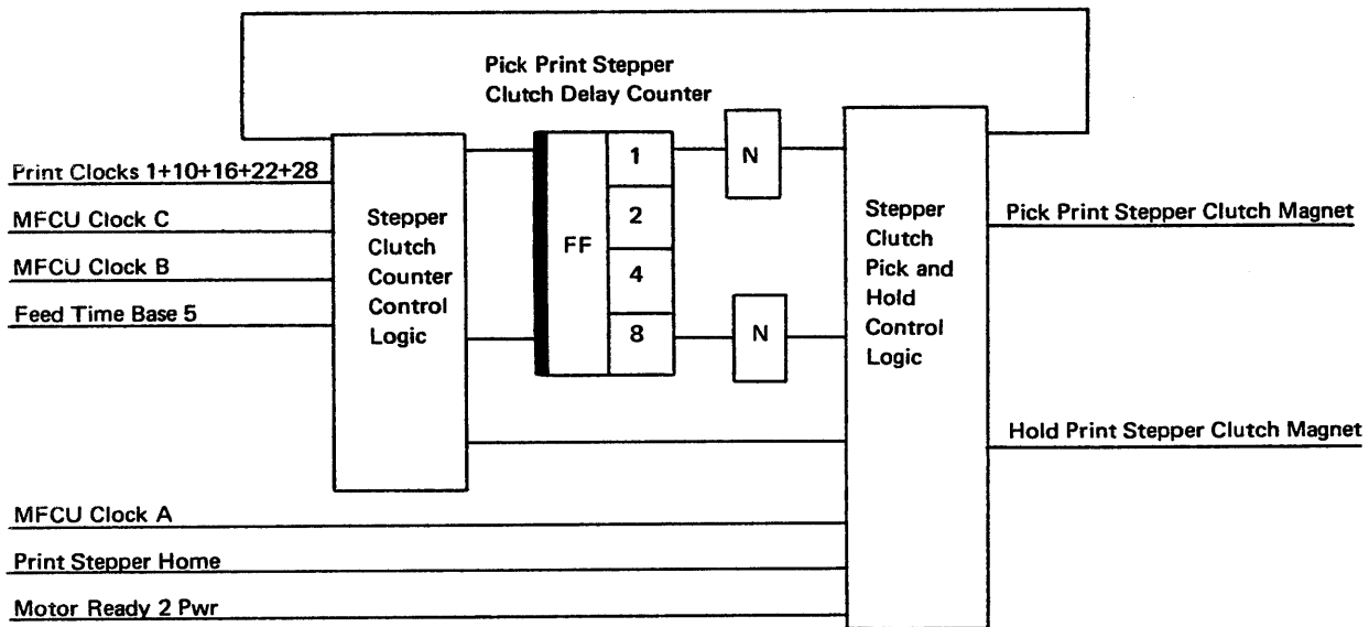
Figure 2-17. Pick Print Stepper Clutch Delay Counter
