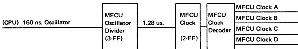
Figure 2-1. MFCU Clock
