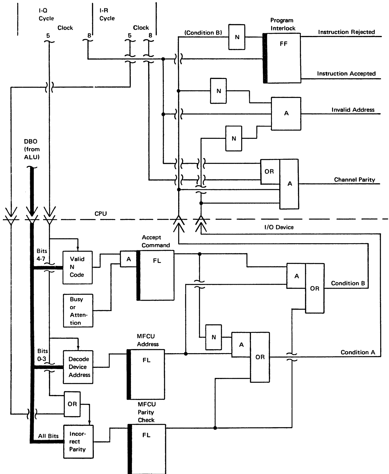
Figure 1-2. SIO-CPU/MFCU Control
