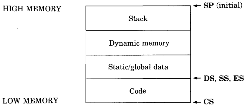
Figure F.3 Version 2.03 Layout for the S and P Models
