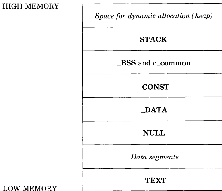
Figure 10.1 Segment Setup in C Programs
