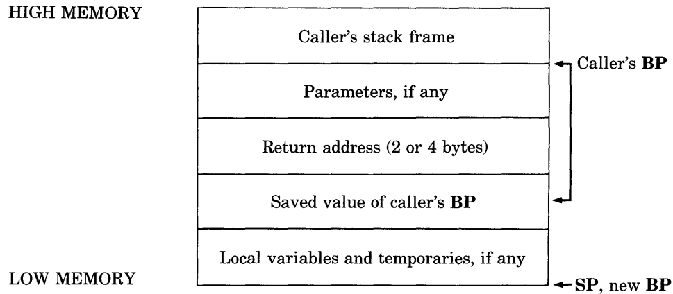
Figure F.1 Version 2.03 Stack Frame Setup
