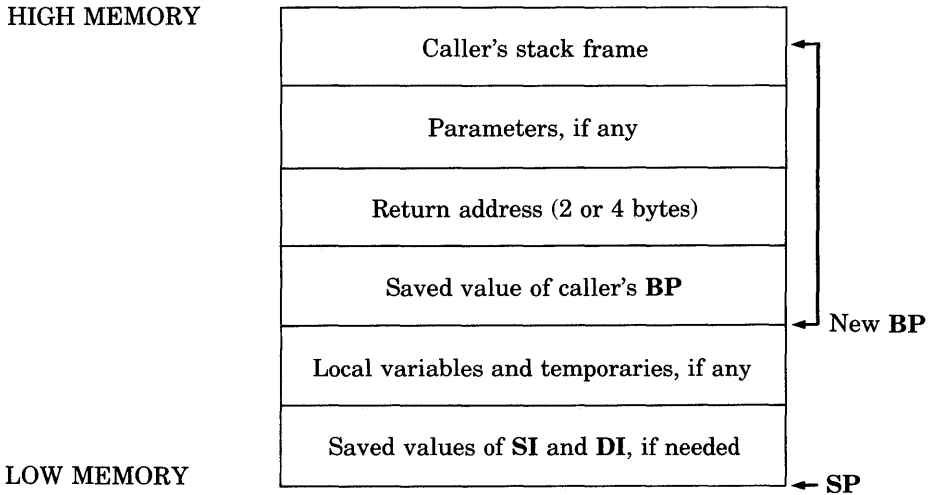
Figure F.2 Version 3.0 Stack Frame Setup
