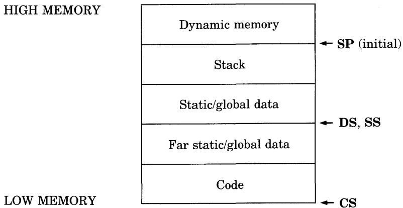
Figure F.4 Layouts for the 3.0 and 4.0 Versions
