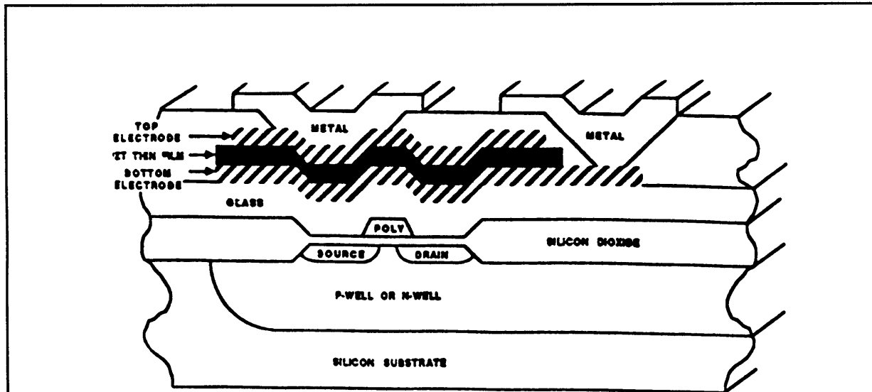
Figure 14. A ferroelectric non-volatile random access memory can retain its state after the loss of power due to the fact that a ferroelectric material can have its permanent polarization charge reversed with the application of an electric field [Ramtron 88].
