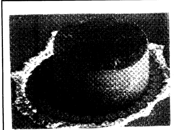
Figure 7. A wobble motor, extruded as opposed to silicon micromachined, uses electrostatic forces applied by the surrounding stator electrodes to force the rotor to "wobble" much like a harmonic gear [Jacobsen et al 89]. Reprinted by permission.
