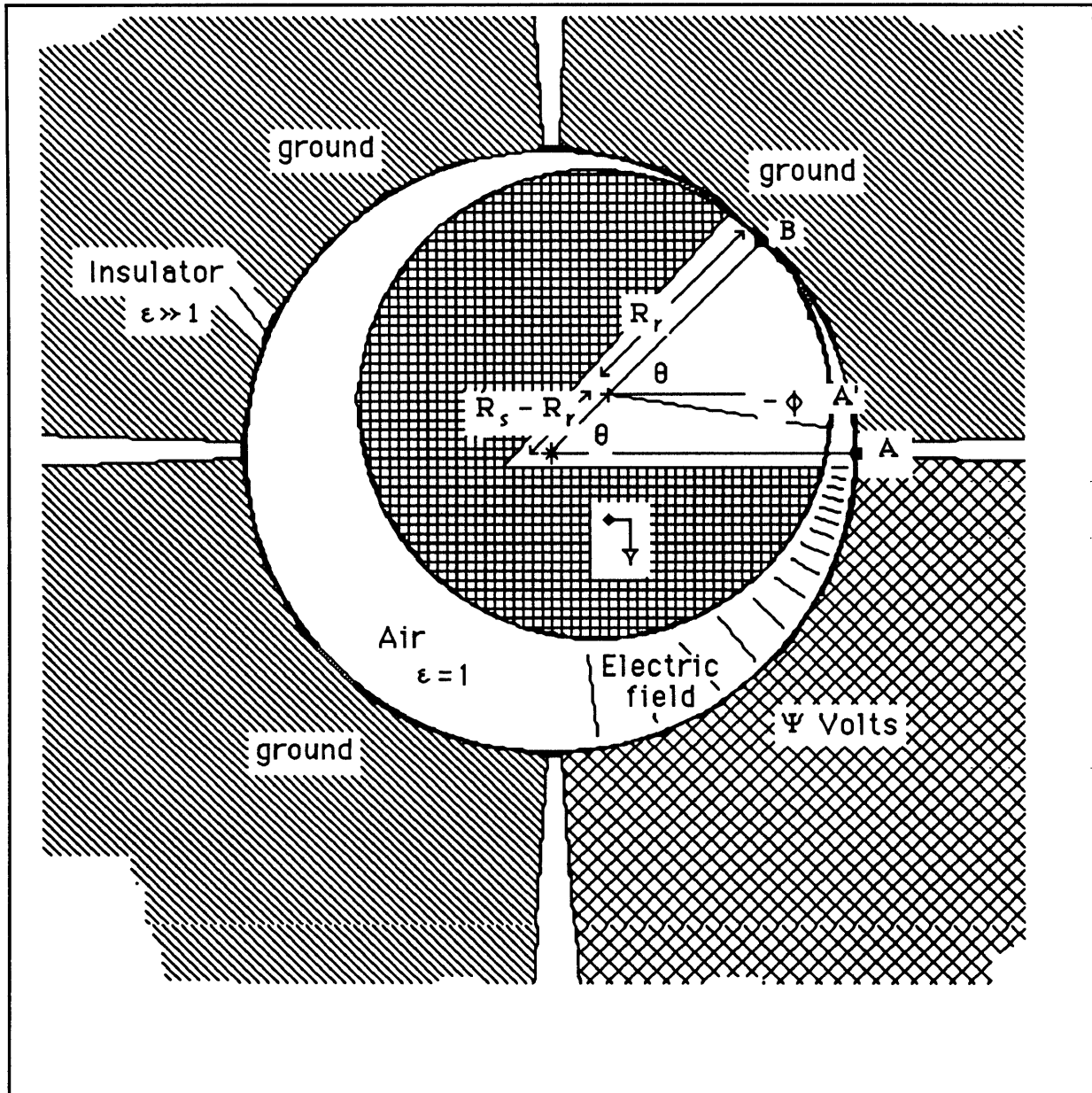
Figure 8. In a wobble motor, stators are pulsed in turn, attracting the rotor with the collapsing force of a capacitor as shown by the electric field lines in the diagram. This causes the rotor to roll inside the housing. The wobble motor provides inherent gear reduction as it takes many electrical cycles around the stator to achieve one rotation of the rotor.
