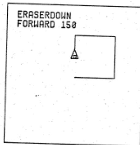
Figure 2b. The turtle erases part of one side of the square by going over it with the eraser down.
