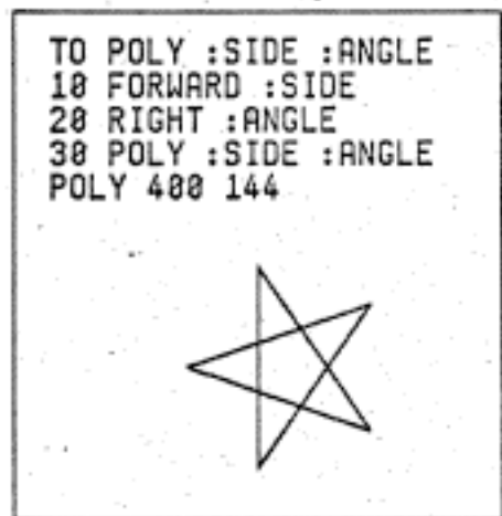
Figure 1f. A typical procedure for drawing polygons. Note that the recursion does not terminate, and the procedure must be stopped by hand.
