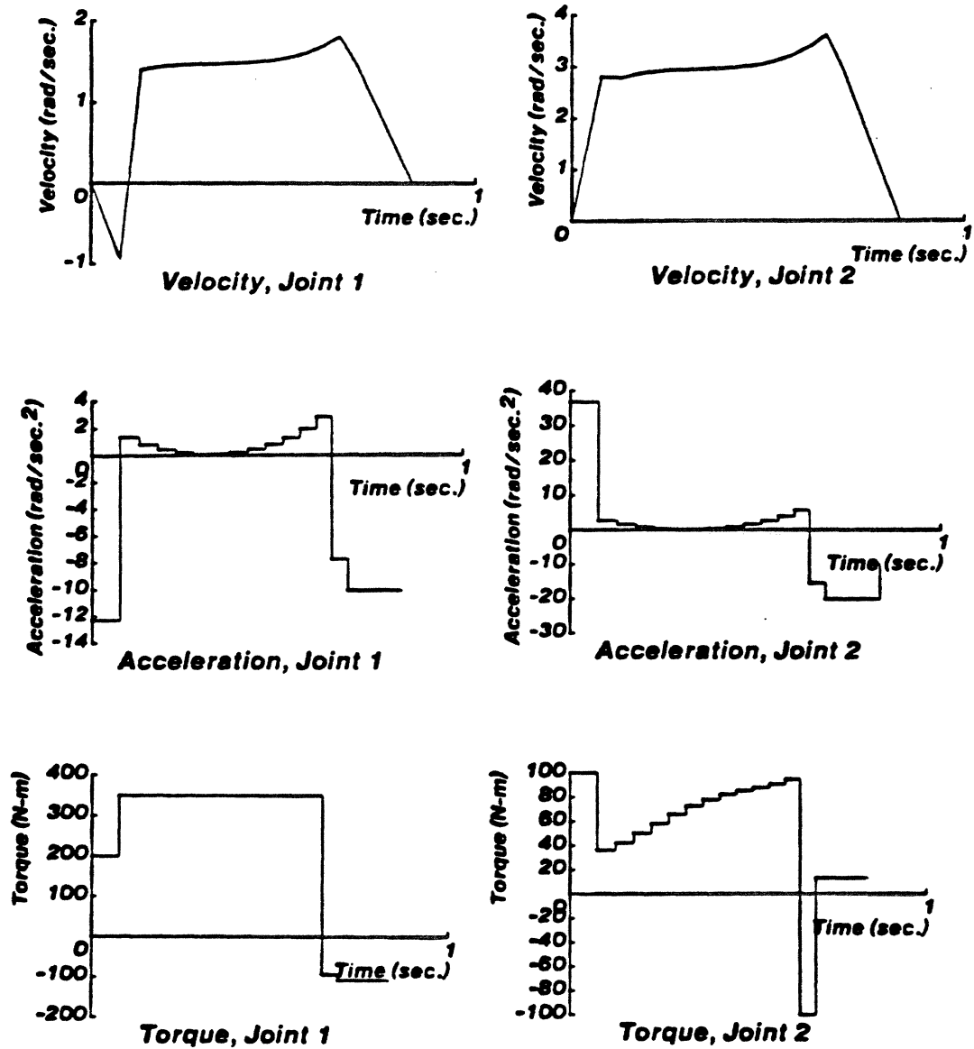
Figure 5: Moving from (-0.5, -1.0) to (0.5, 1.0) : velocity, acceleration, and torque at the joints
