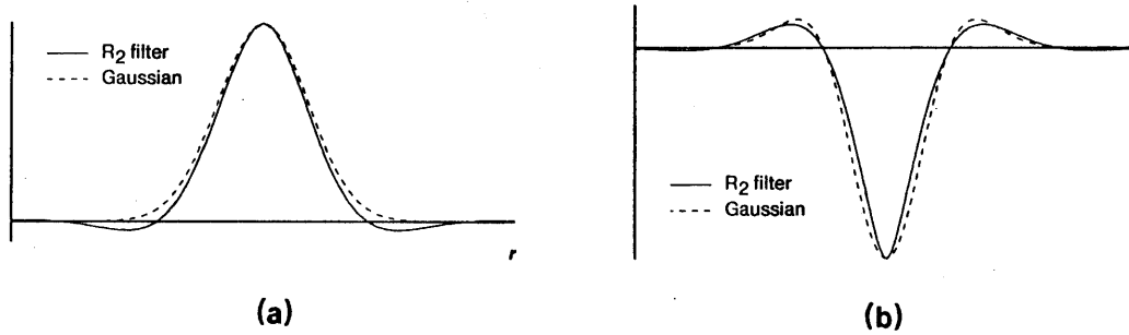
Figure 6 Cross section of (a) two-dimensional regularization filter R_2 and (b) its Laplacian.
