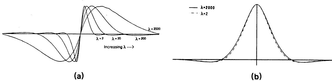
Figure 3 Filter R and first derivative for different values of regularizing parameter \lambda . (a) \lambda affects size of (the first derivative of) R but (b) does not appear to affect shape of R . (Amplitudes are normalized in (a); both amplitudes and widths are scaled linearly and independently in (b) for comparison.)
