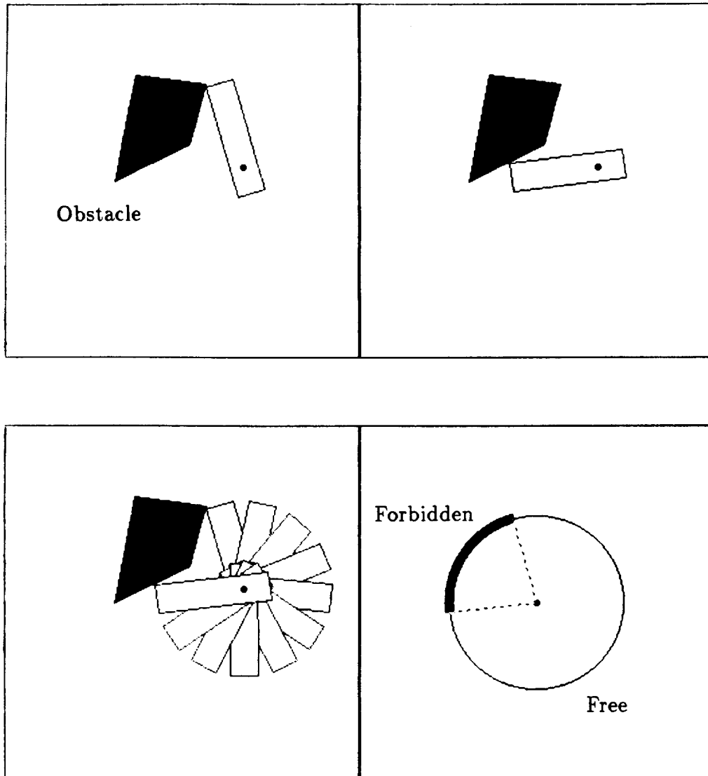
Figure 10. This figure considers the constraints imposed by an obstacle polygon on the possible orientations of a rectangle rotating about a rotation center. The first two frames show the rectangle in two orientations that just touch the obstacle. The third frame shows the free range of motions possible. The last frame represents the range of forbidden and free orientations.
