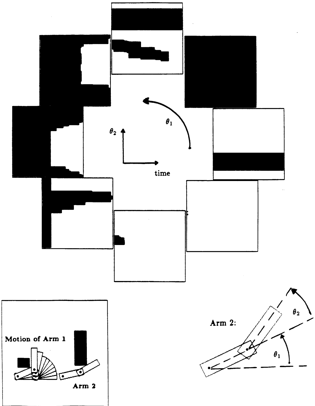
Figure 28. Several slices of the configuration space-time representing the constraints imposed on the right arm by the motion of the left arm and by the stationary obstacles in the environment. Each slice depicts the constraints imposed on Link 2 for a fixed orientation of Link 1.
