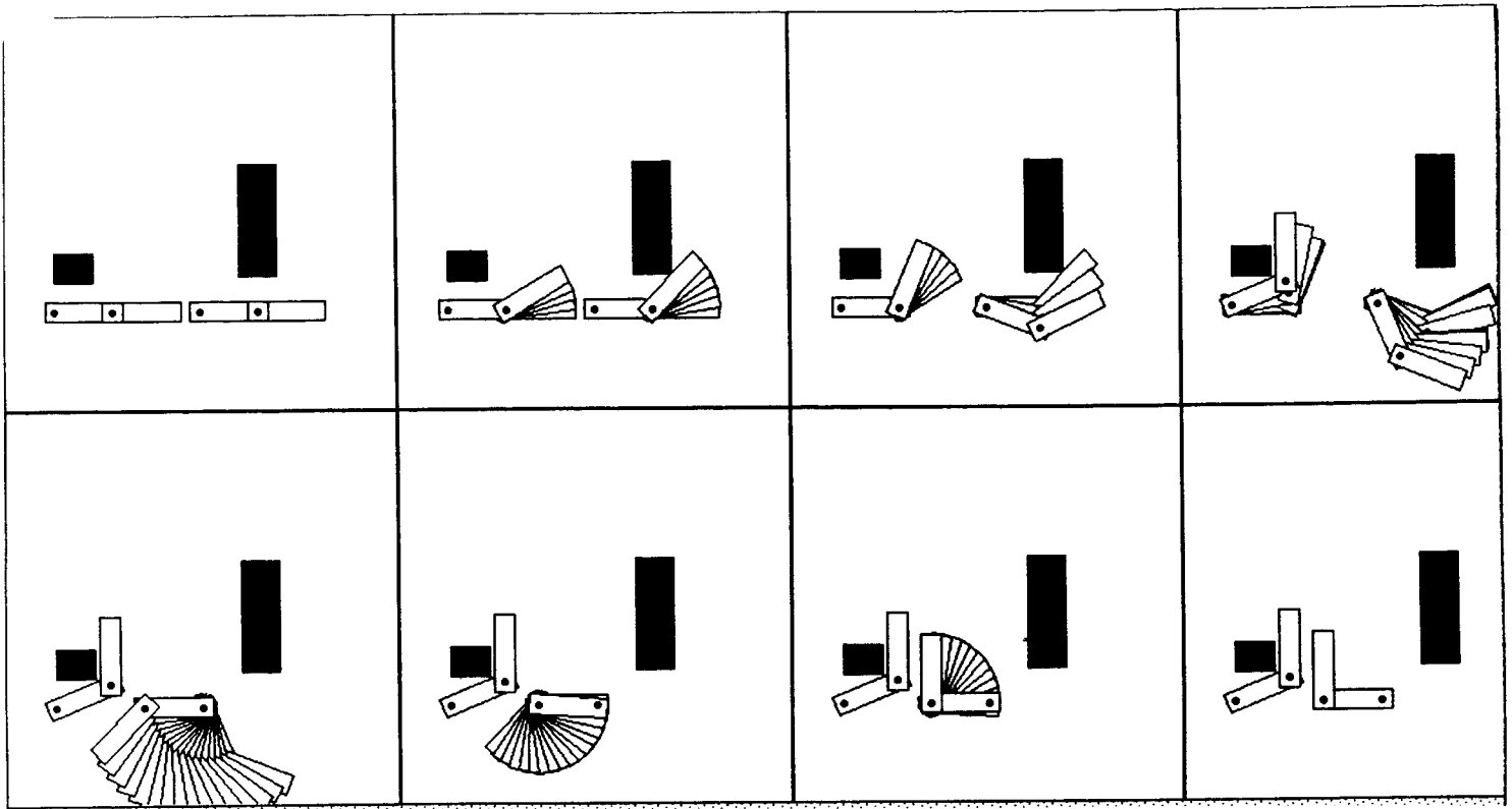
Figure 26. Some sample snapshots of the motions determined by the planner while solving the problem of Figure 25.
