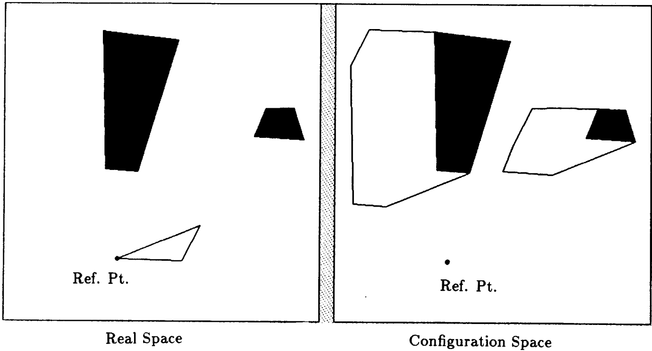
Figure 6. The left figure consists of a translating triangle, and two stationary obstacles. The right figure displays the configuration space constraints imposed on the triangle by the obstacles. For comparison, the constraints are superimposed on the actual obstacles.
