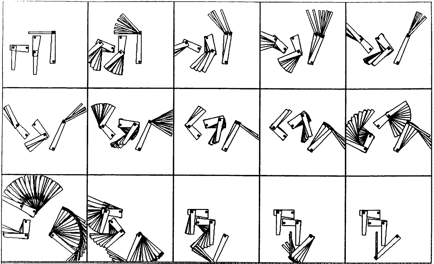
Figure 4. This figure traces a solution determined by our planner for the three articulated arms of Figure 3.
