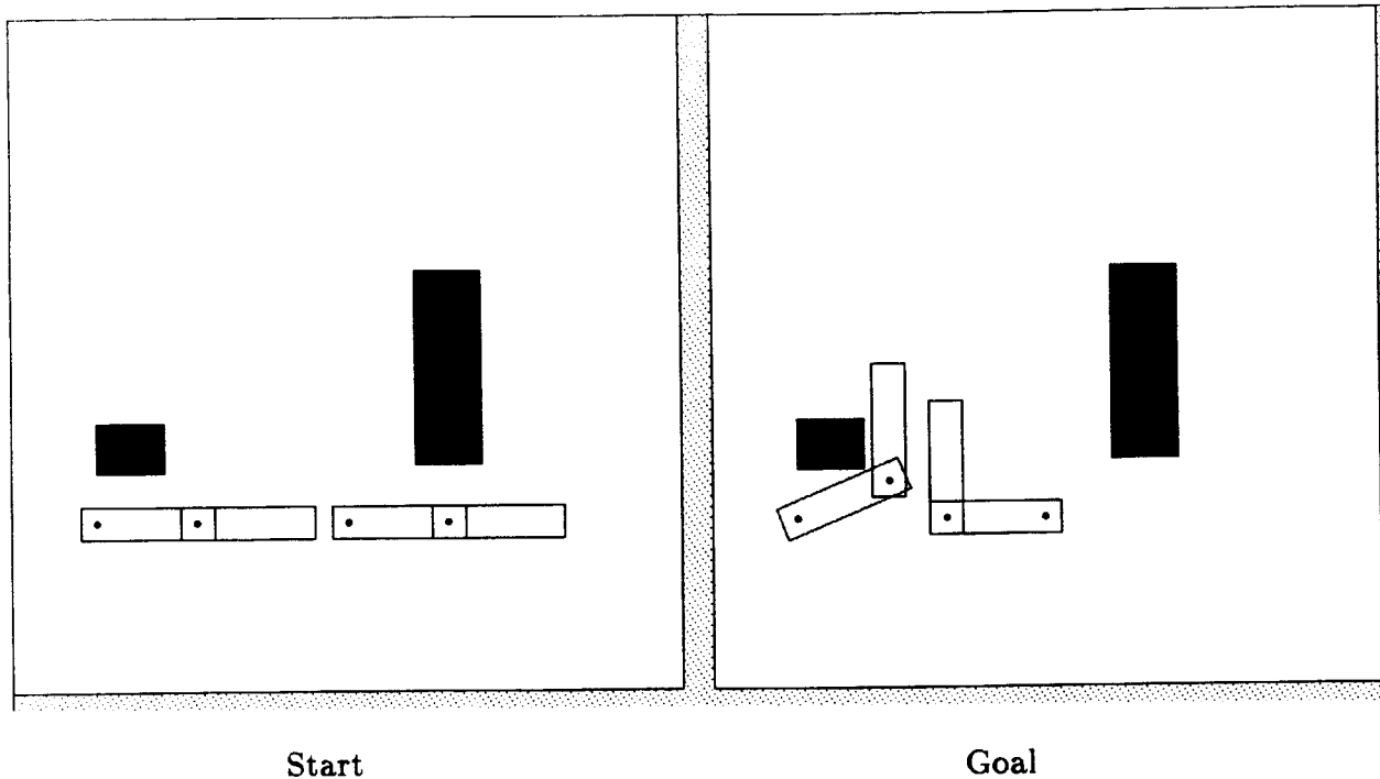
Figure 25. Start and goal configurations for two arms. The motion of the left arm is planned first. The motion of the right arm is planned given the motion of the first arm.
