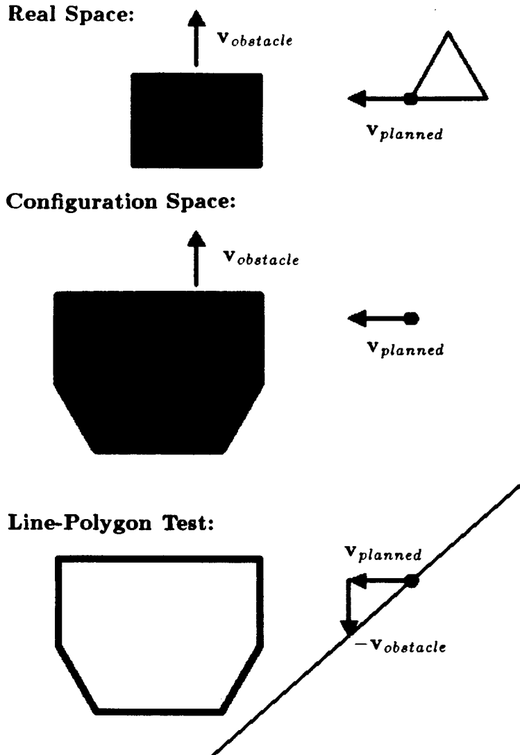
Figure 8. The problem of deciding whether two moving objects collide is first transformed into the problem of deciding whether a moving point collides with a moving configuration space obstacle. This problem is then transformed into a line-polygon intersection test.
