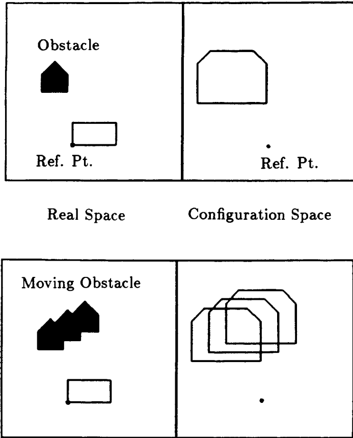
Figure 7. The top two frames show a rectangle and a stationary obstacle, along with the constraints in the rectangle's configuration space that are determined by the obstacle. The bottom two frames show how the translation of the real space obstacle is reflected in configuration space by a translation of the configuration space obstacle.
