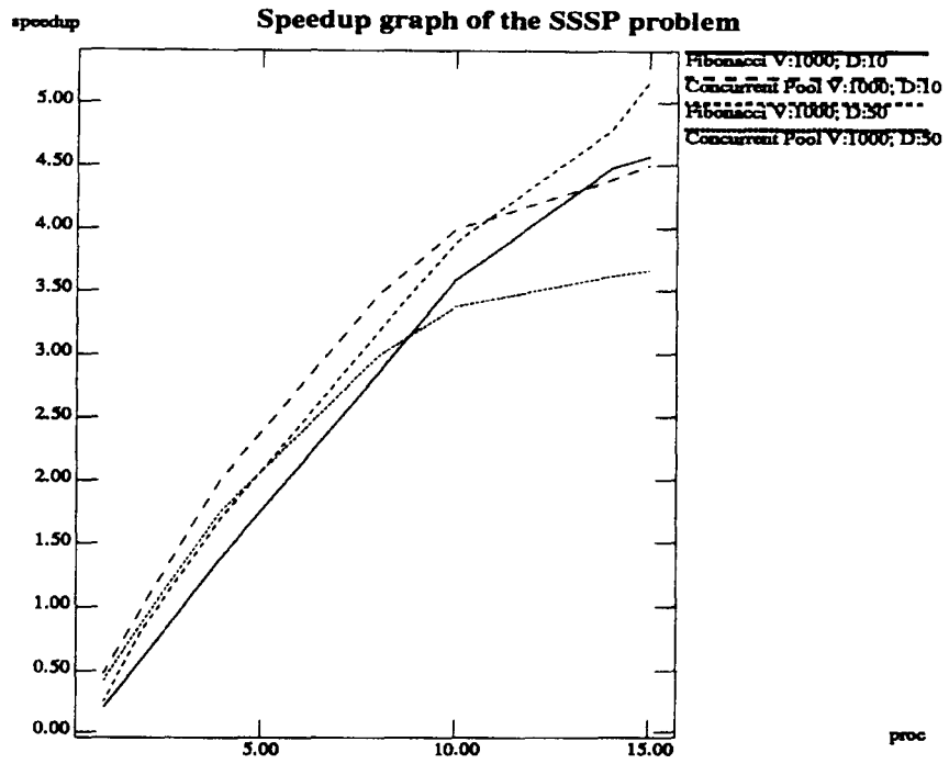
Figure 5.10: The speedup graph for the SSSP problem
