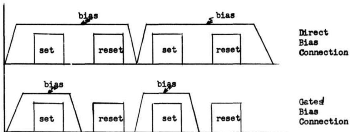
Timing Diagram for Switch Input Pulses
