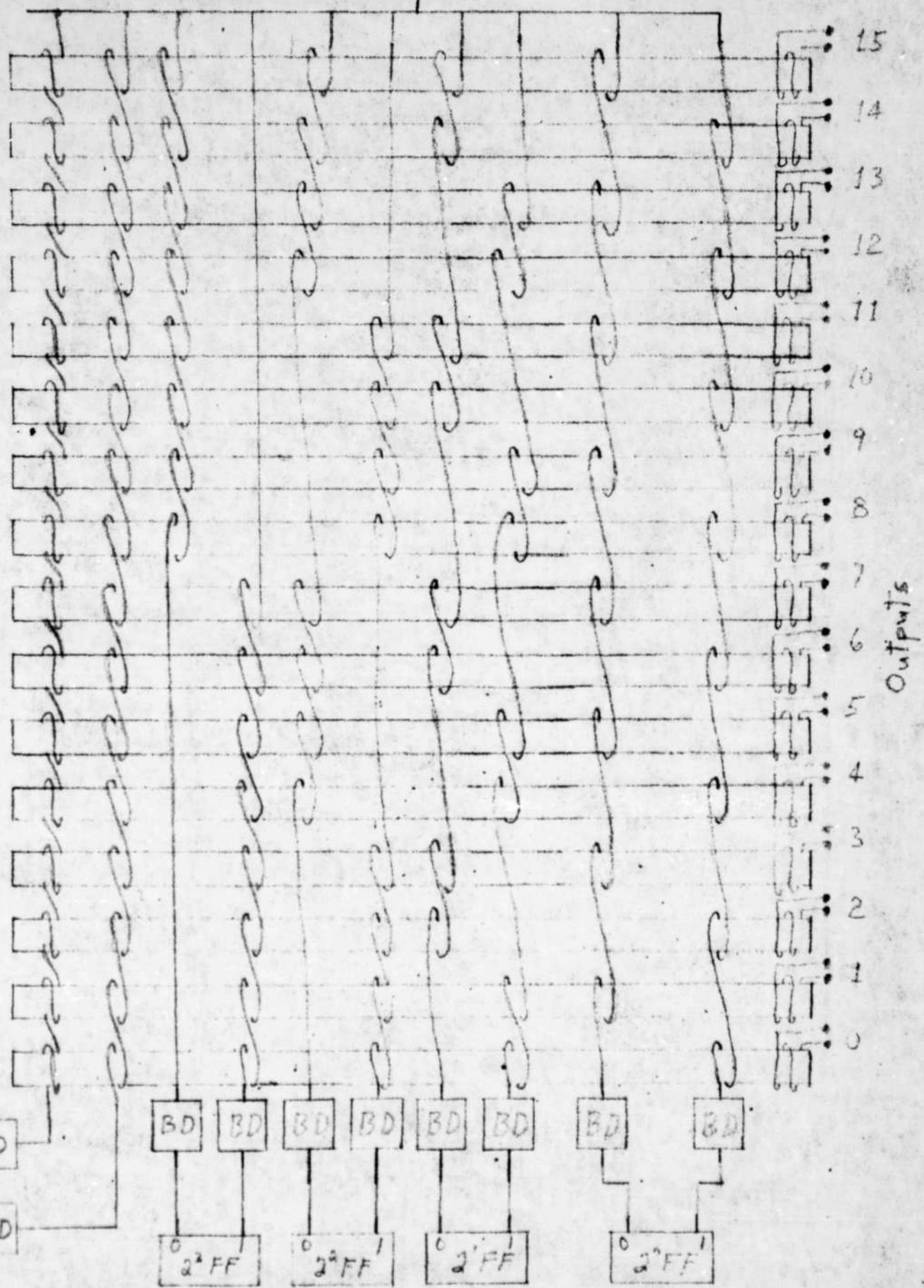
Magnetic Matrix Switch with One Set and One Reset Winding; Direct Bias Driver Connections Figure 1 Smith 5-21-53
