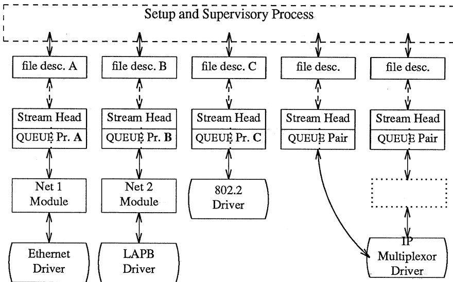
Figure 11-1. Internet Multiplexor Before Connecting
