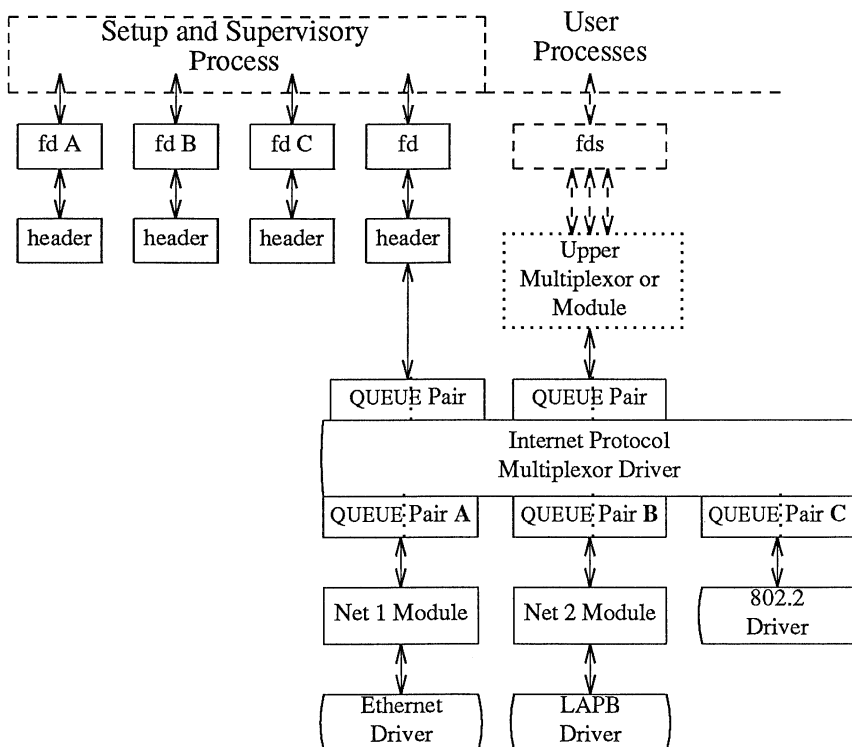
Figure 11-2. Internet Multiplexor After Connecting
