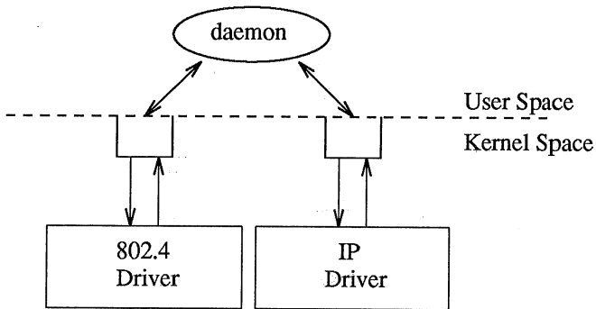
Figure 3-5. Before Link
