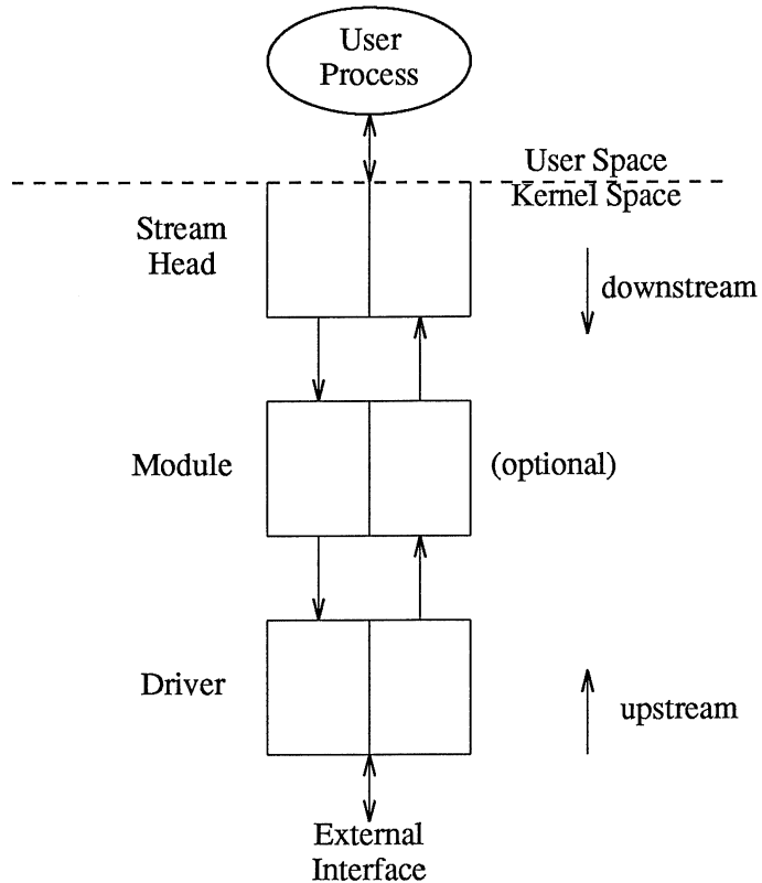
Figure 1. Basic Stream
