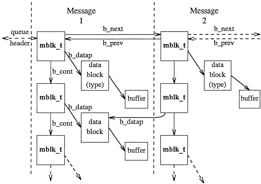
Figure 7-1. Message Form and Linkage
