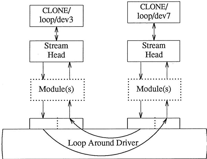
Figure 10-1. Loop Around Streams
