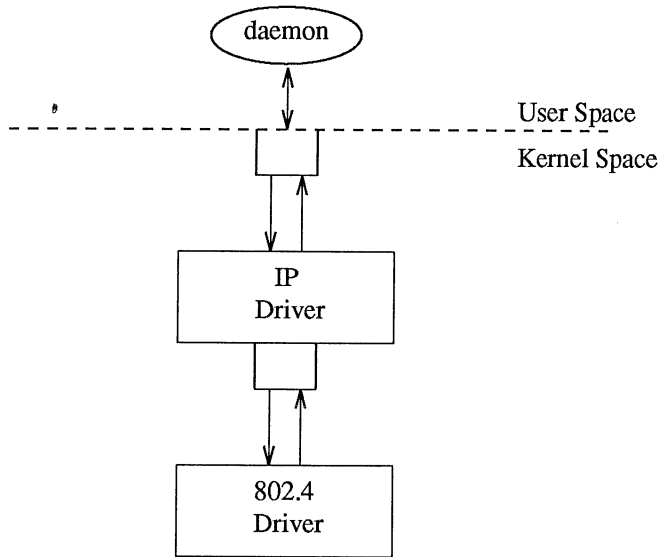
Figure 3-6. The complete Stream
