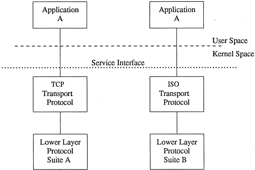
Figure 4-1. Protocol Substitution
