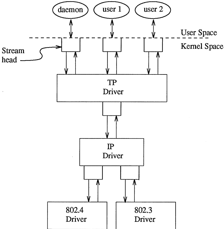
Figure 3-4. Protocol Multiplexor
