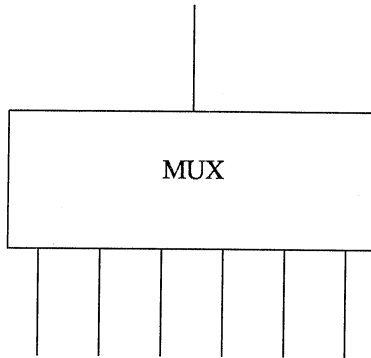
Figure 3-2. One-to-many Multiplexor
