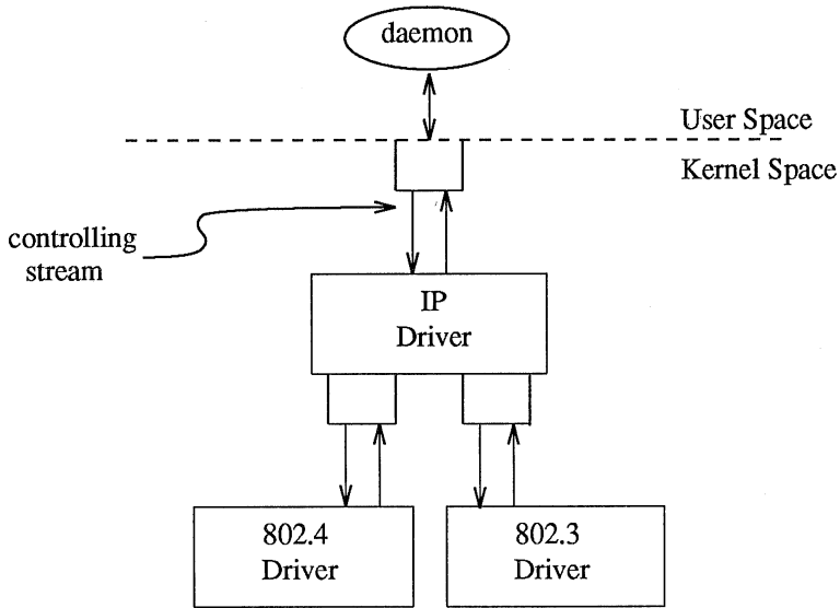
Figure 3-7. IP Multiplexor
