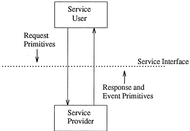
Figure 4-2. Service Interface
