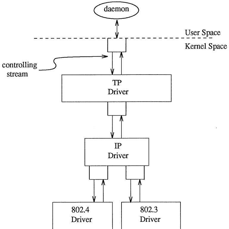
Figure 3-8. TP Multiplexor
