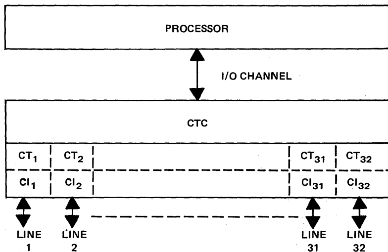
Figure 8-1. GCS Subsystem
