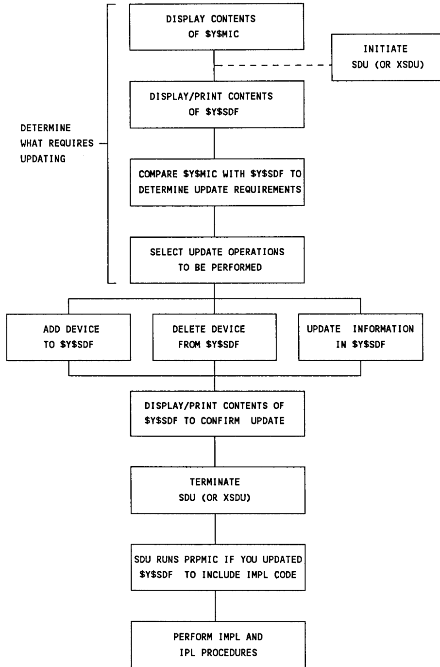
Figure 2-8. Updating $Y$SDF
