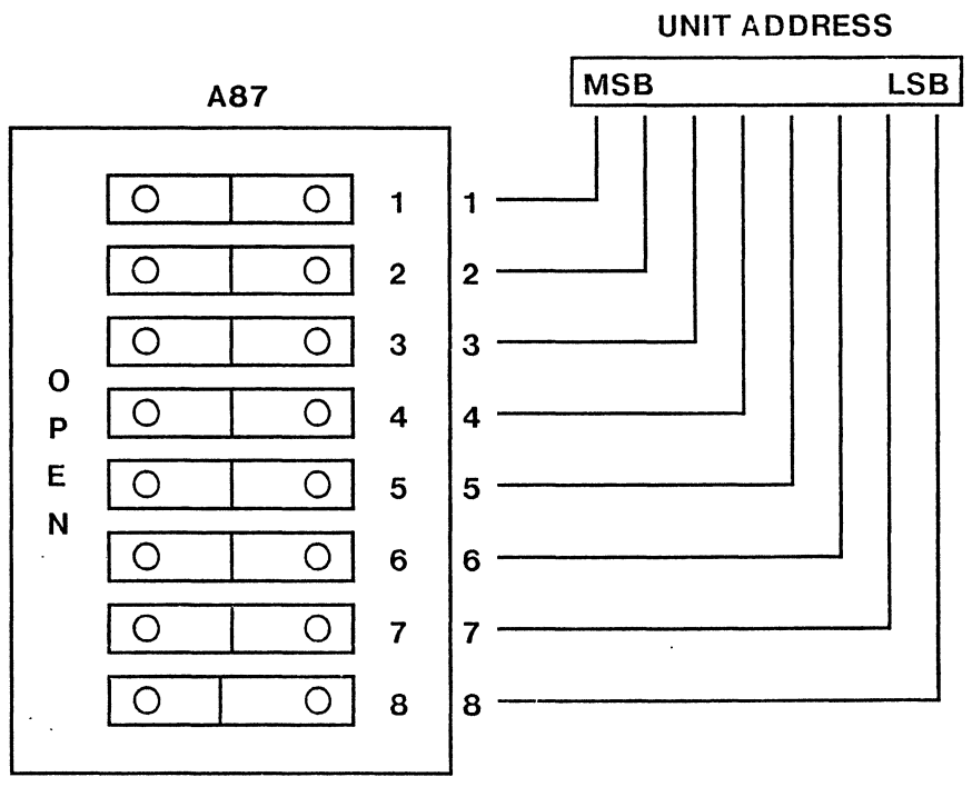
FIGURE 1. PDP11 ETHERNET NETWORK INTERFACE SWITCH SETTINGS Filed on: PDP11SW.sil
