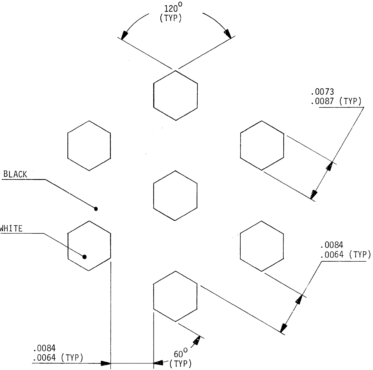
DETAIL A ENLARGED (SEE SHEET 3)
