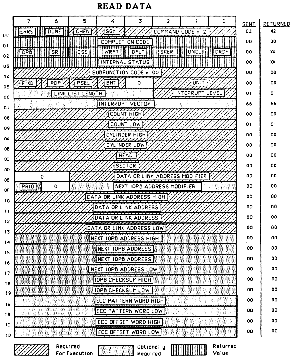
FIGURE 7-10. SAMPLE READ DATA IOPB
