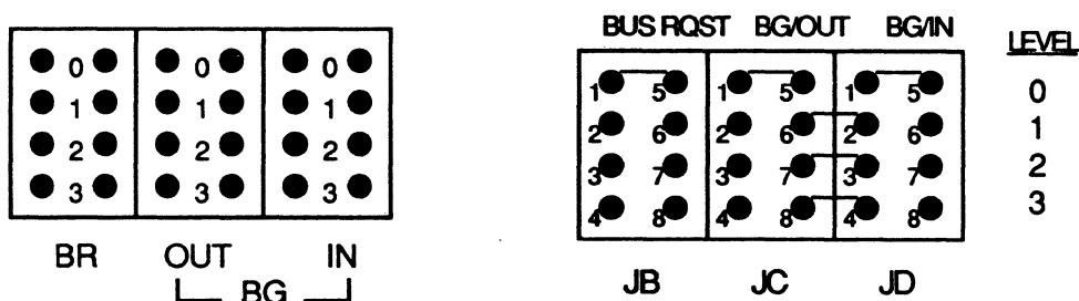
Figure 2-3A. Actual Board Layout
