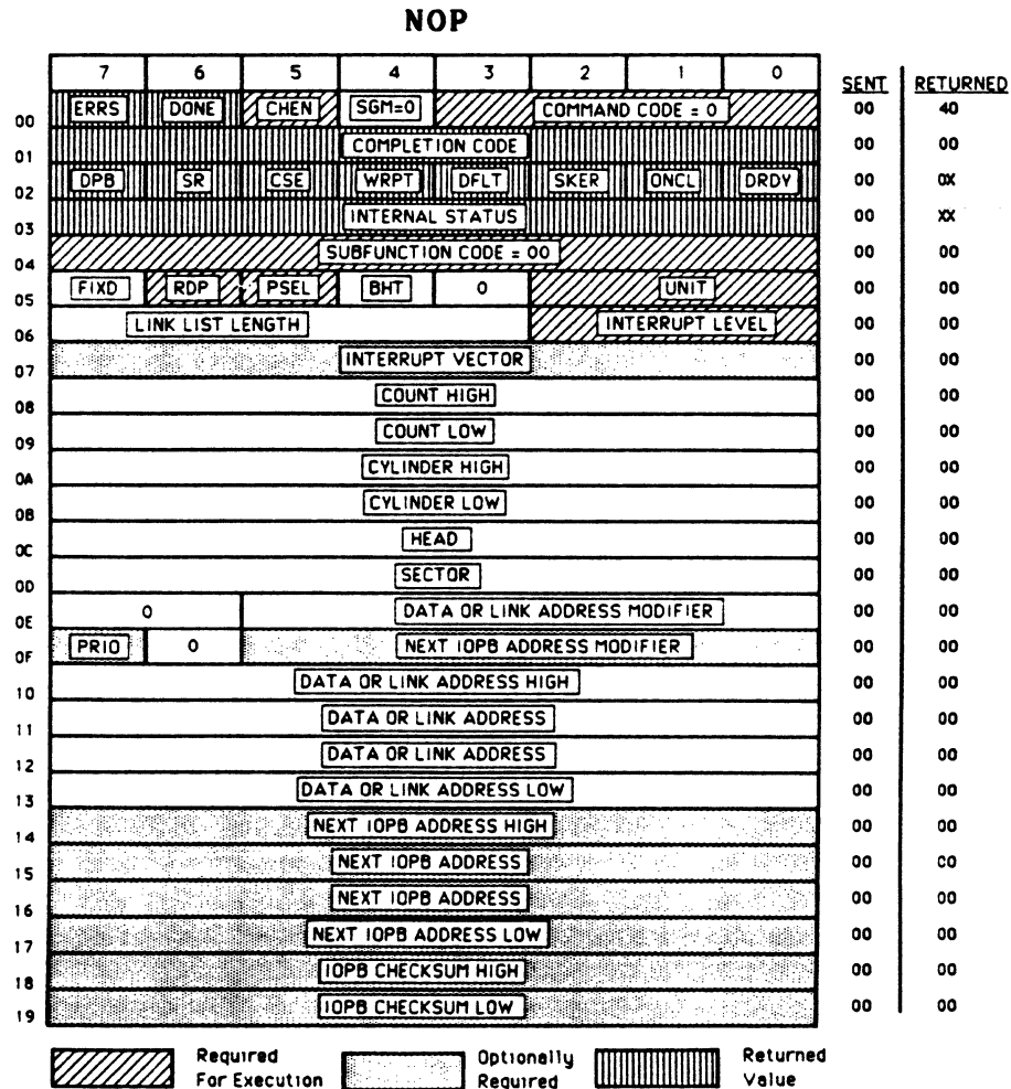
FIGURE 7-1. SAMPLE NOP IOPB
