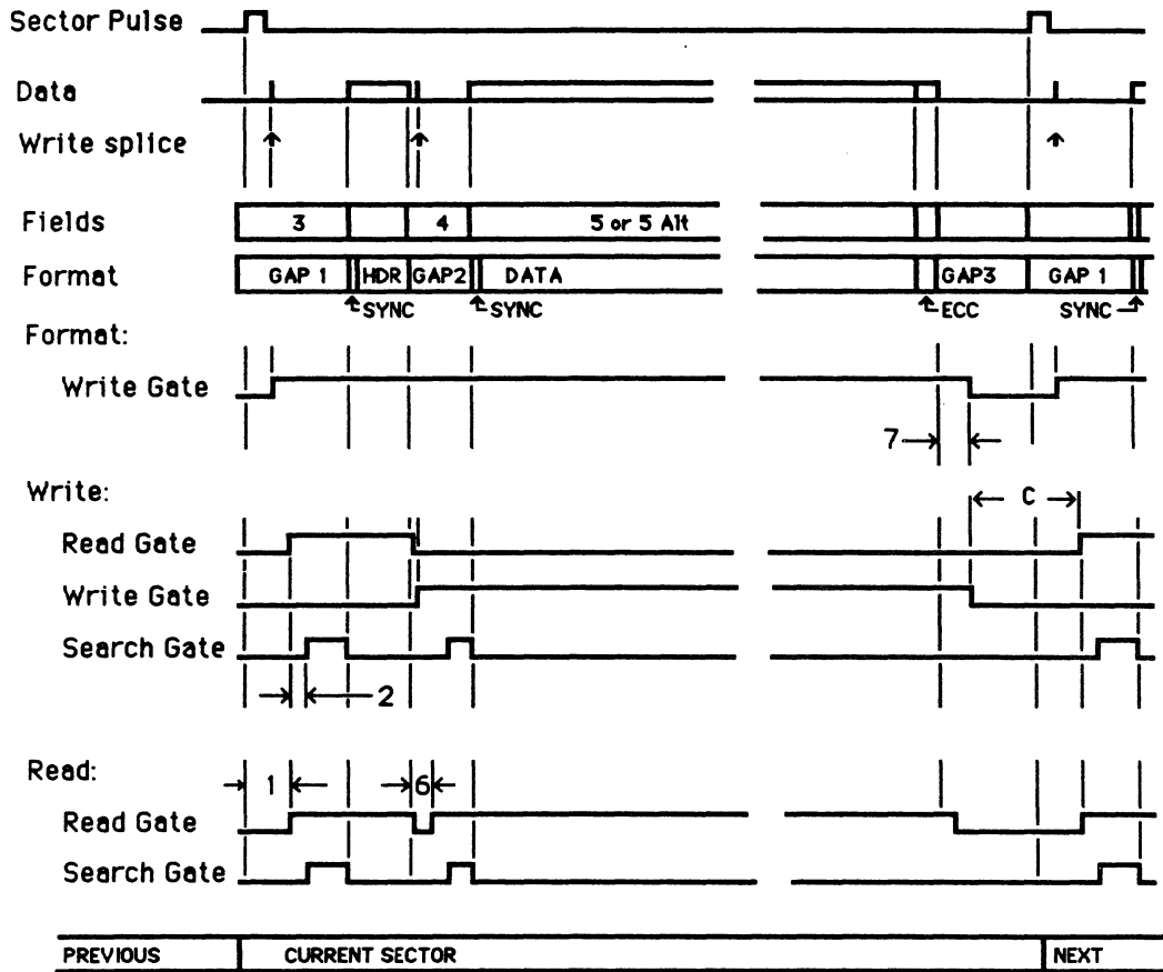
FIGURE 8-7. SECTOR GAP SIZES
