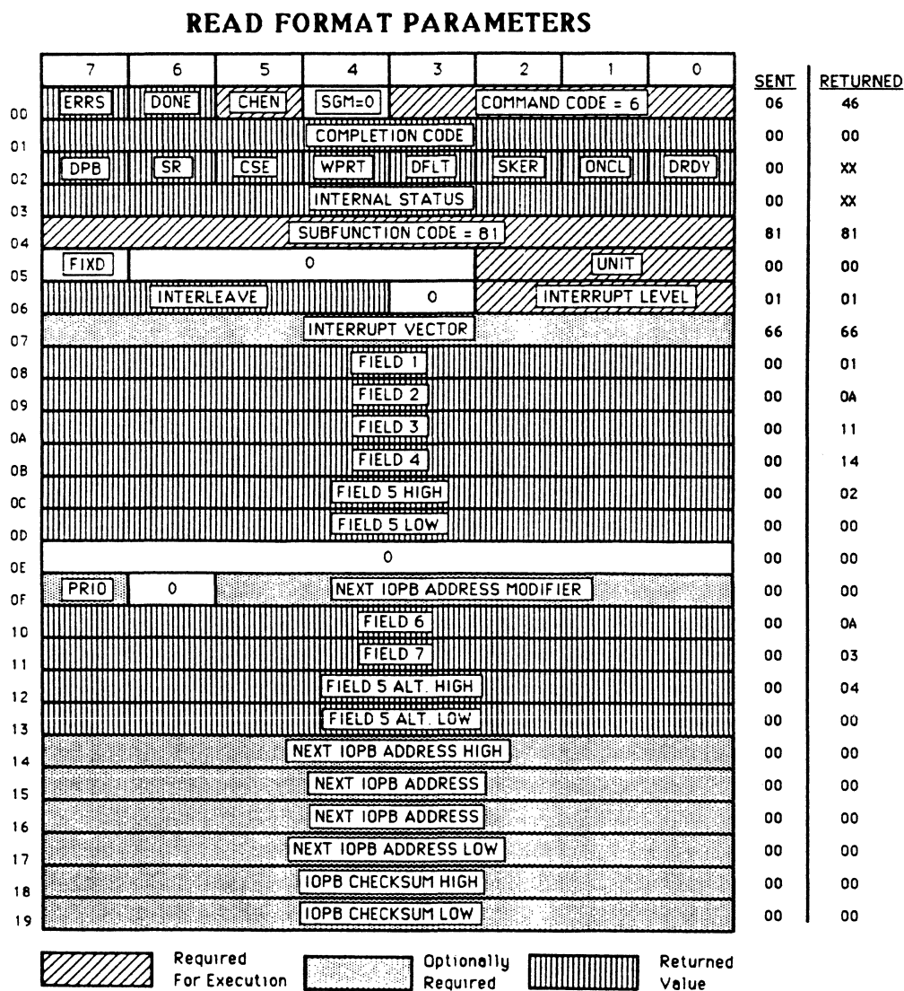
FIGURE 7-4. SAMPLE READ FORMAT PARAMETERS IOPB
