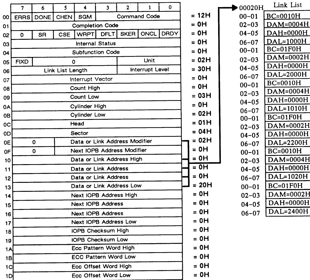
Figure 8-11. Scatter/Gather Transfers
