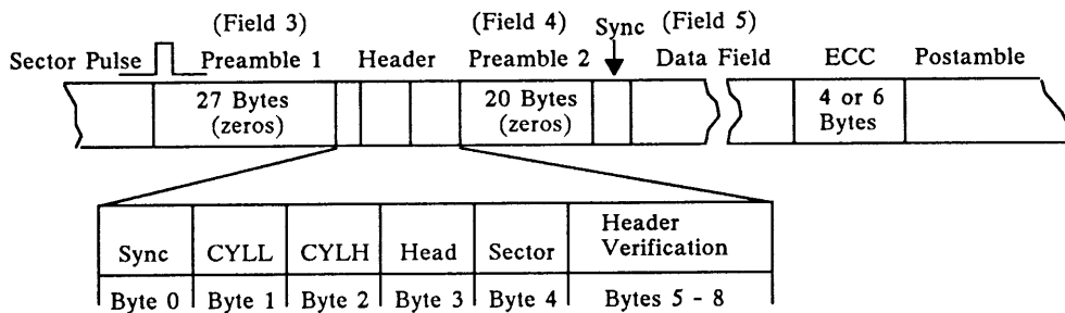
Figure 8-4. Standard Field Formats
