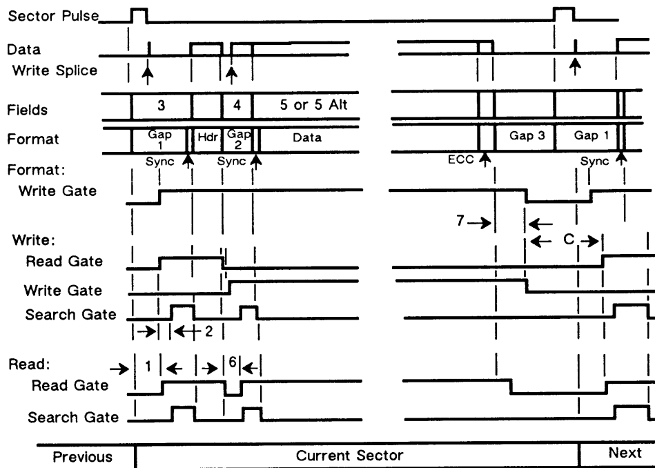
Figure 8-3. Sector Gap Sizes
