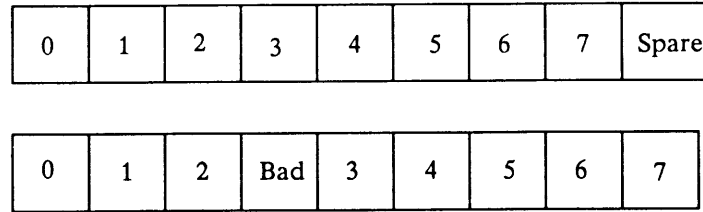
Figure 8-5. Sector Slip
