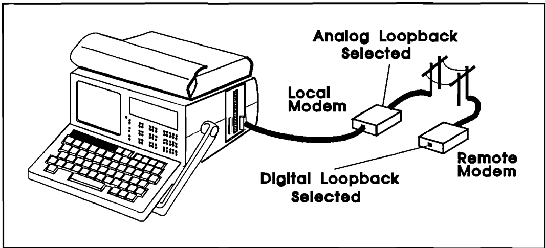
Figure 4-3. Connection for Loopback Testing
